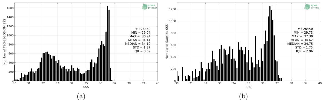
Figure 2: Histograms of SSS from TSG-LEGOS-DM (a) and Aquarius-L3-JPL-V5-7DAY-RUNNING (b) considering all match-up pairs per bins of 0.1 over the Gulf Stream Pi-MEP region and for the full satellite product period.
