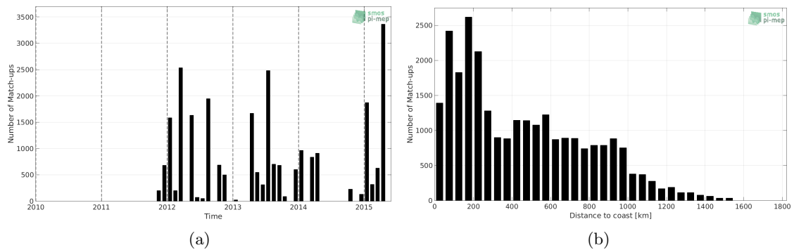
Figure 1: Number of match-ups between TSG-LEGOS-DM and Aquarius-L3-JPL-V5-7DAY-RUNNING SSS as a function of time (a) and as function of the distance to coast (b) over the Gulf Stream Pi-MEP region and for the full satellite product period.
