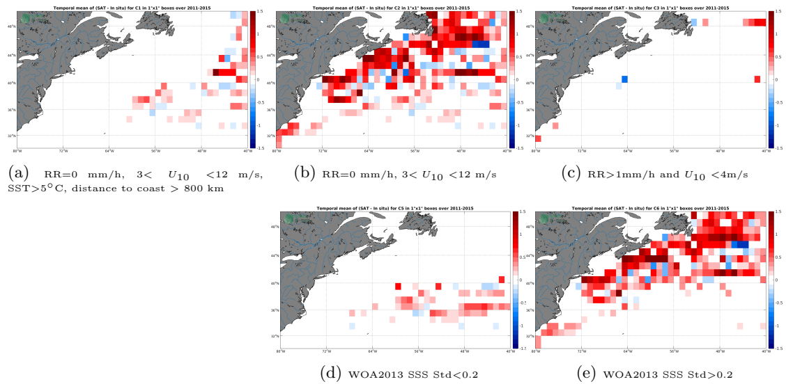
Figure 12: Temporal mean gridded over spatial boxes of size 1^\circ \times 1^\circ of \Delta SSS (Aquarius-L3-JPL-V5-7DAY-RUNNING - TSG-LEGOS-DM) for 5 different subdatasets corresponding to:RR=0 mm/h, 3 < U_{10} < 12 m/s, SST >5^\circ C, distance to coast > 800 km (a), RR=0 mm/h, 3 < U_{10} < 12 m/s (b), RR >1 mm/h and U_{10} < 4 m/s (c), WOA2013 SSS Std <0.2 (d), WOA2013 SSS Std >0.2 (e).
