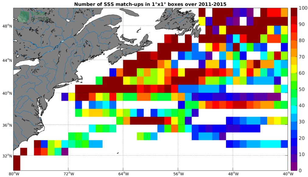
Figure 4: Number of SSS match-ups between TSG-LEGOS-DM SSS and the Aquarius-L3-JPL-V5-7DAY-RUNNING SSS product for the Gulf Stream Pi-MEP region over 1^\circ \times 1^\circ boxes and for the full satellite product period.
