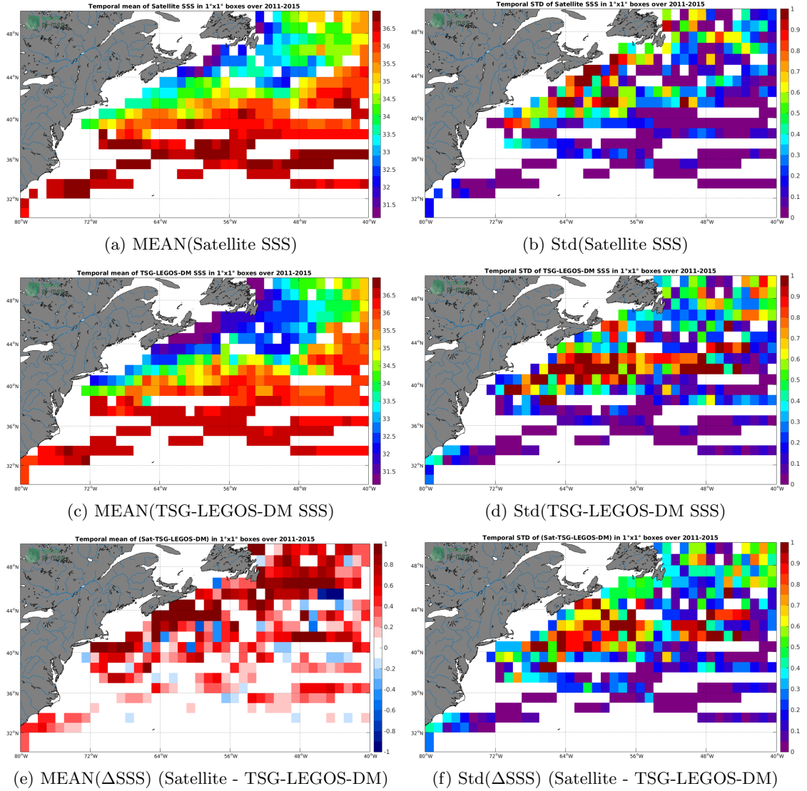
Figure 6: Temporal mean (left) and Std (right) of SSS from Aquarius-L3-JPL-V5-7DAY-RUNNING (top), TSG-LEGOS-DM (middle), and of \Delta\text{SSS} (Satellite - TSG-LEGOS-DM). Only match-up pairs are used to generate these maps.
