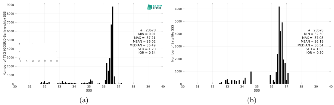
Figure 3: Histograms of SSS from TSG (GOSUD-Sailing-ship) (a) and Aquarius SSS L3 CAP v5 - 7-Day running (JPL) (b) considering all match-up pairs per bins of 0.1 over the Gulf Stream Pi-MEP region and for the full satellite product period.
