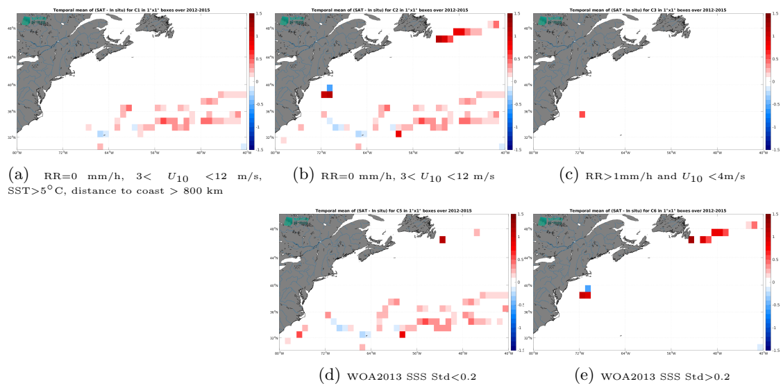
Figure 14: Temporal mean gridded over spatial boxes of size 1^\circ \times 1^\circ of \Delta SSS (Aquarius SSS L3 CAP v5 - 7-Day running (JPL) - TSG (GOSUD-Sailing-ship)) for 5 different subdatasets corresponding to:RR=0 mm/h, 3 < U_{10} < 12 m/s, SST >5^\circ\text{C} , distance to coast > 800 km (a), RR=0 mm/h, 3 < U_{10} < 12 m/s (b), RR >1 mm/h and U_{10} < 4 m/s (c), WOA2013 SSS Std <0.2 (d), WOA2013 SSS Std >0.2 (e).
