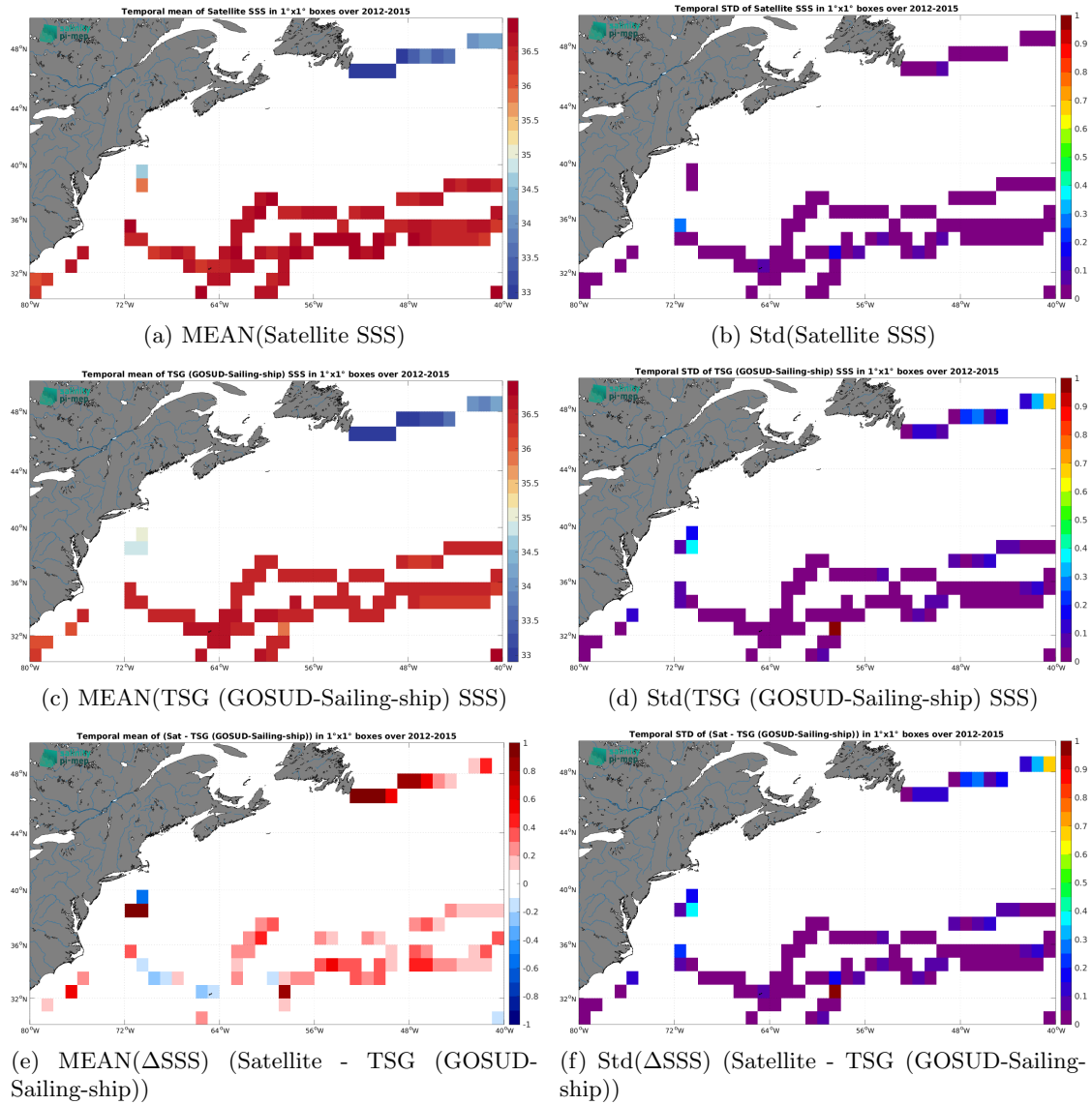
Figure 7: Temporal mean (left) and Std (right) of SSS from Aquarius SSS L3 CAP v5 - 7-Day running (JPL) (top), TSG (GOSUD-Sailing-ship) (middle), and of \Delta SSS (Satellite - TSG (GOSUD-Sailing-ship)). Only match-up pairs are used to generate these maps.
