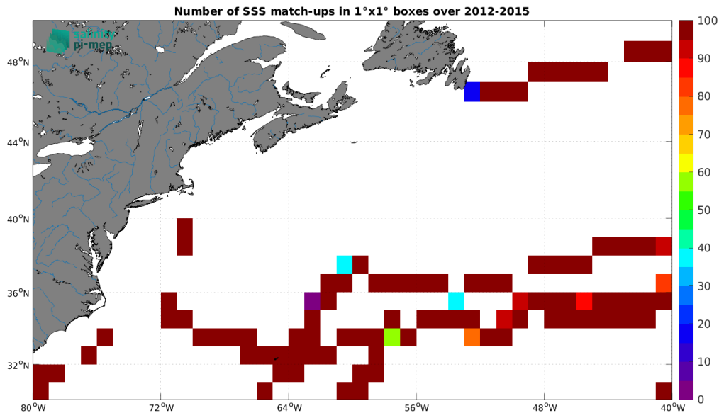
Figure 5: Number of SSS match-ups between TSG (GOSUD-Sailing-ship) SSS and the Aquarius SSS L3 CAP v5 - 7-Day running (JPL) SSS product for the Gulf Stream Pi-MEP region over 1^\circ \times 1^\circ boxes and for the full satellite product period.
