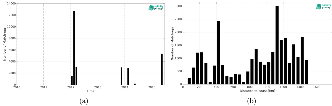
Figure 2: Number of match-ups between TSG (GOSUD-Sailing-ship) and Aquarius SSS L3 CAP v5 - 7-Day running (JPL) SSS as a function of time (a) and as function of the distance to coast (b) over the Gulf Stream Pi-MEP region and for the full satellite product period.
