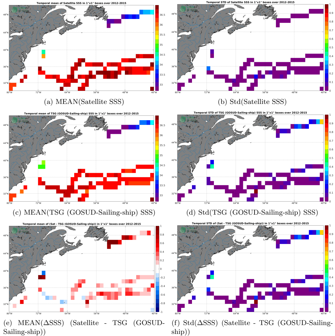
Figure 6: Temporal mean (left) and Std (right) of SSS from Aquarius SSS L3 CAP v5 - 7-Day running (JPL) (top), TSG (GOSUD-Sailing-ship) (middle), and of \Delta\text{SSS} (Satellite - TSG (GOSUD-Sailing-ship)). Only match-up pairs are used to generate these maps.
