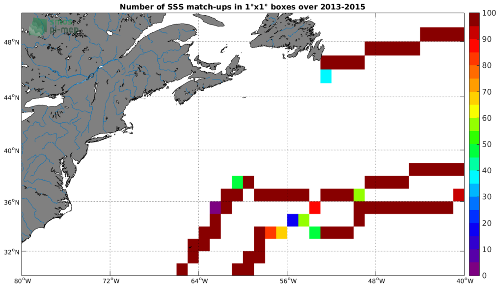
Figure 4: Number of SSS match-ups between TSG-GOSUD-Sailing-ship SSS and the Aquarius-L3-JPL-V5-7DAY-RUNNING SSS product for the Gulf Stream Pi-MEP region over 1°x1° boxes and for the full satellite product period.
