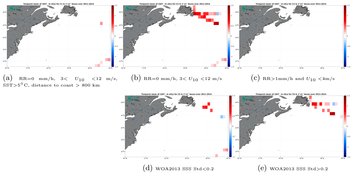
Figure 14: Temporal mean gridded over spatial boxes of size 1^\circ \times 1^\circ of \Delta SSS (Aquarius SSS L3 CAP v5 - 7-Day running (JPL) - TSG (GOSUD-Research-vessel)) for 5 different subdatasets corresponding to: RR=0 mm/h, 3 < U_{10} < 12 m/s, SST > 5°C, distance to coast > 800 km (a), RR=0 mm/h, 3 < U_{10} < 12 m/s (b), RR > 1mm/h and U_{10} < 4 m/s (c), WOA2013 SSS Std < 0.2 (d), WOA2013 SSS Std > 0.2 (e).
