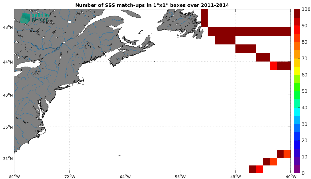
Figure 5: Number of SSS match-ups between TSG (GOSUD-Research-vessel) SSS and the Aquarius SSS L3 CAP v5 - 7-Day running (JPL) SSS product for the Gulf Stream Pi-MEP region over 1^\circ \times 1^\circ boxes and for the full satellite product period.
