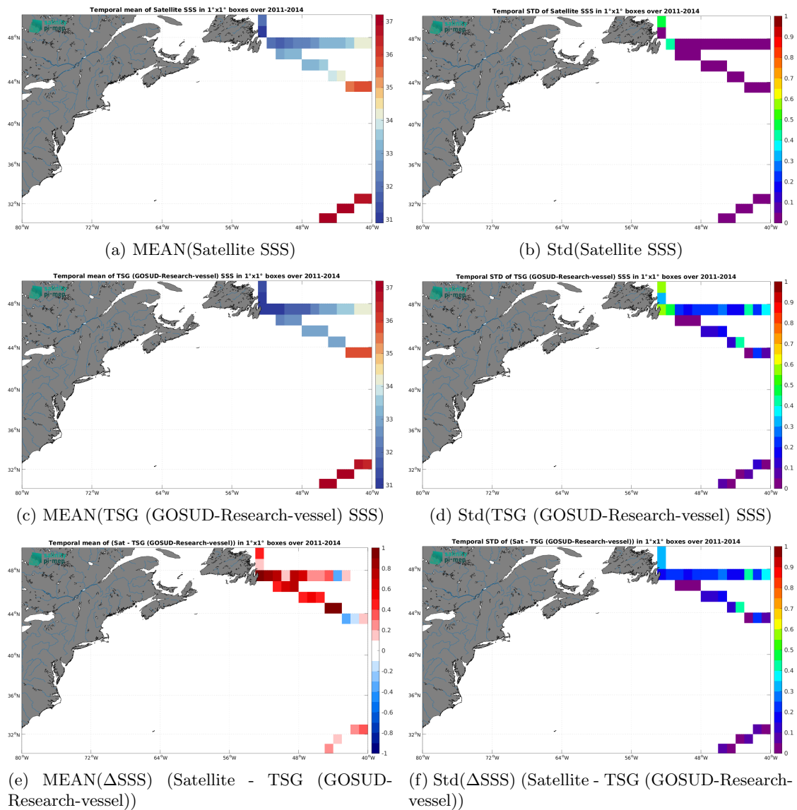
Figure 7: Temporal mean (left) and Std (right) of SSS from Aquarius SSS L3 CAP v5 - 7-Day running (JPL) (top), TSG (GOSUD-Research-vessel) (middle), and of \Delta SSS (Satellite - TSG (GOSUD-Research-vessel)). Only match-up pairs are used to generate these maps.
