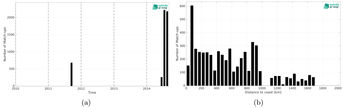
Figure 2: Number of match-ups between TSG (GOSUD-Research-vessel) and Aquarius SSS L3 CAP v5 - 7-Day running (JPL) SSS as a function of time (a) and as function of the distance to coast (b) over the Gulf Stream Pi-MEP region and for the full satellite product period.
