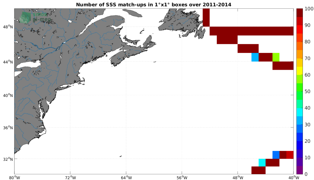
Figure 4: Number of SSS match-ups between TSG (GOSUD-Research-vessel) SSS and the Aquarius SSS L3 CAP v5 - 7-Day running (JPL) SSS product for the Gulf Stream Pi-MEP region over 1^\circ \times 1^\circ boxes and for the full satellite product period.
