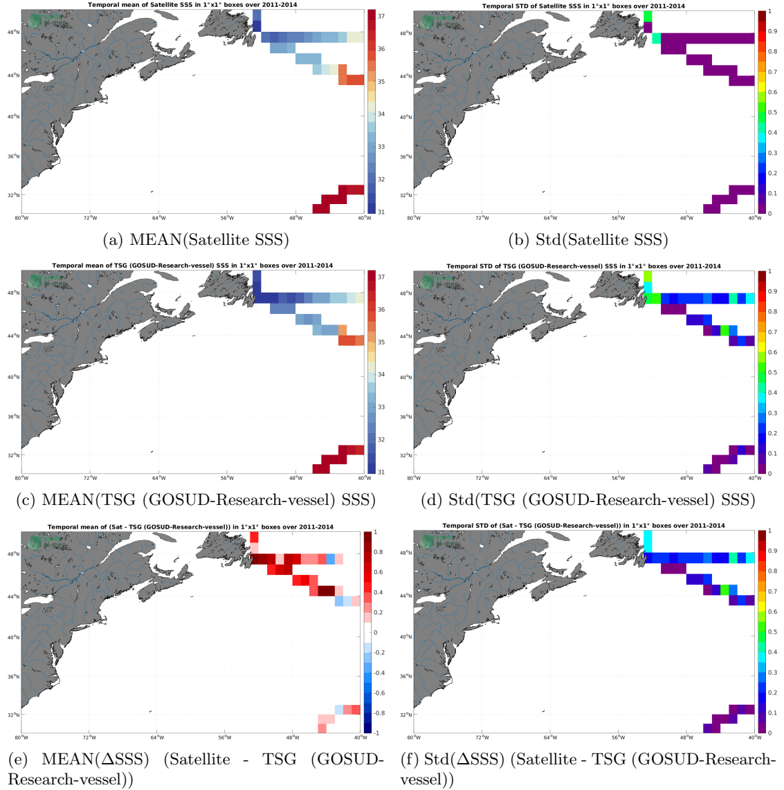
Figure 6: Temporal mean (left) and Std (right) of SSS from Aquarius SSS L3 CAP v5 - 7-Day running (JPL) (top), TSG (GOSUD-Research-vessel) (middle), and of \Delta SSS (Satellite - TSG (GOSUD-Research-vessel)). Only match-up pairs are used to generate these maps.
