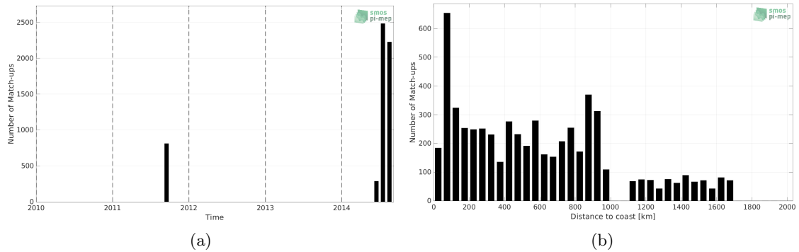
Figure 1: Number of match-ups between TSG (GOSUD-Research-vessel) and Aquarius SSS L3 CAP v5 - 7-Day running (JPL) SSS as a function of time (a) and as function of the distance to coast (b) over the Gulf Stream Pi-MEP region and for the full satellite product period.
