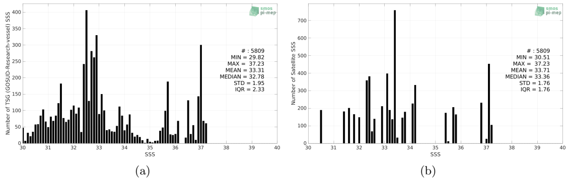
Figure 2: Histograms of SSS from TSG (GOSUD-Research-vessel) (a) and Aquarius SSS L3 CAP v5 - 7-Day running (JPL) (b) considering all match-up pairs per bins of 0.1 over the Gulf Stream Pi-MEP region and for the full satellite product period.
