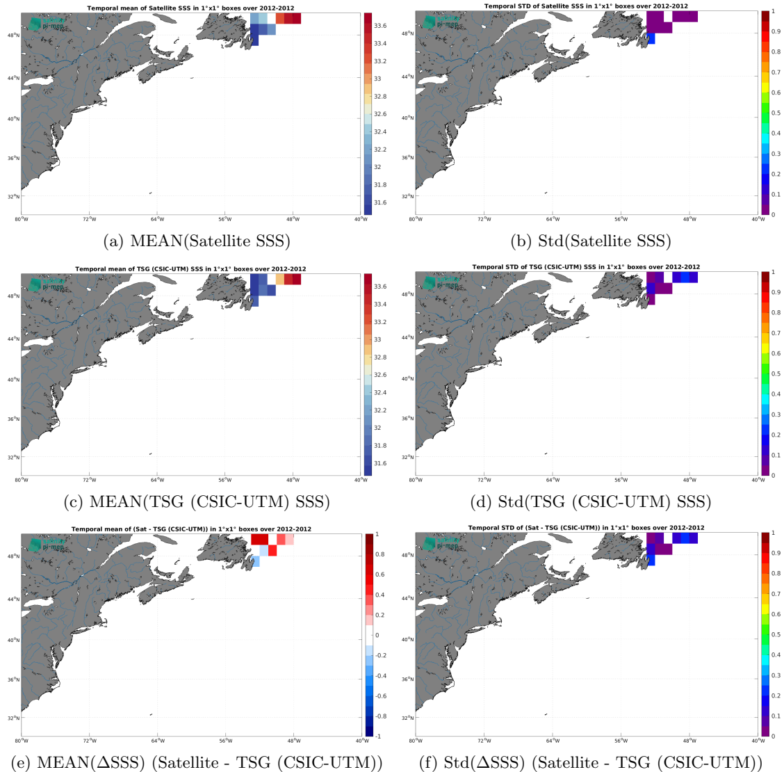
Figure 7: Temporal mean (left) and Std (right) of SSS from Aquarius SSS L3 CAP v5 - 7-Day running (JPL) (top), TSG (CSIC-UTM) (middle), and of \Delta SSS (Satellite - TSG (CSIC-UTM)). Only match-up pairs are used to generate these maps.
