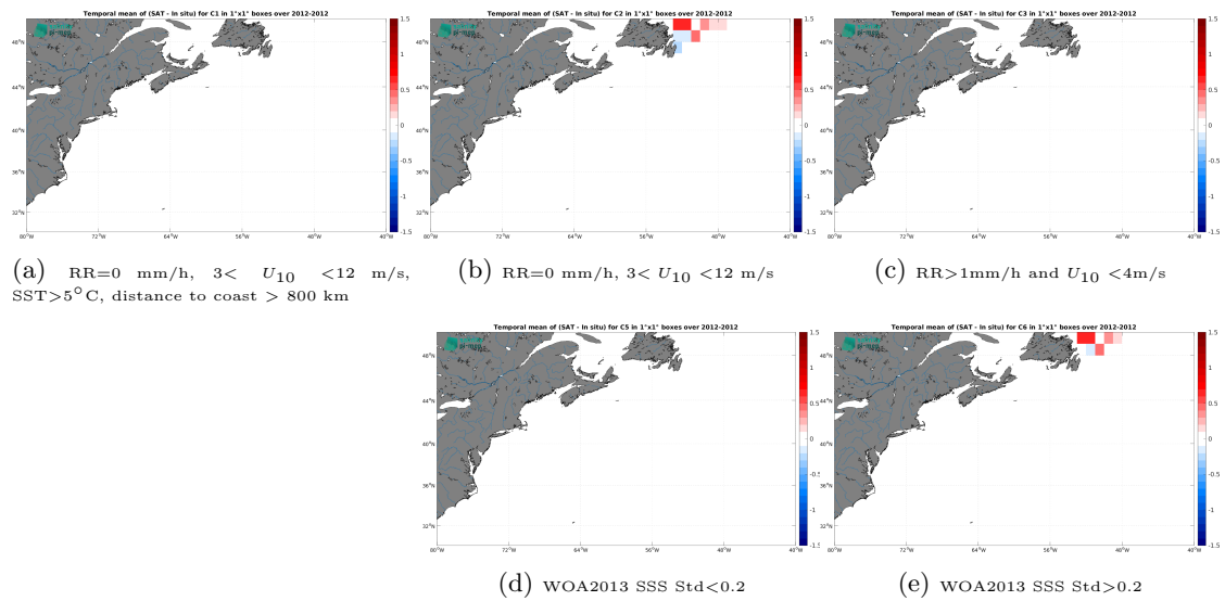
Figure 14: Temporal mean gridded over spatial boxes of size 1^\circ \times 1^\circ of \Delta SSS (Aquarius SSS L3 CAP v5 - 7-Day running (JPL) - TSG (CSIC-UTM)) for 5 different subdatasets corresponding to: RR=0 mm/h, 3 < U_{10} < 12 m/s, SST > 5°C, distance to coast > 800 km (a), RR=0 mm/h, 3 < U_{10} < 12 m/s (b), RR > 1mm/h and U_{10} < 4 m/s (c), WOA2013 SSS Std < 0.2 (d), WOA2013 SSS Std > 0.2 (e).
