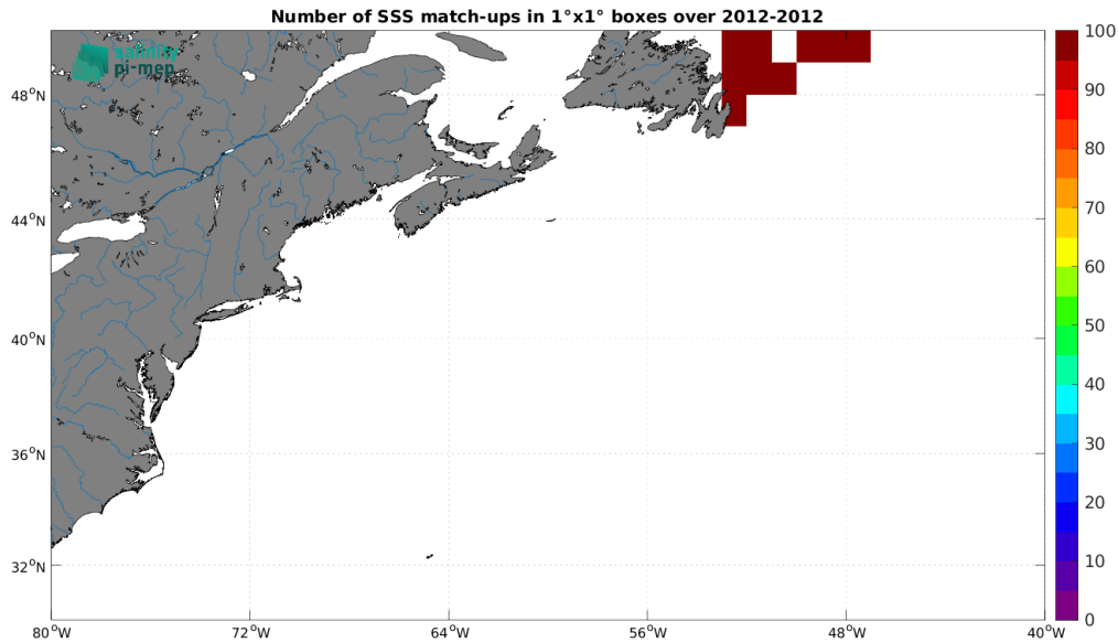
Figure 5: Number of SSS match-ups between TSG (CSIC-UTM) SSS and the Aquarius SSS L3 CAP v5 - 7-Day running (JPL) SSS product for the Gulf Stream Pi-MEP region over 1^\circ \times 1^\circ boxes and for the full satellite product period.
