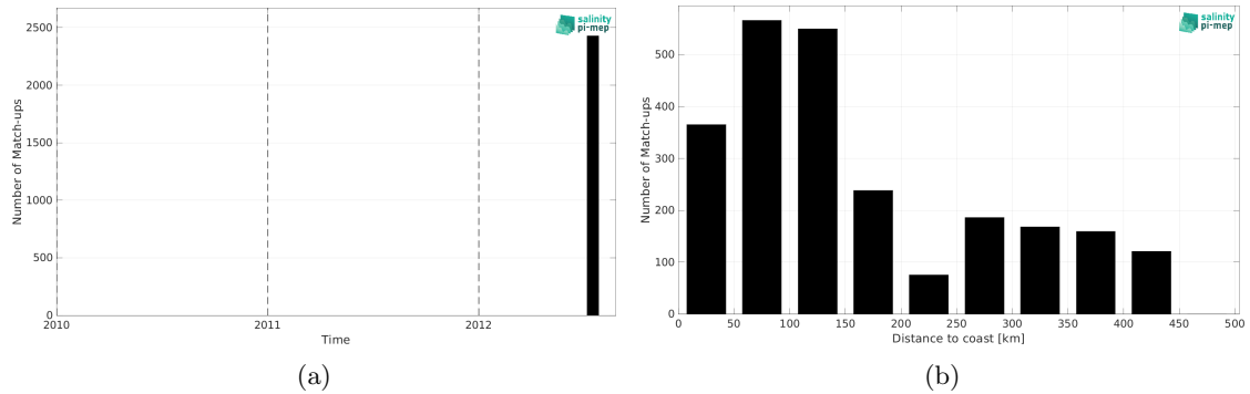
Figure 2: Number of match-ups between TSG (CSIC-UTM) and Aquarius SSS L3 CAP v5 - 7-Day running (JPL) SSS as a function of time (a) and as function of the distance to coast (b) over the Gulf Stream Pi-MEP region and for the full satellite product period.
