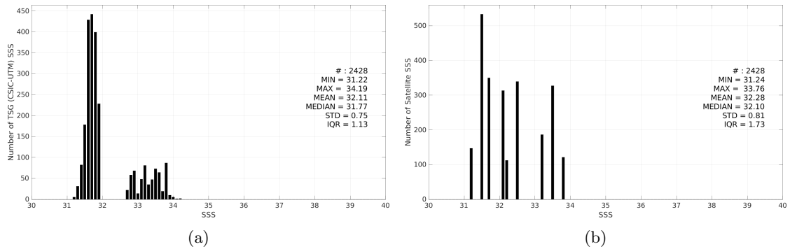
Figure 3: Histograms of SSS from TSG (CSIC-UTM) (a) and Aquarius SSS L3 CAP v5 - 7-Day running (JPL) (b) considering all match-up pairs per bins of 0.1 over the Gulf Stream Pi-MEP region and for the full satellite product period.
