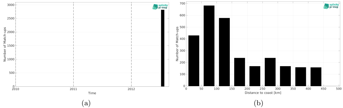
Figure 1: Number of match-ups between TSG (CSIC-UTM) and Aquarius SSS L3 CAP v5 - 7-Day running (JPL) SSS as a function of time (a) and as function of the distance to coast (b) over the Gulf Stream Pi-MEP region and for the full satellite product period.
