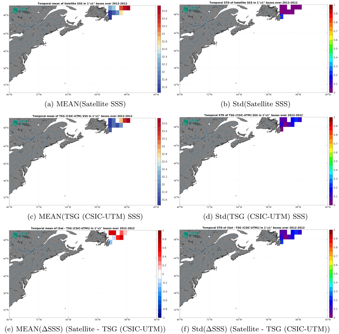
Figure 6: Temporal mean (left) and Std (right) of SSS from Aquarius SSS L3 CAP v5 - 7-Day running (JPL) (top), TSG (CSIC-UTM) (middle), and of \Delta SSS (Satellite - TSG (CSIC-UTM)). Only match-up pairs are used to generate these maps.
