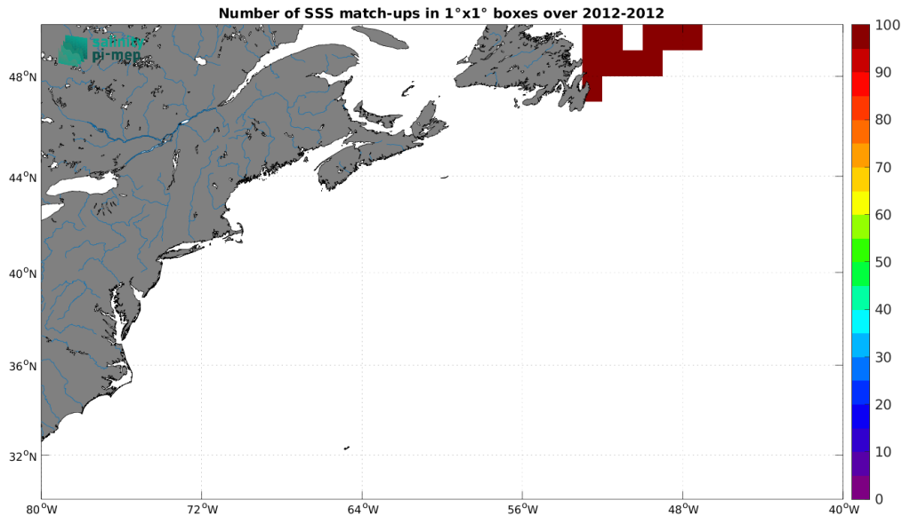
Figure 4: Number of SSS match-ups between TSG (CSIC-UTM) SSS and the Aquarius SSS L3 CAP v5 - 7-Day running (JPL) SSS product for the Gulf Stream Pi-MEP region over 1^\circ \times 1^\circ boxes and for the full satellite product period.
