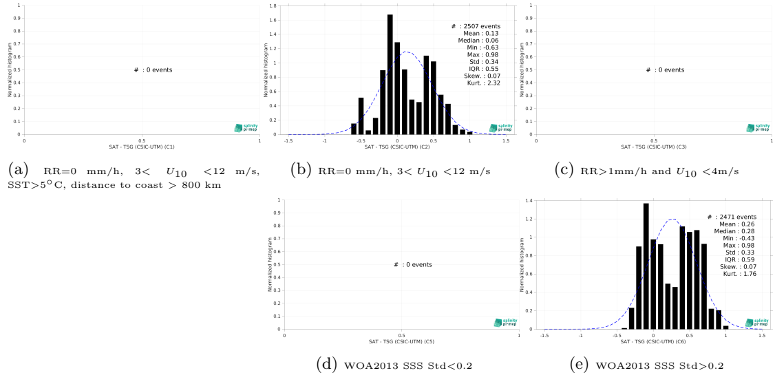
Figure 13: Normalized histogram of \Delta SSS (Aquarius SSS L3 CAP v5 - 7-Day running (JPL) - TSG (CSIC-UTM)) for 5 different subdatasets corresponding to: RR=0 mm/h, 3 < U_{10} < 12 m/s, SST > 5°C, distance to coast > 800 km (a), RR=0 mm/h, 3 < U_{10} < 12 m/s (b), RR > 1mm/h and U_{10} < 4 m/s (c), WOA2013 SSS Std < 0.2 (d), WOA2013 SSS Std > 0.2 (e).
