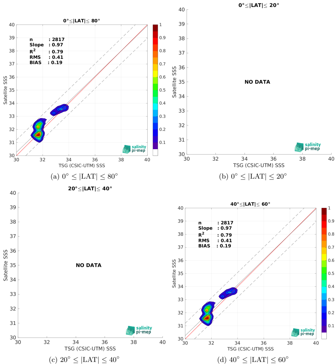
Figure 9: Contour maps of the concentration of Aquarius SSS L3 CAP v5 - 7-Day running (JPL) SSS (y-axis) versus TSG (CSIC-UTM) SSS (x-axis) at match-up pairs for different latitude bands. For each plot, the red line shows x=y . The black thin and dashed lines indicate a linear fit through the data cloud and the \pm 95\% confidence levels, respectively. The number match-up pairs n , the slope and R^2 coefficient of the linear fit, the root mean square (RMS) and the mean bias between satellite and in situ data are indicated for each latitude band in each plots.
