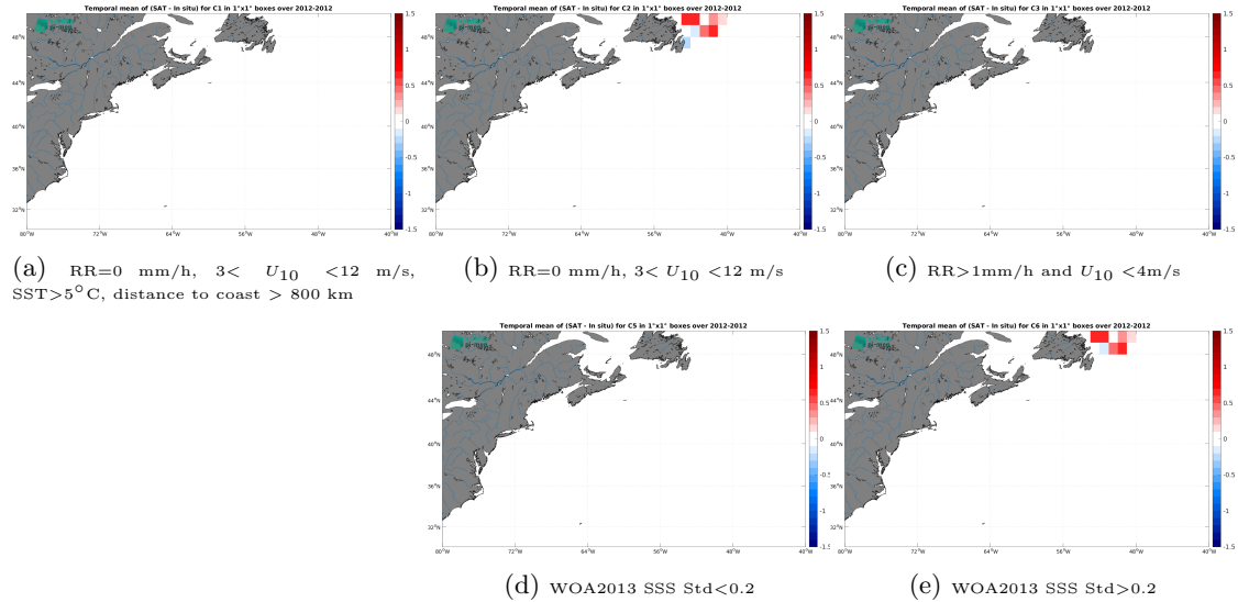
Figure 12: Temporal mean gridded over spatial boxes of size 1^{\circ}\times 1^{\circ} of \Delta\text{SSS} (Aquarius SSS L3 CAP v5 - 7-Day running (JPL) - TSG (CSIC-UTM)) for 5 different subdatasets corresponding to:RR=0 mm/h, 3 < U_{10} < 12 m/s, SST >5^{\circ}\text{C} , distance to coast > 800 km (a), RR=0 mm/h, 3 < U_{10} < 12 m/s (b), RR >1 mm/h and U_{10} < 4 m/s (c), WOA2013 SSS Std <0.2 (d), WOA2013 SSS Std >0.2 (e).
