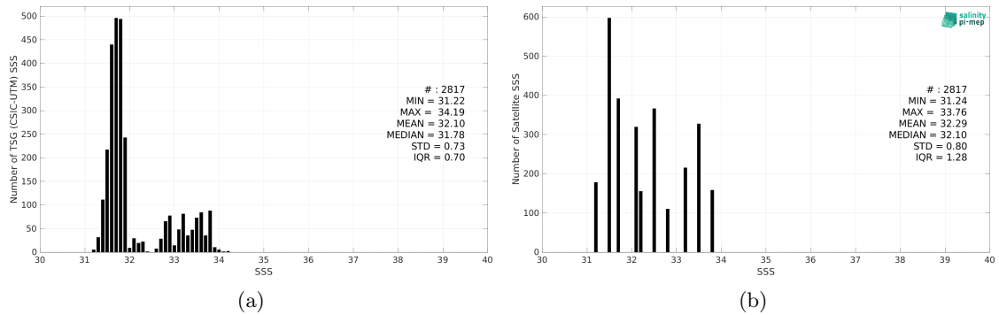
Figure 2: Histograms of SSS from TSG (CSIC-UTM) (a) and Aquarius SSS L3 CAP v5 - 7-Day running (JPL) (b) considering all match-up pairs per bins of 0.1 over the Gulf Stream Pi-MEP region and for the full satellite product period.
