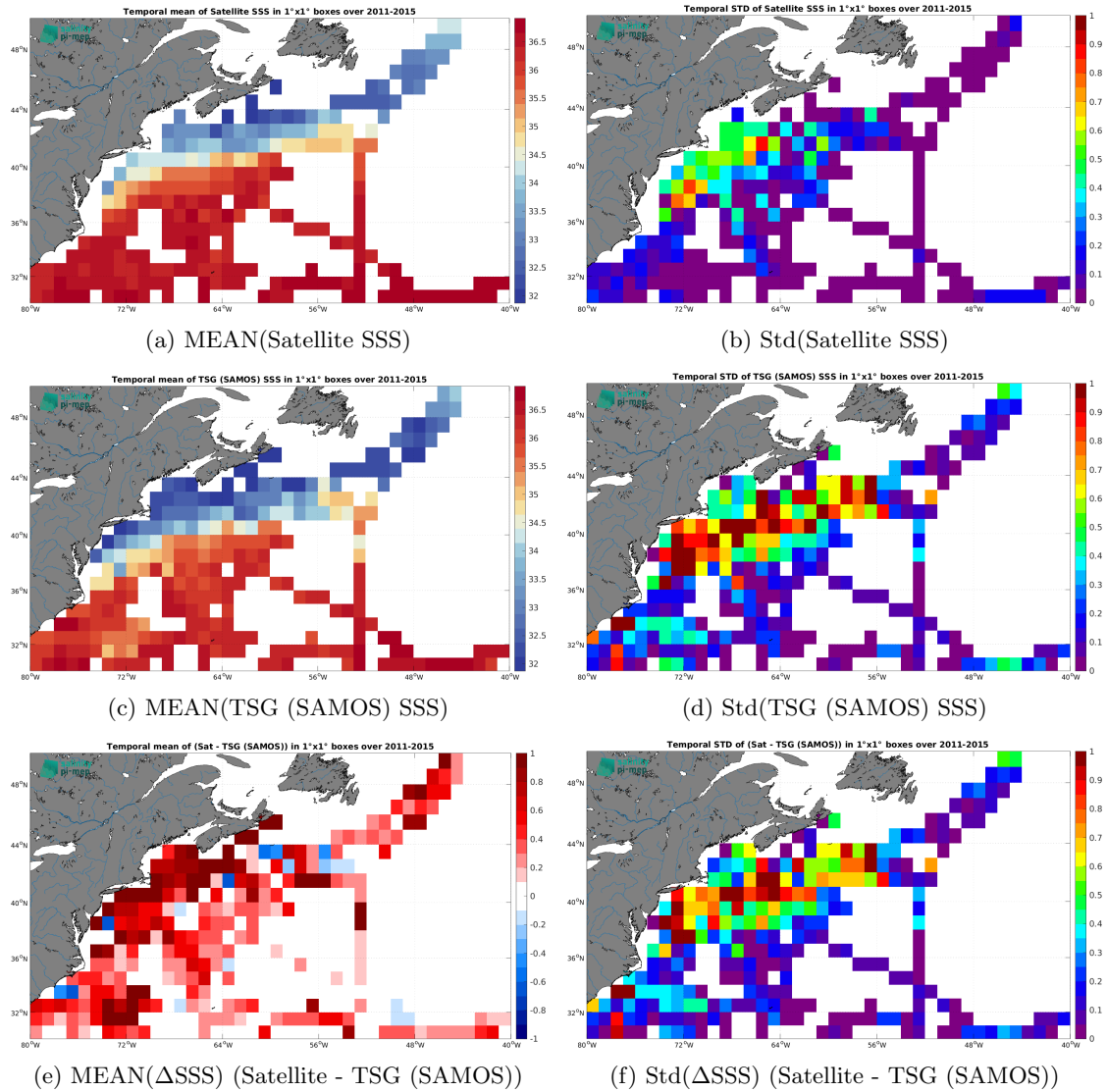
Figure 7: Temporal mean (left) and Std (right) of SSS from Aquarius SSS L3 CAP v5 - Monthly (JPL) (top), TSG (SAMOS) (middle), and of \Delta SSS (Satellite - TSG (SAMOS)). Only match-up pairs are used to generate these maps.
