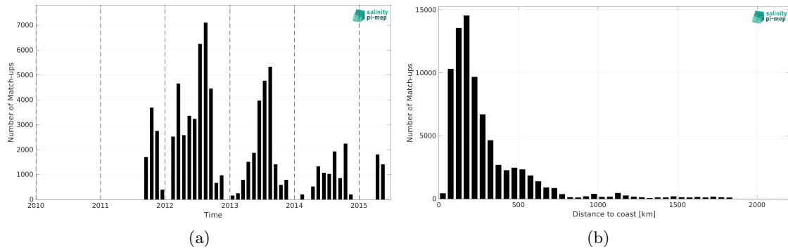
Figure 2: Number of match-ups between TSG (SAMOS) and Aquarius SSS L3 CAP v5 - Monthly (JPL) SSS as a function of time (a) and as function of the distance to coast (b) over the Gulf Stream Pi-MEP region and for the full satellite product period.
