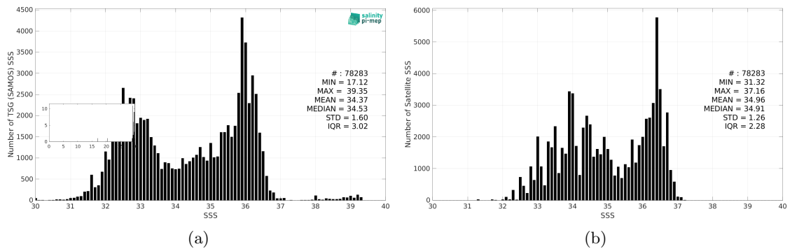
Figure 3: Histograms of SSS from TSG (SAMOS) (a) and Aquarius SSS L3 CAP v5 - Monthly (JPL) (b) considering all match-up pairs per bins of 0.1 over the Gulf Stream Pi-MEP region and for the full satellite product period.
