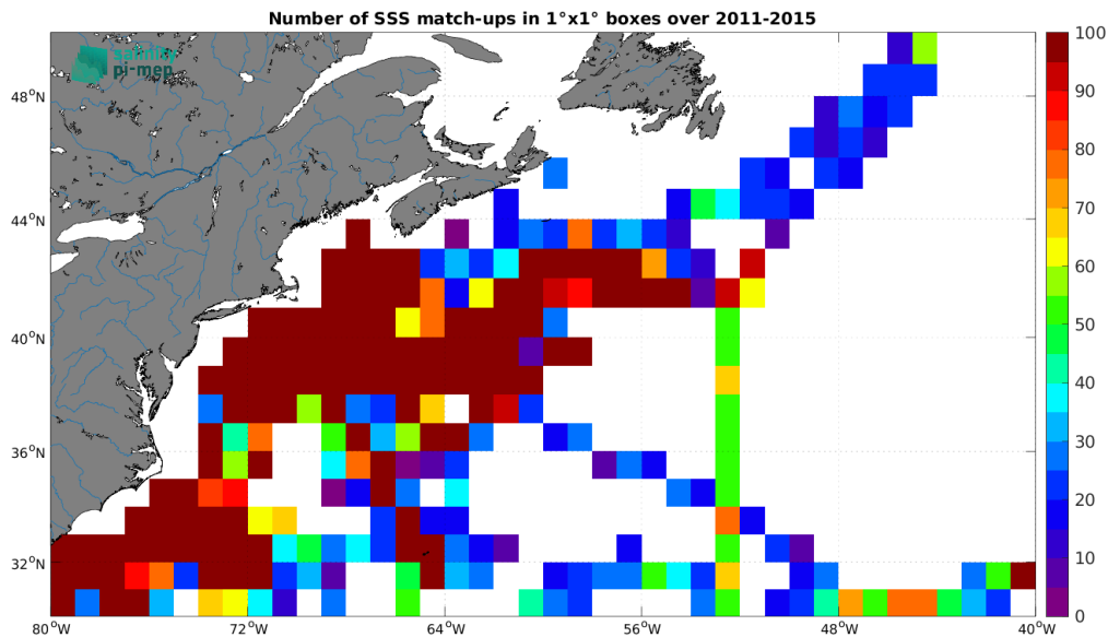
Figure 5: Number of SSS match-ups between TSG (SAMOS) SSS and the Aquarius SSS L3 CAP v5 - Monthly (JPL) SSS product for the Gulf Stream Pi-MEP region over 1^\circ \times 1^\circ boxes and for the full satellite product period.
