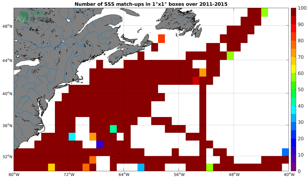
Figure 4: Number of SSS match-ups between TSG (SAMOS) SSS and the Aquarius SSS L3 CAP v5 - Monthly (JPL) SSS product for the Gulf Stream Pi-MEP region over 1^{\circ} \times 1^{\circ} boxes and for the full satellite product period.
