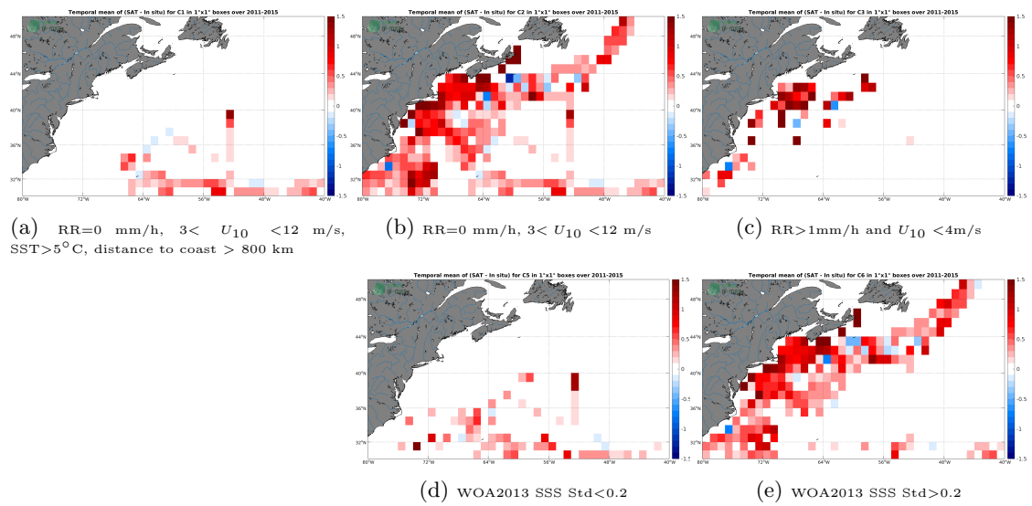
Figure 12: Temporal mean gridded over spatial boxes of size 1°x1° of \Delta SSS (Aquarius SSS L3 CAP v5 - Monthly (JPL) - TSG (SAMOS)) for 5 different subdatasets corresponding to:RR=0 mm/h, 3 < U_{10} < 12 m/s, SST > 5°C, distance to coast > 800 km (a), RR=0 mm/h, 3 < U_{10} < 12 m/s (b), RR > 1mm/h and U_{10} < 4 m/s (c), WOA2013 SSS Std < 0.2 (d), WOA2013 SSS Std > 0.2 (e).
