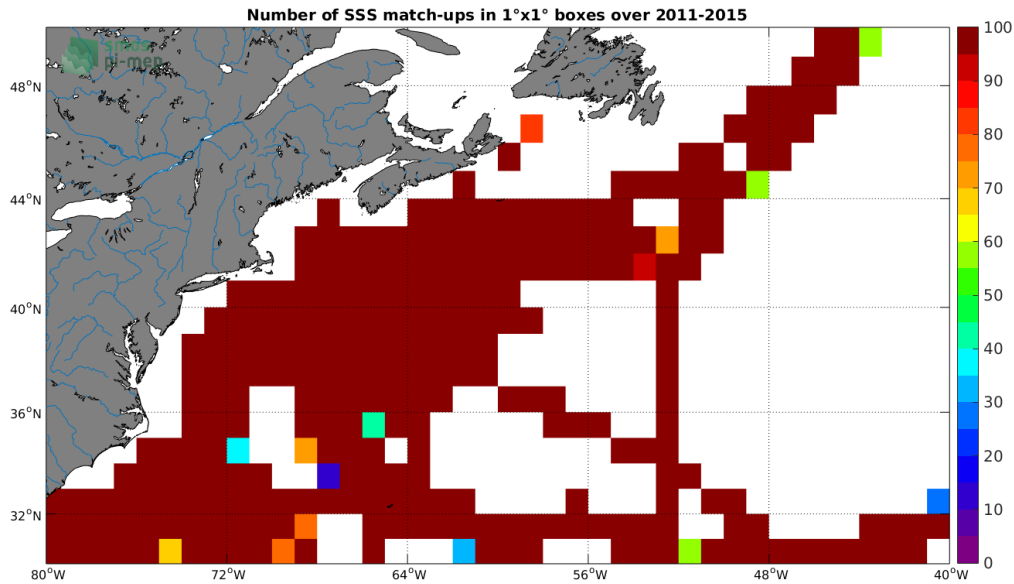
Figure 4: Number of SSS match-ups between TSG-SAMOS SSS and the Aquarius-L3-JPL-V5-MONTHLY SSS product for the Gulf Stream Pi-MEP region over 1°x1° boxes and for the full satellite product period.
