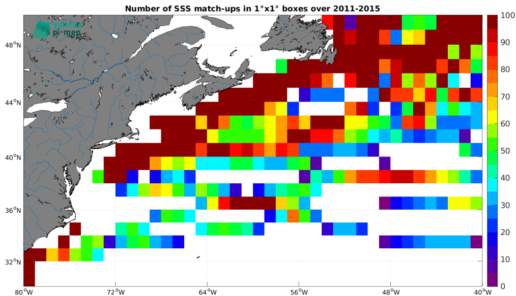
Figure 5: Number of SSS match-ups between TSG (LEGOS-DM) SSS and the Aquarius SSS L3 CAP v5 - Monthly (JPL) SSS product for the Gulf Stream Pi-MEP region over 1^\circ \times 1^\circ boxes and for the full satellite product period.
