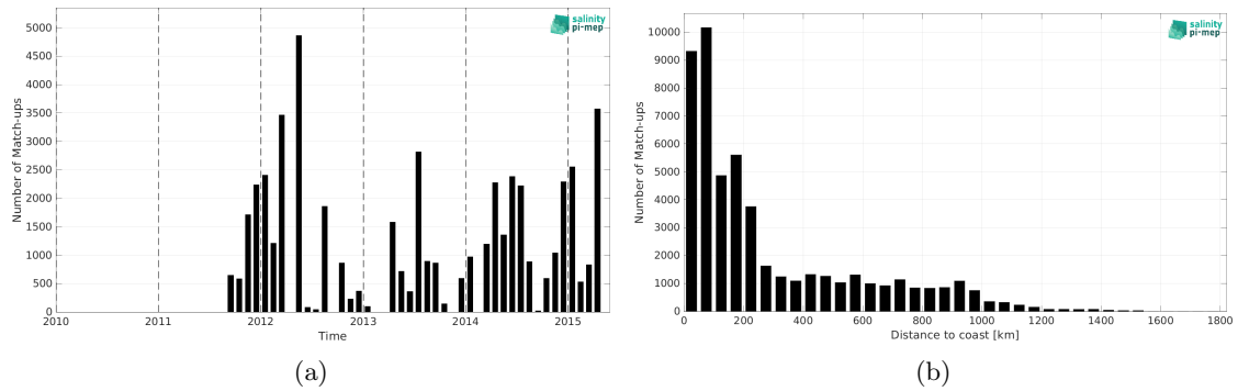
Figure 2: Number of match-ups between TSG (LEGOS-DM) and Aquarius SSS L3 CAP v5 - Monthly (JPL) SSS as a function of time (a) and as function of the distance to coast (b) over the Gulf Stream Pi-MEP region and for the full satellite product period.
