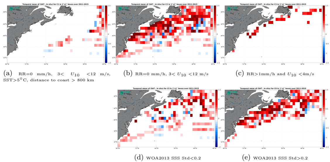
Figure 14: Temporal mean gridded over spatial boxes of size 1^\circ \times 1^\circ of \Delta SSS (Aquarius SSS L3 CAP v5 - Monthly (JPL) - TSG (LEGOS-DM)) for 5 different subdatasets corresponding to: RR=0 mm/h, 3 < U_{10} < 12 m/s, SST > 5°C, distance to coast > 800 km (a), RR=0 mm/h, 3 < U_{10} < 12 m/s (b), RR > 1mm/h and U_{10} < 4 m/s (c), WOA2013 SSS Std < 0.2 (d), WOA2013 SSS Std > 0.2 (e).
