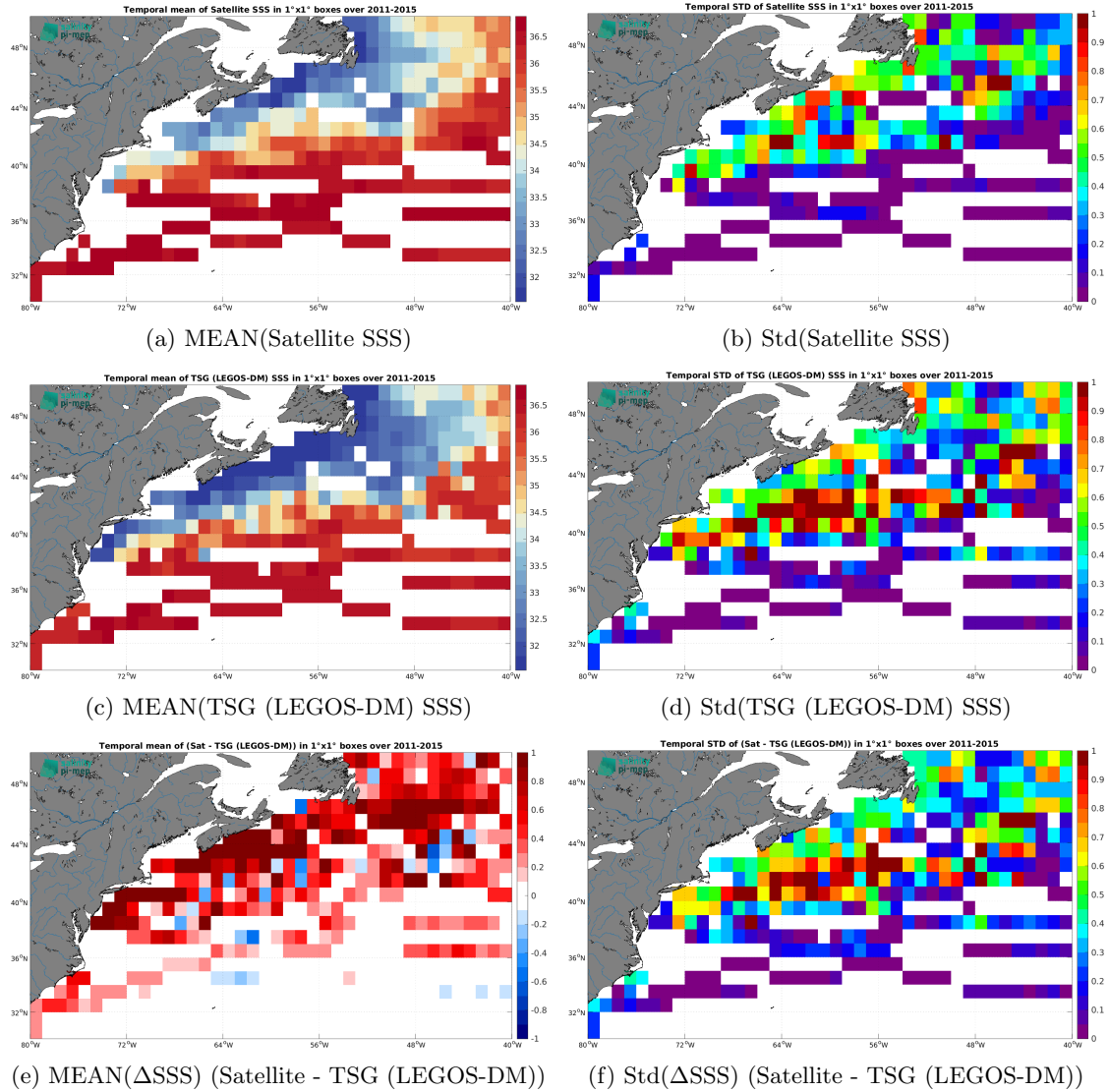
Figure 7: Temporal mean (left) and Std (right) of SSS from Aquarius SSS L3 CAP v5 - Monthly (JPL) (top), TSG (LEGOS-DM) (middle), and of \Delta SSS (Satellite - TSG (LEGOS-DM)). Only match-up pairs are used to generate these maps.
