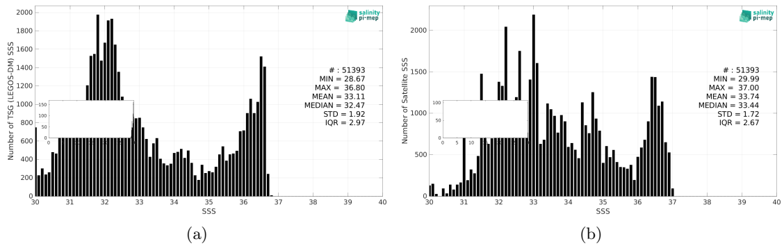
Figure 3: Histograms of SSS from TSG (LEGOS-DM) (a) and Aquarius SSS L3 CAP v5 - Monthly (JPL) (b) considering all match-up pairs per bins of 0.1 over the Gulf Stream Pi-MEP region and for the full satellite product period.
