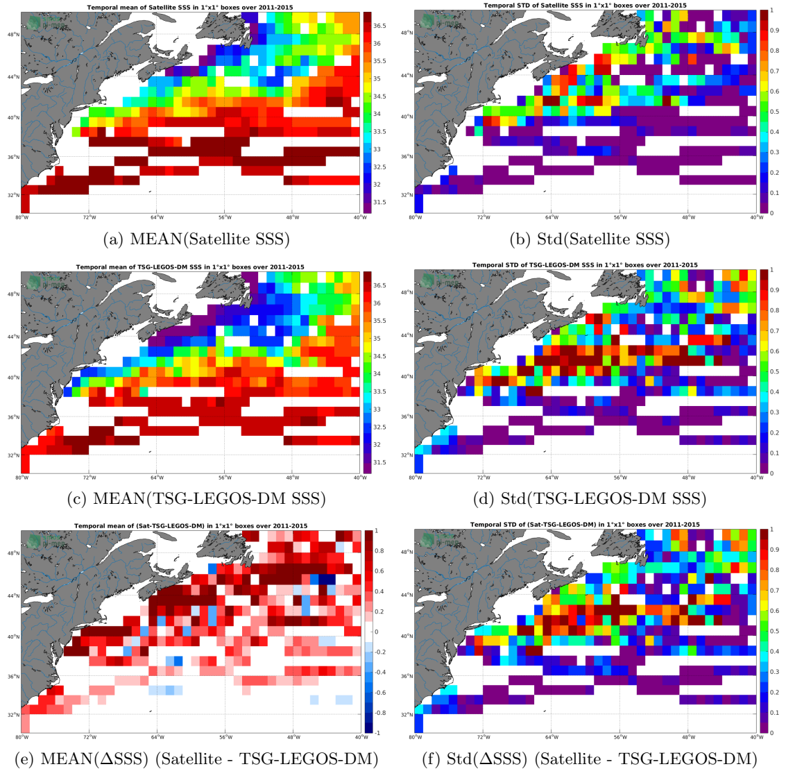
Figure 6: Temporal mean (left) and Std (right) of SSS from Aquarius-L3-JPL-V5-MONTHLY (top), TSG-LEGOS-DM (middle), and of \Delta\text{SSS} (Satellite - TSG-LEGOS-DM). Only match-up pairs are used to generate these maps.
