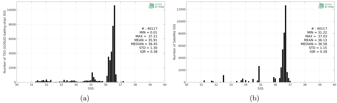
Figure 2: Histograms of SSS from TSG (GOSUD-Sailing-ship) (a) and Aquarius SSS L3 CAP v5 - Monthly (JPL) (b) considering all match-up pairs per bins of 0.1 over the Gulf Stream Pi-MEP region and for the full satellite product period.
