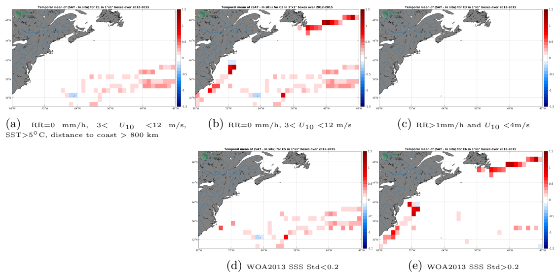
Figure 12: Temporal mean gridded over spatial boxes of size 1°x1° of \Delta SSS (Aquarius SSS L3 CAP v5 - Monthly (JPL) - TSG (GOSUD-Sailing-ship)) for 5 different subdatasets corresponding to:RR=0 mm/h, 3 < U_{10} < 12 m/s, SST>5°C, distance to coast > 800 km (a), RR=0 mm/h, 3 < U_{10} < 12 m/s (b), RR>1mm/h and U_{10} < 4 m/s (c), WOA2013 SSS Std<0.2 (d), WOA2013 SSS Std>0.2 (e).
