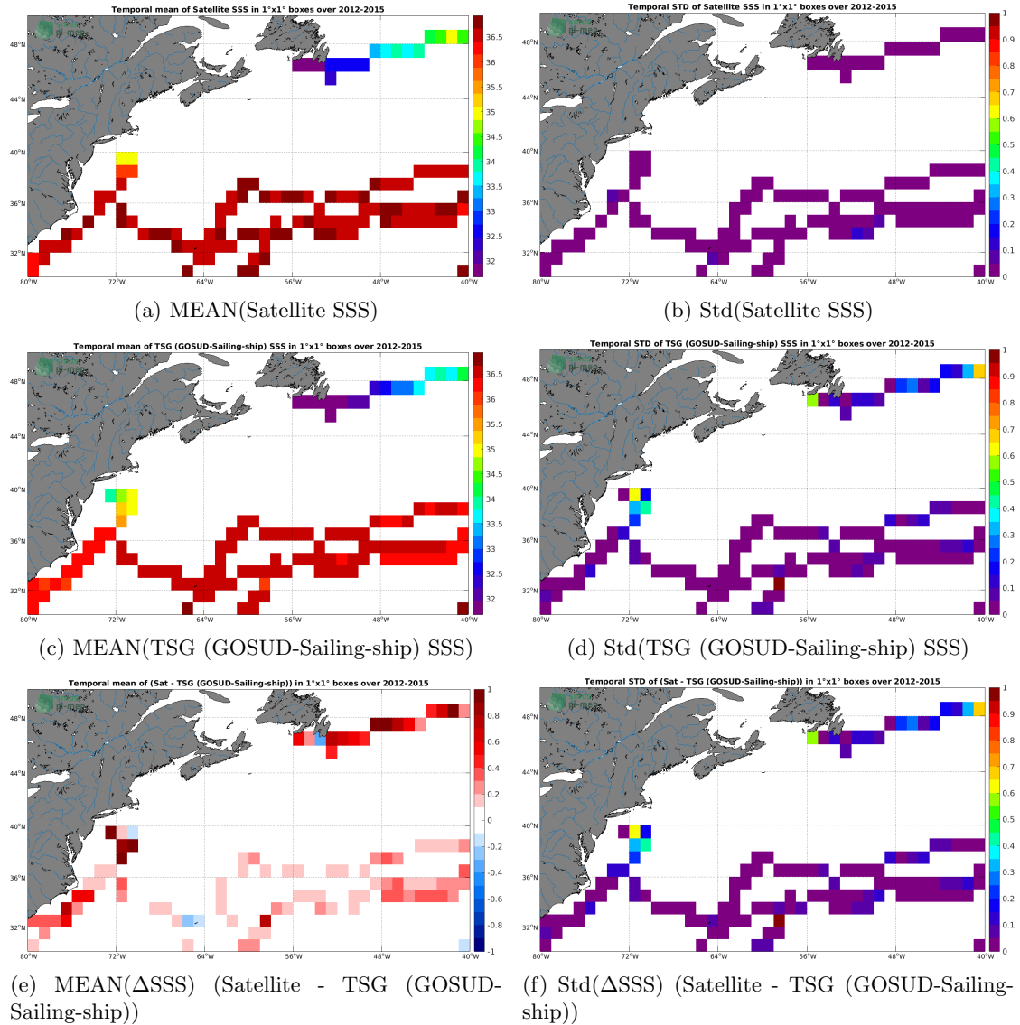
Figure 6: Temporal mean (left) and Std (right) of SSS from Aquarius SSS L3 CAP v5 - Monthly (JPL) (top), TSG (GOSUD-Sailing-ship) (middle), and of \Delta\text{SSS} (Satellite - TSG (GOSUD-Sailing-ship)). Only match-up pairs are used to generate these maps.
