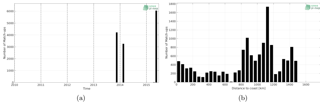
Figure 1: Number of match-ups between TSG-GOSUD-Sailing-ship and Aquarius-L3-JPL-V5-MONTHLY SSS as a function of time (a) and as function of the distance to coast (b) over the Gulf Stream Pi-MEP region and for the full satellite product period.
