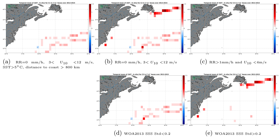
Figure 12: Temporal mean gridded over spatial boxes of size 1^\circ \times 1^\circ of \Delta SSS (Aquarius-L3-JPL-V5-MONTHLY - TSG-GOSUD-Sailing-ship) for 5 different subdatasets corresponding to:RR=0 mm/h, 3 < U_{10} < 12 m/s, SST >5^\circ C, distance to coast > 800 km (a), RR=0 mm/h, 3 < U_{10} < 12 m/s (b), RR >1 mm/h and U_{10} < 4 m/s (c), WOA2013 SSS Std <0.2 (d), WOA2013 SSS Std >0.2 (e).
