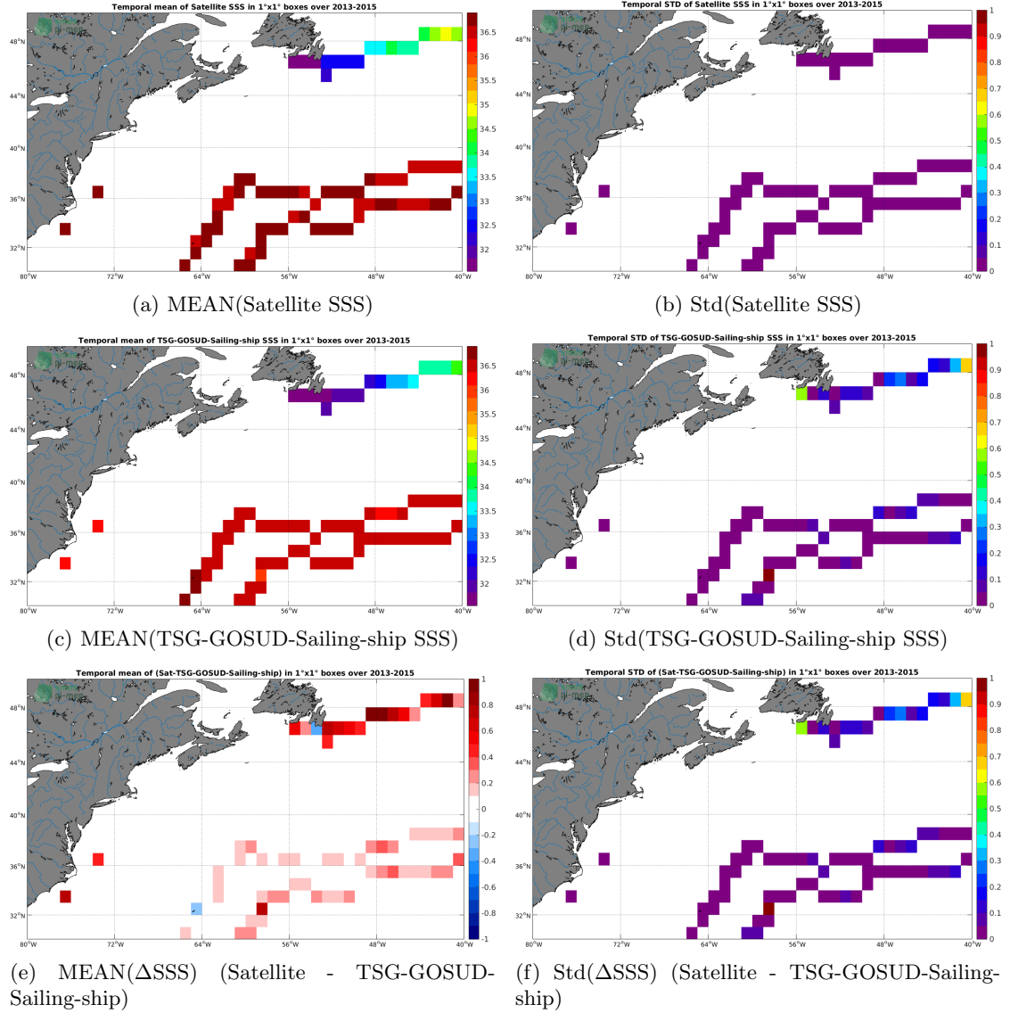
Figure 6: Temporal mean (left) and Std (right) of SSS from Aquarius-L3-JPL-V5-MONTHLY (top), TSG-GOSUD-Sailing-ship (middle), and of \Delta SSS (Satellite - TSG-GOSUD-Sailing-ship). Only match-up pairs are used to generate these maps.
