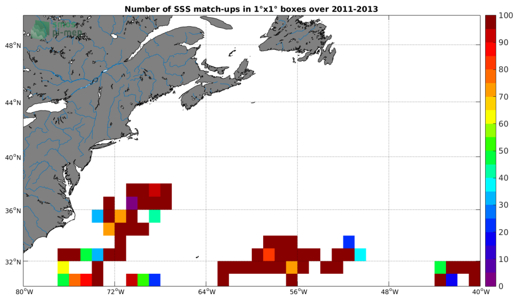
Figure 3: Number of SSS match-ups between Surface drifters SSS and the Aquarius-L3-JPL-V5-MONTHLY SSS product for the Gulf Stream Pi-MEP region over 1°x1° boxes and for the full satellite product period.
