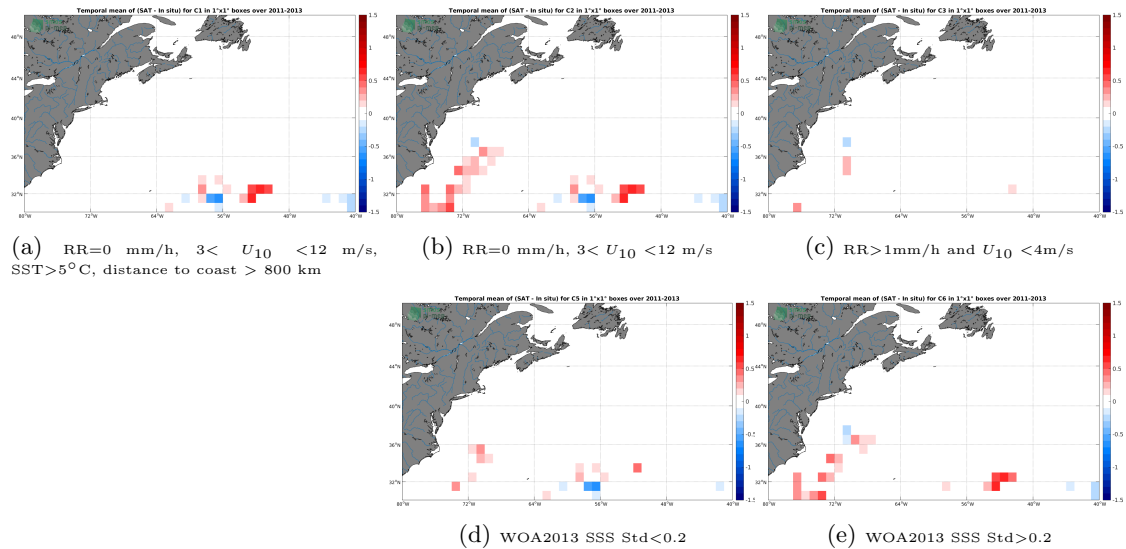
Figure 11: Temporal mean gridded over spatial boxes of size 1^{\circ}\times 1^{\circ} of \Delta\text{SSS} (Aquarius-L3-JPL-V5-MONTHLY - Surface drifters) for 5 different subdatasets corresponding to:RR=0 mm/h, 3 < U_{10} < 12 m/s, SST >5^{\circ}\text{C} , distance to coast > 800 km (a), RR=0 mm/h, 3 < U_{10} < 12 m/s (b), RR >1 mm/h and U_{10} < 4 m/s (c), WOA2013 SSS Std <0.2 (d), WOA2013 SSS Std >0.2 (e).
