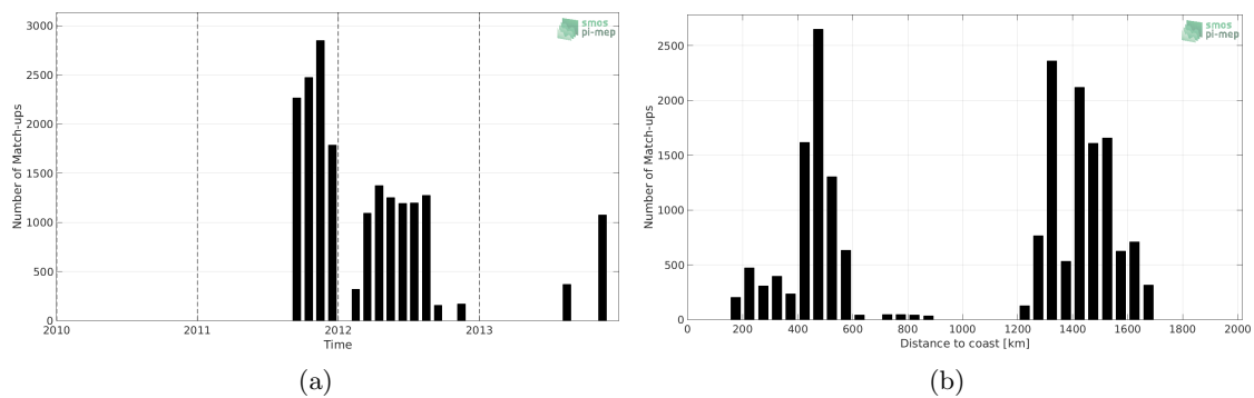
Figure 1: Number of match-ups between Surface drifters and Aquarius-L3-JPL-V5-MONTHLY SSS as a function of time (a) and as function of the distance to coast (b) over the Gulf Stream Pi-MEP region and for the full satellite product period.
