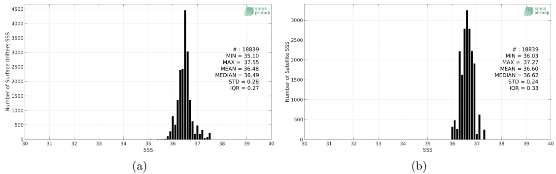
Figure 2: Histograms of SSS from Surface drifters (a) and Aquarius-L3-JPL-V5-MONTHLY (b) considering all match-up pairs per bins of 0.1 over the Gulf Stream Pi-MEP region and for the full satellite product period.
