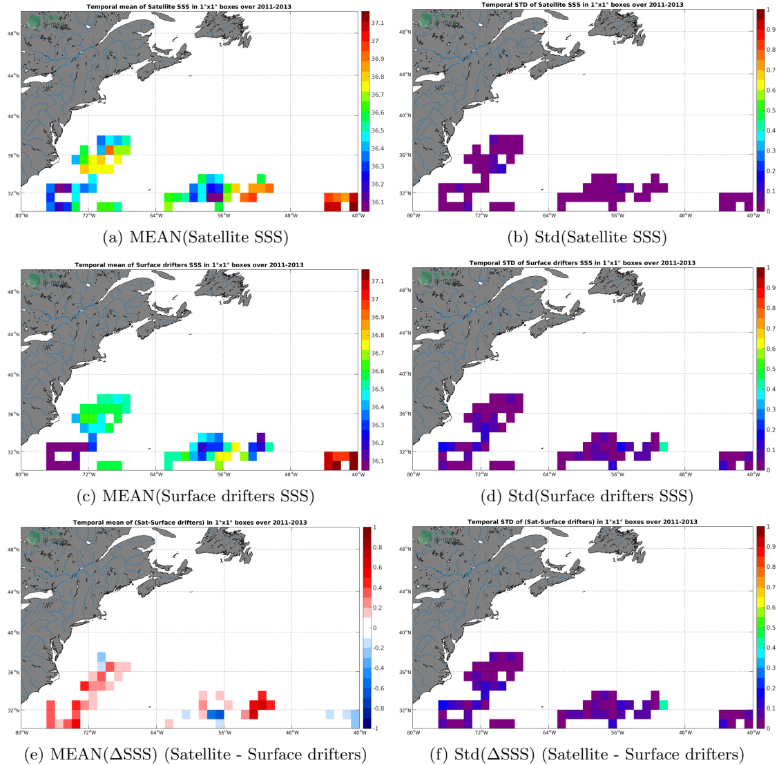
Figure 5: Temporal mean (left) and Std (right) of SSS from Aquarius-L3-JPL-V5-MONTHLY (top), Surface drifters (middle), and of \Delta SSS (Satellite - Surface drifters). Only match-up pairs are used to generate these maps.
