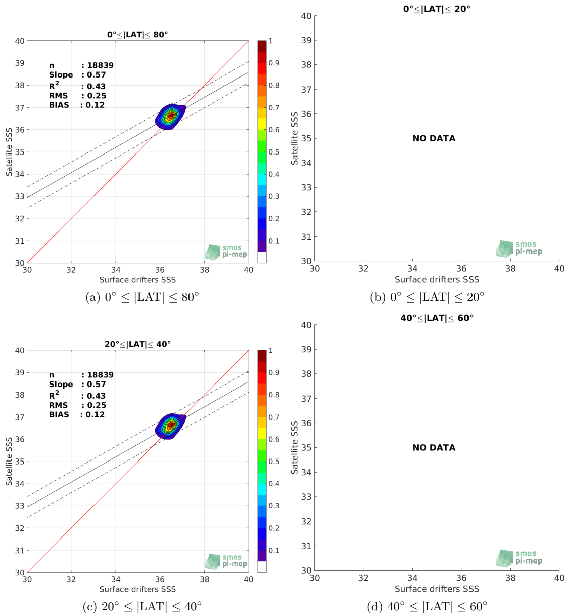
Figure 8: Contour maps of the concentration of Aquarius-L3-JPL-V5-MONTHLY SSS (y-axis) versus Surface drifters SSS (x-axis) at match-up pairs for different latitude bands. For each plot, the red line shows x=y . The black thin and dashed lines indicate a linear fit through the data cloud and the \pm 95\% confidence levels, respectively. The number match-up pairs n , the slope and R^2 coefficient of the linear fit, the root mean square (RMS) and the mean bias between satellite and in situ data are indicated for each latitude band in each plots.
