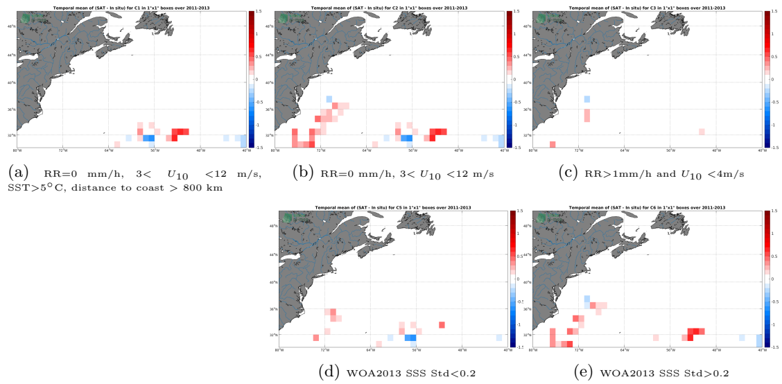
Figure 11: Temporal mean gridded over spatial boxes of size 1^\circ \times 1^\circ of \Delta SSS (Aquarius-L3-JPL-V5-MONTHLY - Surface drifters) for 5 different subdatasets corresponding to: RR=0 mm/h, 3 < U_{10} < 12 m/s, SST > 5^\circ C , distance to coast > 800 km (a), RR=0 mm/h, 3 < U_{10} < 12 m/s (b), RR > 1 mm/h and U_{10} < 4 m/s (c), WOA2013 SSS Std < 0.2 (d), WOA2013 SSS Std > 0.2 (e).
