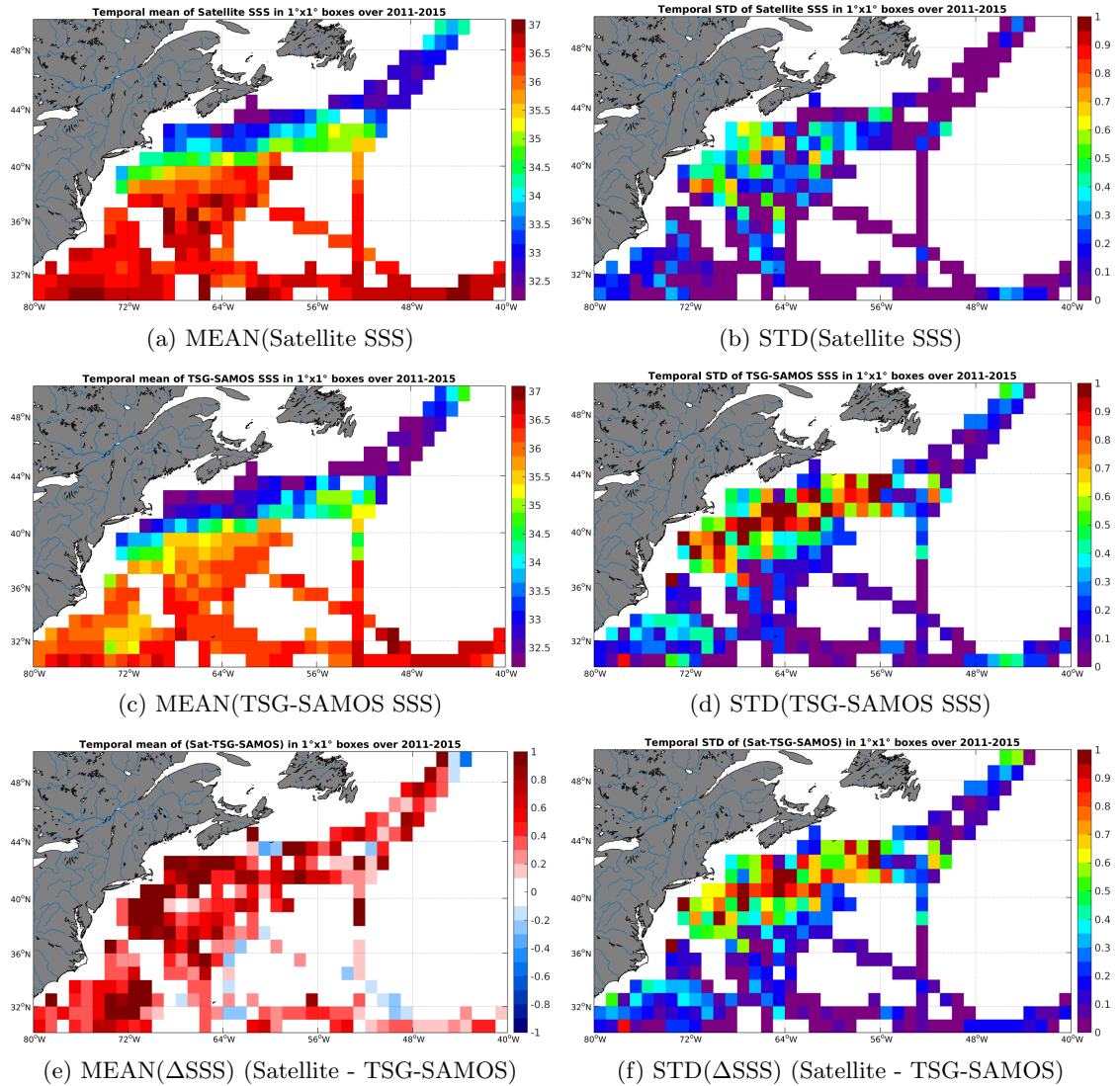
Figure 6: Temporal mean (left) and STD (right) of SSS from Aquarius-L3-JPL-V4-7DAY-RUNNING (top), TSG-SAMOS (middle), and of \Delta SSS (Satellite - TSG-SAMOS). Only match-up pairs are used to generate these maps.
