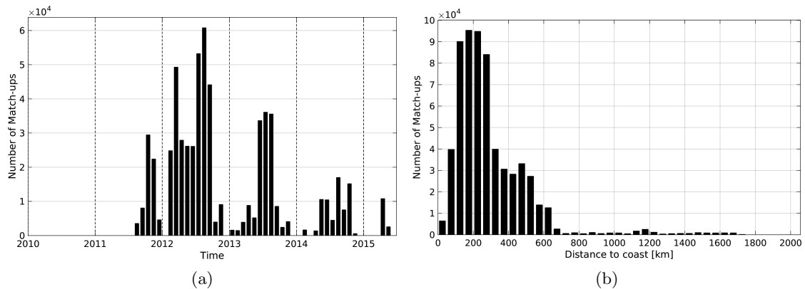
Figure 1: Number of match-ups between TSG-SAMOS and Aquarius-L3-JPL-V4-7DAY-RUNNING SSS as a function of time (a) and as function of the distance to coast (b) over the Gulf Stream Pi-MEP region and for the full satellite product period.
