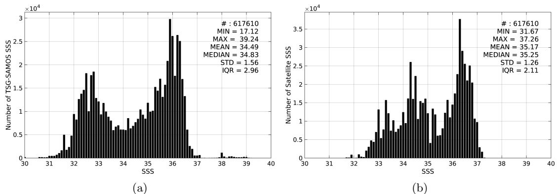
Figure 2: Histograms of SSS from TSG-SAMOS (a) and Aquarius-L3-JPL-V4-7DAY-RUNNING (b) considering all match-up pairs per bins of 0.1 over the Gulf Stream Pi-MEP region and for the full satellite product period.
