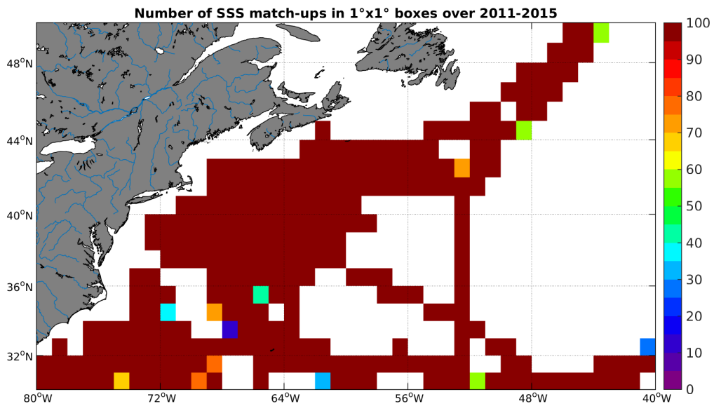
Figure 4: Number of SSS match-ups between TSG-SAMOS SSS and the Aquarius-L3-JPL-V4-7DAY-RUNNING SSS product for the Gulf Stream Pi-MEP region over 1^\circ \times 1^\circ boxes and for the full satellite product period.
