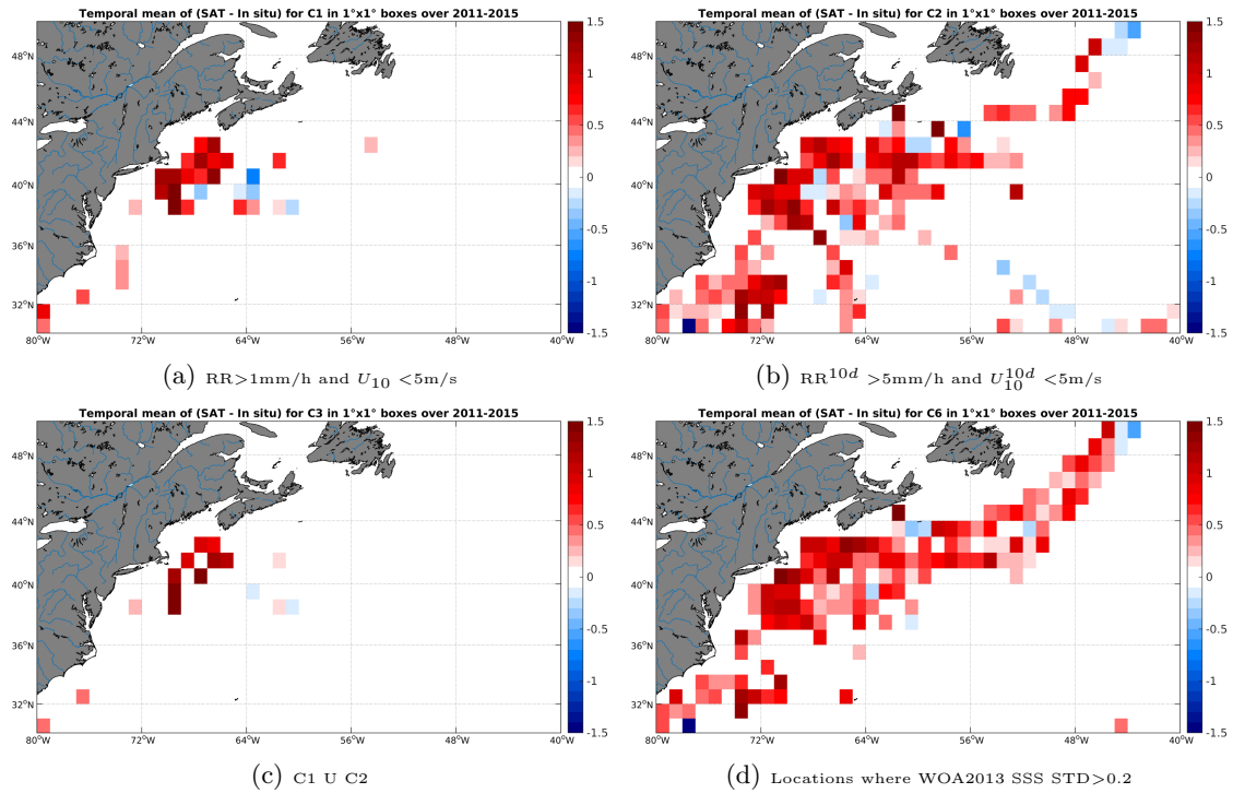
Figure 12: Temporal mean gridded over spatial boxes of size 1^\circ \times 1^\circ of \Delta SSS (Aquarius-L3-JPL-V4-7DAY-RUNNING - TSG-SAMOS) for 4 different subdatasets corresponding to:RR>1mm/h and U_{10} < 5\text{m/s} (a), RR^{10d} > 5\text{mm/h} and U_{10}^{10d} < 5\text{m/s} (b), C1 U C2 (c),Locations where WOA2013 SSS STD>0.2 (d).
