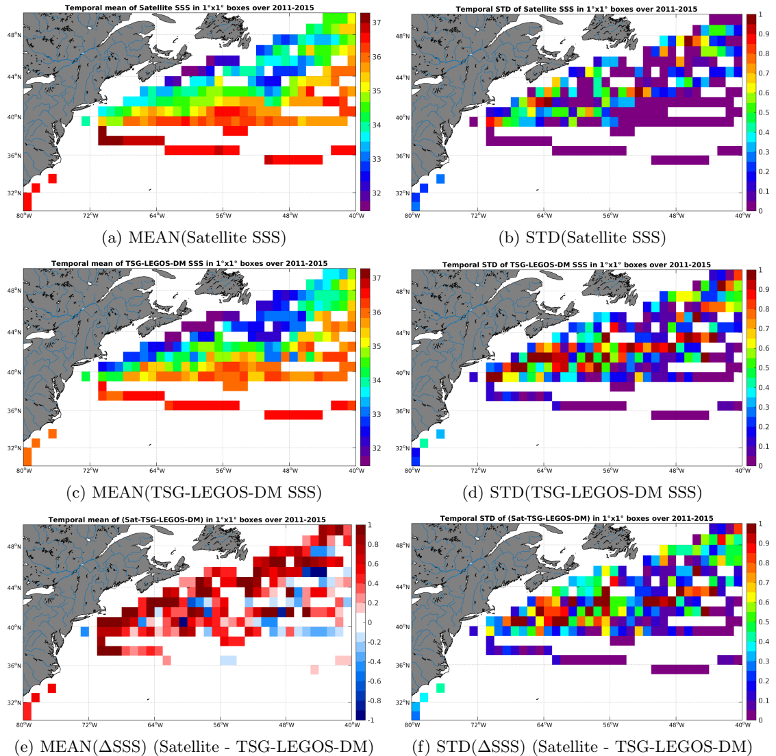
Figure 6: Temporal mean (left) and STD (right) of SSS from Aquarius-L3-JPL-V4-7DAY-RUNNING (top), TSG-LEGOS-DM (middle), and of \Delta SSS (Satellite - TSG-LEGOS-DM). Only match-up pairs are used to generate these maps.
