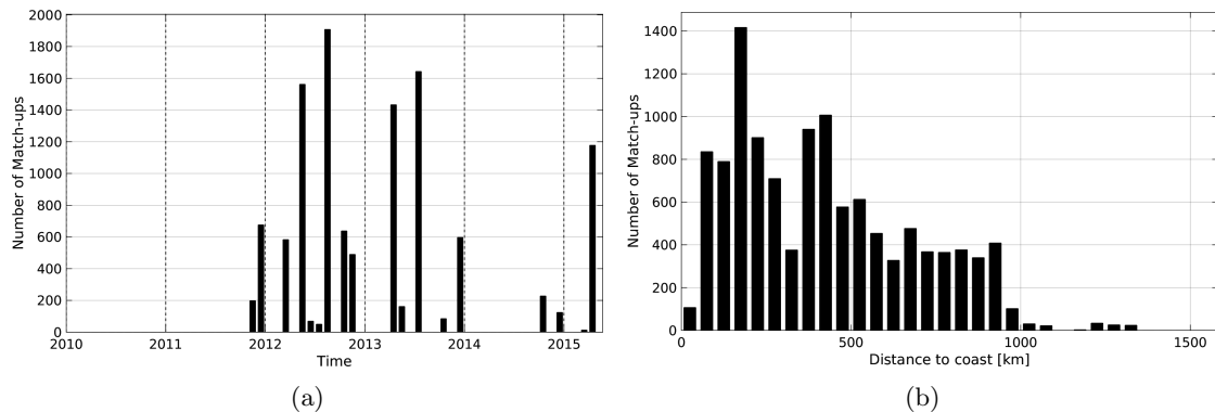
Figure 1: Number of match-ups between TSG-LEGOS-DM and Aquarius-L3-JPL-V4-7DAY-RUNNING SSS as a function of time (a) and as function of the distance to coast (b) over the Gulf Stream Pi-MEP region and for the full satellite product period.
