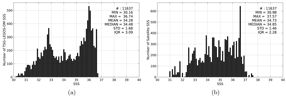
Figure 2: Histograms of SSS from TSG-LEGOS-DM (a) and Aquarius-L3-JPL-V4-7DAY-RUNNING (b) considering all match-up pairs per bins of 0.1 over the Gulf Stream Pi-MEP region and for the full satellite product period.
