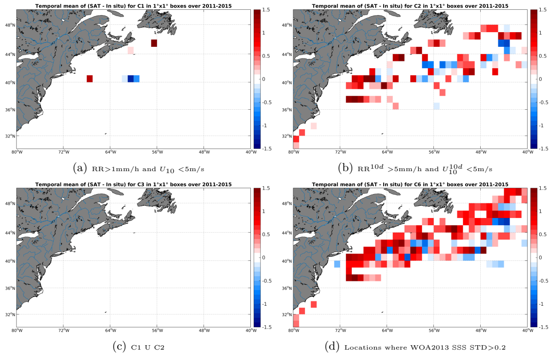
Figure 12: Temporal mean gridded over spatial boxes of size 1^\circ \times 1^\circ of \Delta SSS (Aquarius-L3-JPL-V4-7DAY-RUNNING - TSG-LEGOS-DM) for 4 different subdatasets corresponding to: RR > 1mm/h and U_{10} < 5\text{m/s} (a), RR^{10d} > 5\text{mm/h} and U_{10}^{10d} < 5\text{m/s} (b), C1 U C2 (c), Locations where WOA2013 SSS STD > 0.2 (d).
