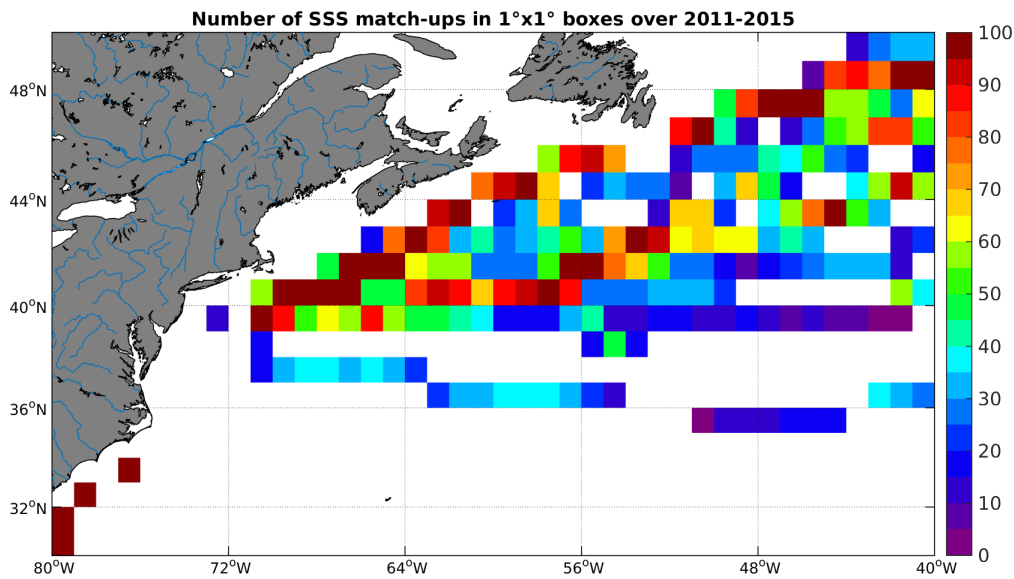
Figure 4: Number of SSS match-ups between TSG-LEGOS-DM SSS and the Aquarius-L3-JPL-V4-7DAY-RUNNING SSS product for the Gulf Stream Pi-MEP region over 1^\circ \times 1^\circ boxes and for the full satellite product period.
