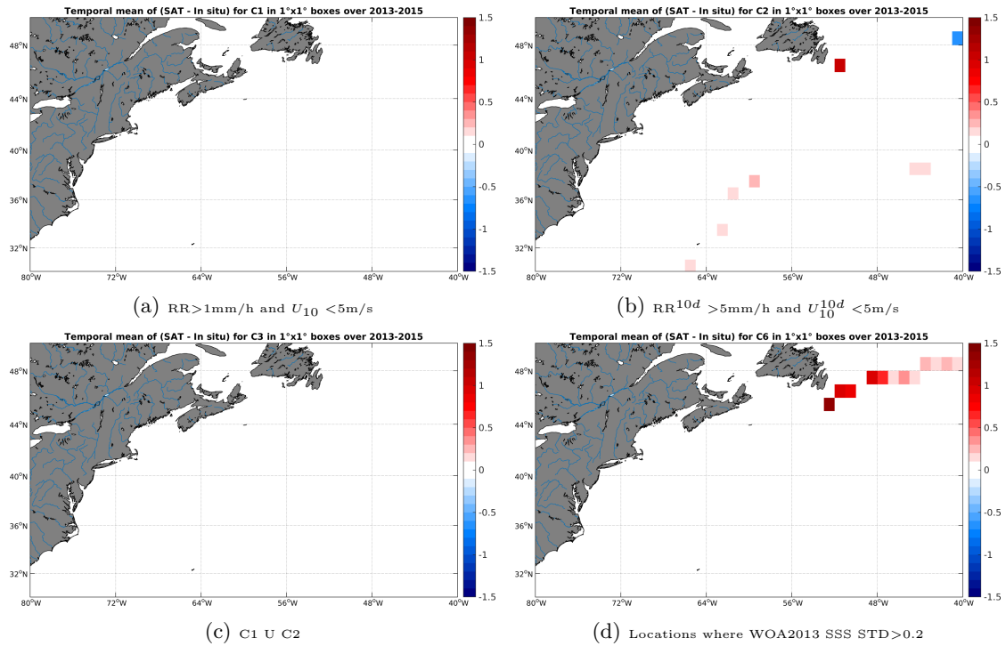
Figure 12: Temporal mean gridded over spatial boxes of size 1°x1° of \Delta SSS (Aquarius-L3-JPL-V4-7DAY-RUNNING - TSG-GOSUD-Sailing-ship) for 4 different subdatasets corresponding to:RR>1mm/h and U_{10} < 5\text{m/s} (a), RR^{10d} > 5\text{mm/h} and U_{10}^{10d} < 5\text{m/s} (b), C1 U C2 (c),Locations where WOA2013 SSS STD>0.2 (d).
