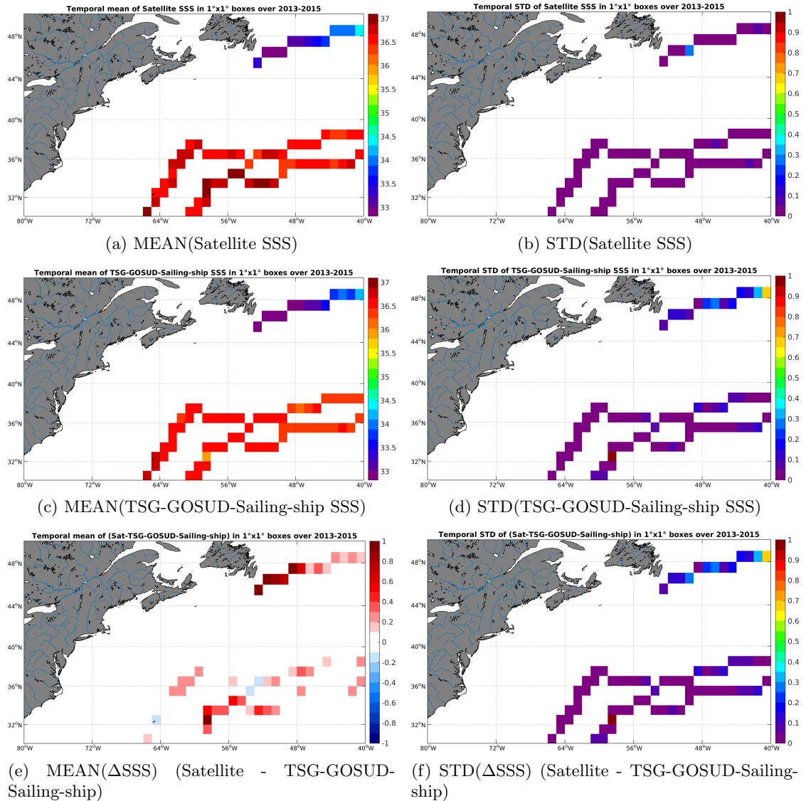
Figure 6: Temporal mean (left) and STD (right) of SSS from Aquarius-L3-JPL-V4-7DAY-RUNNING (top), TSG-GOSUD-Sailing-ship (middle), and of \Delta SSS (Satellite - TSG-GOSUD-Sailing-ship). Only match-up pairs are used to generate these maps.
