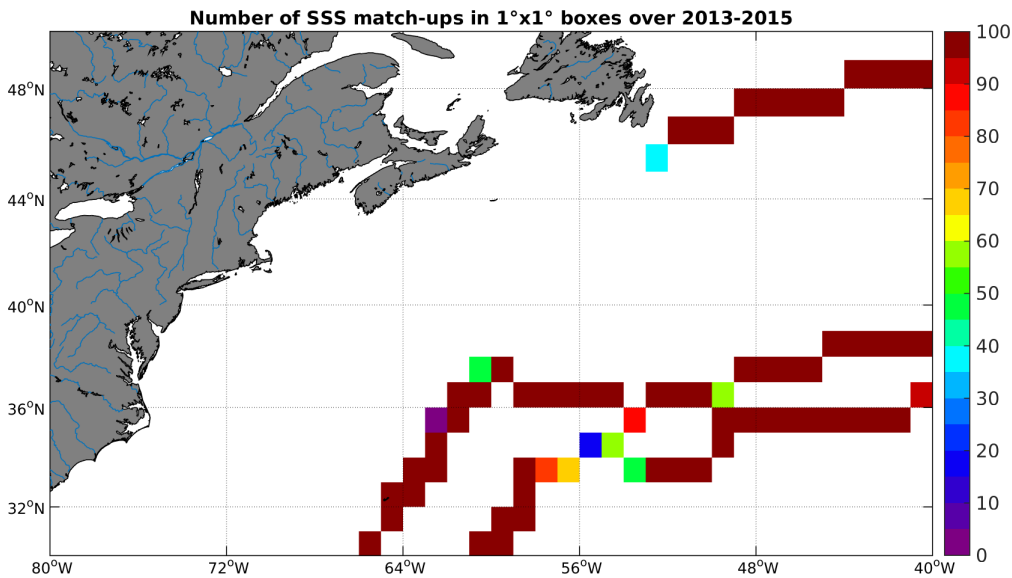
Figure 4: Number of SSS match-ups between TSG-GOSUD-Sailing-ship SSS and the Aquarius-L3-JPL-V4-7DAY-RUNNING SSS product for the Gulf Stream Pi-MEP region over 1°x1° boxes and for the full satellite product period.
