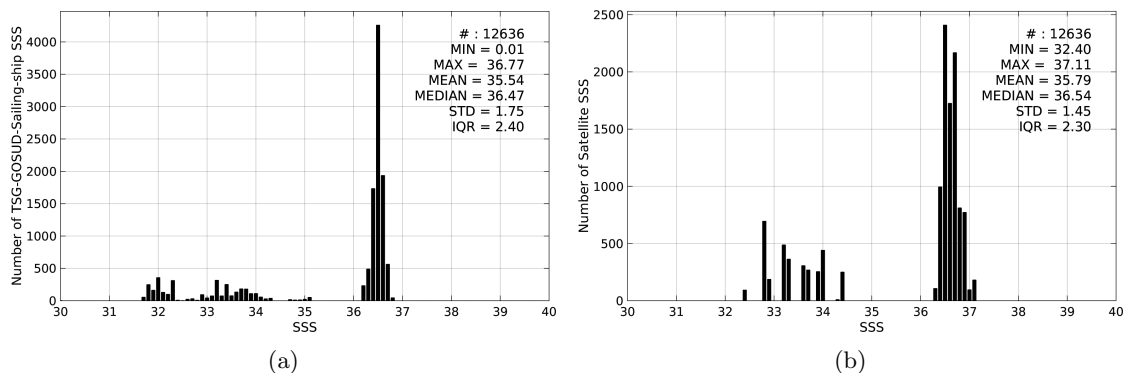
Figure 2: Histograms of SSS from TSG-GOSUD-Sailing-ship (a) and Aquarius-L3-JPL-V4-7DAY-RUNNING (b) considering all match-up pairs per bins of 0.1 over the Gulf Stream Pi-MEP region and for the full satellite product period.
