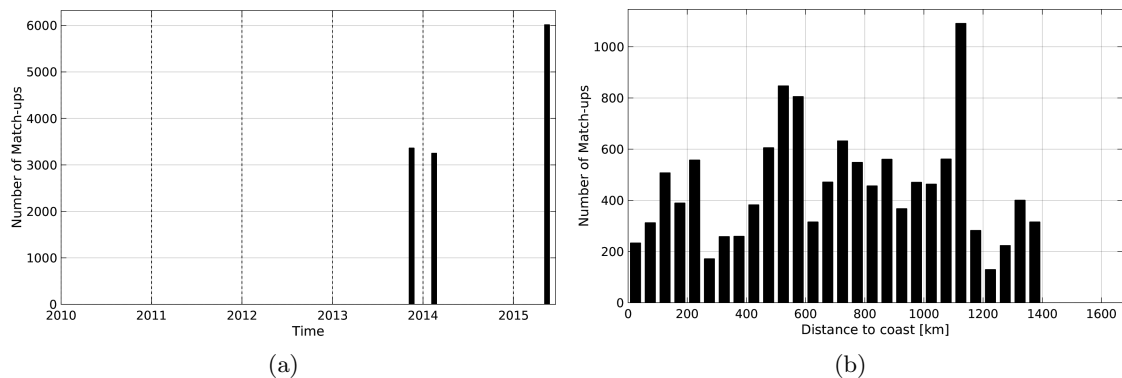
Figure 1: Number of match-ups between TSG-GOSUD-Sailing-ship and Aquarius-L3-JPL-V4-7DAY-RUNNING SSS as a function of time (a) and as function of the distance to coast (b) over the Gulf Stream Pi-MEP region and for the full satellite product period.
