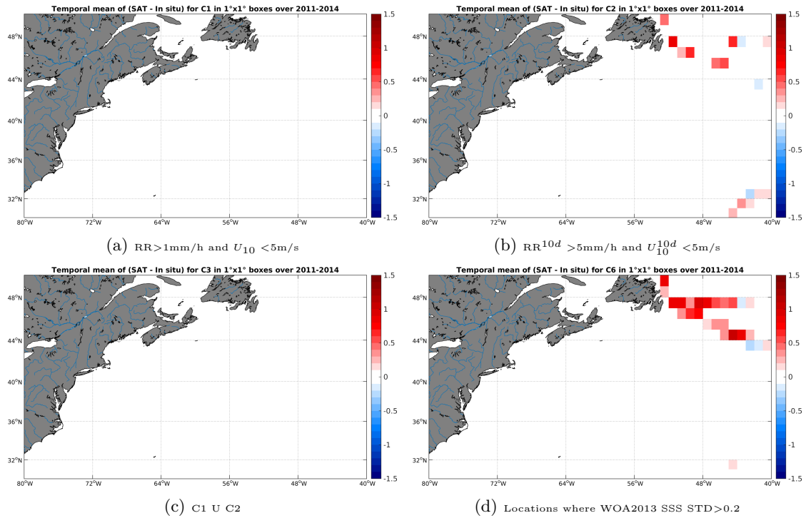
Figure 12: Temporal mean gridded over spatial boxes of size 1°x1° of \Delta SSS (Aquarius-L3-JPL-V4-7DAY-RUNNING - TSG-GOSUD-Research-vessel) for 4 different subdatasets corresponding to:RR>1mm/h and U_{10} < 5m/s (a), RR^{10d} > 5mm/h and U_{10}^{10d} < 5m/s (b), C1 U C2 (c),Locations where WOA2013 SSS STD>0.2 (d).
