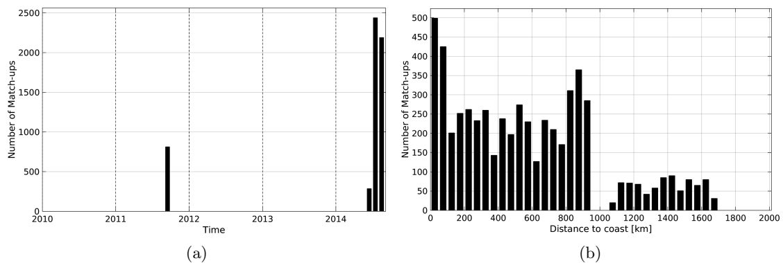
Figure 1: Number of match-ups between TSG-GOSUD-Research-vessel and Aquarius-L3-JPL-V4-7DAY-RUNNING SSS as a function of time (a) and as function of the distance to coast (b) over the Gulf Stream Pi-MEP region and for the full satellite product period.
