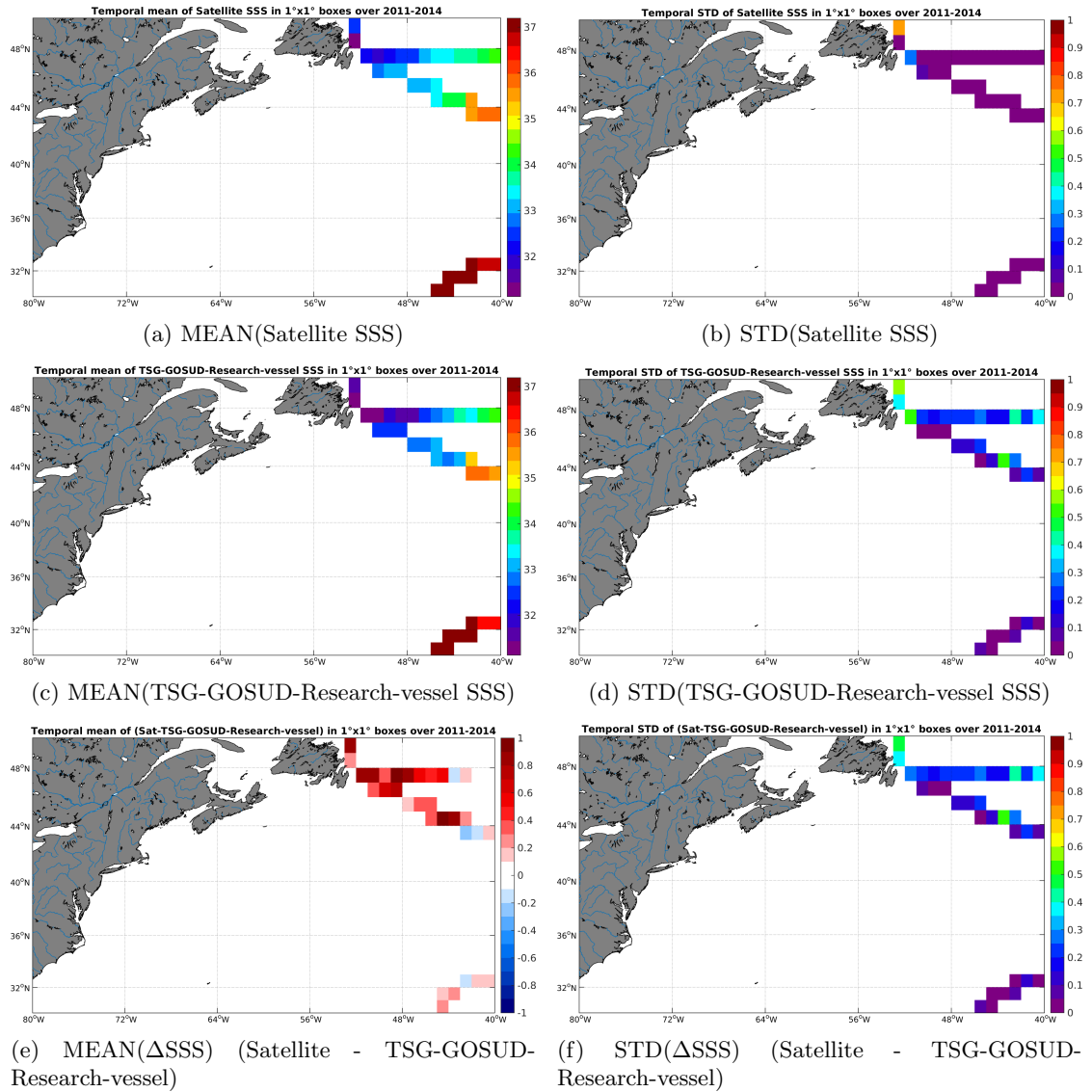
Figure 6: Temporal mean (left) and STD (right) of SSS from Aquarius-L3-JPL-V4-7DAY-RUNNING (top), TSG-GOSUD-Research-vessel (middle), and of \Delta SSS (Satellite - TSG-GOSUD-Research-vessel). Only match-up pairs are used to generate these maps.
