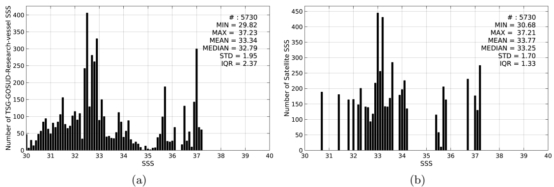
Figure 2: Histograms of SSS from TSG-GOSUD-Research-vessel (a) and Aquarius-L3-JPL-V4-7DAY-RUNNING (b) considering all match-up pairs per bins of 0.1 over the Gulf Stream Pi-MEP region and for the full satellite product period.
