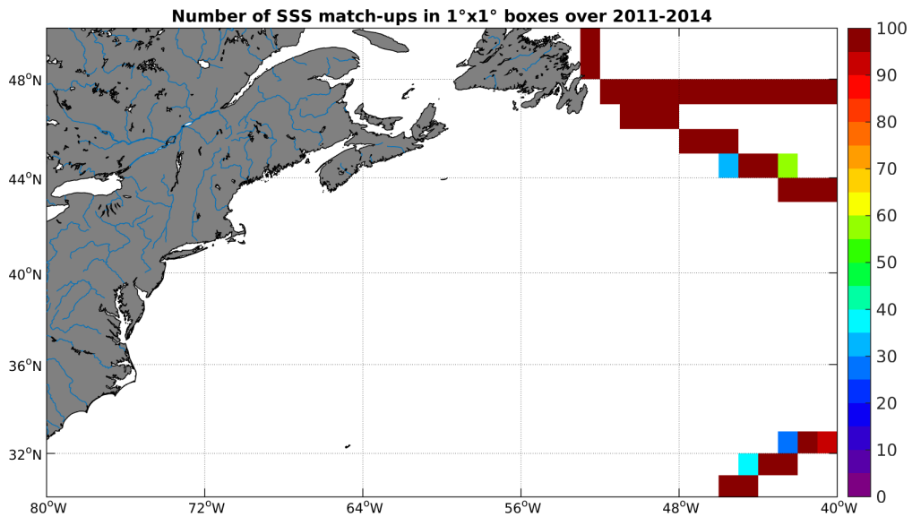
Figure 4: Number of SSS match-ups between TSG-GOSUD-Research-vessel SSS and the Aquarius-L3-JPL-V4-7DAY-RUNNING SSS product for the Gulf Stream Pi-MEP region over 1^\circ \times 1^\circ boxes and for the full satellite product period.
