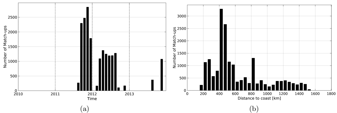
Figure 1: Number of match-ups between Surface drifters and Aquarius-L3-JPL-V4-7DAY-RUNNING SSS as a function of time (a) and as function of the distance to coast (b) over the Gulf Stream Pi-MEP region and for the full satellite product period.
