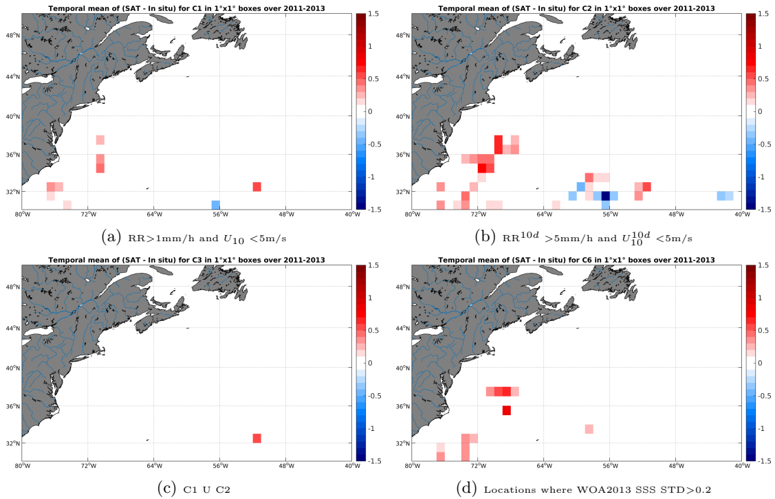
Figure 11: Temporal mean gridded over spatial boxes of size 1^\circ \times 1^\circ of \Delta SSS (Aquarius-L3-JPL-V4-7DAY-RUNNING - Surface drifters) for 4 different subdatasets corresponding to: RR > 1\text{mm/h} and U_{10} < 5\text{m/s} (a), RR^{10d} > 5\text{mm/h} and U_{10}^{10d} < 5\text{m/s} (b), C1 U C2 (c), Locations where WOA2013 SSS STD > 0.2 (d).
