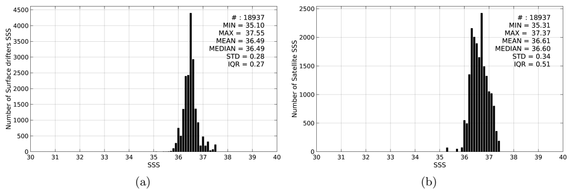
Figure 2: Histograms of SSS from Surface drifters (a) and Aquarius-L3-JPL-V4-7DAY-RUNNING (b) considering all match-up pairs per bins of 0.1 over the Gulf Stream Pi-MEP region and for the full satellite product period.
