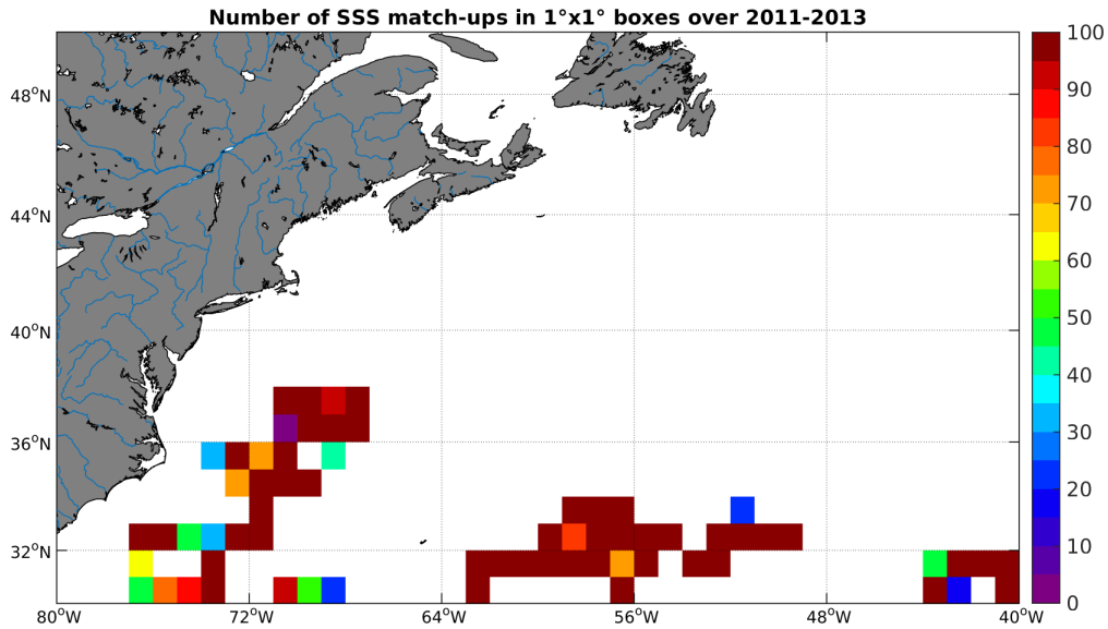
Figure 3: Number of SSS match-ups between Surface drifters SSS and the Aquarius-L3-JPL-V4-7DAY-RUNNING SSS product for the Gulf Stream Pi-MEP region over 1^\circ \times 1^\circ boxes and for the full satellite product period.
