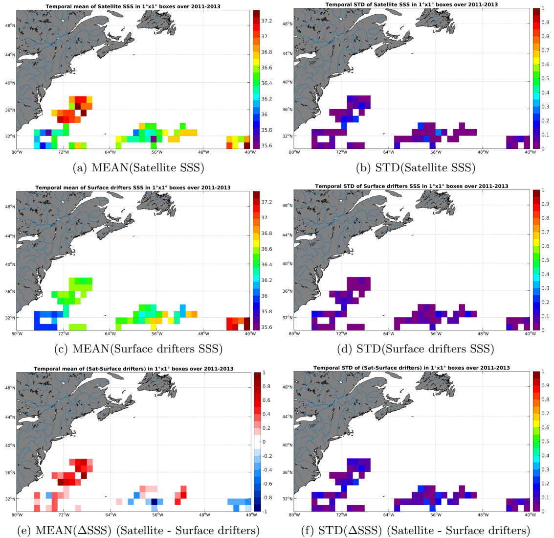
Figure 5: Temporal mean (left) and STD (right) of SSS from Aquarius-L3-JPL-V4-7DAY-RUNNING (top), Surface drifters (middle), and of \Delta SSS (Satellite - Surface drifters). Only match-up pairs are used to generate these maps.
