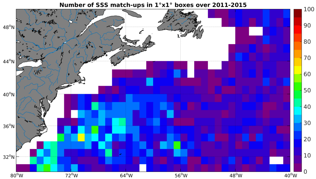
Figure 4: Number of SSS match-ups between Argo SSS and the Aquarius-L3-JPL-V4-7DAY-RUNNING SSS product for the Gulf Stream Pi-MEP region over 1^\circ \times 1^\circ boxes and for the full satellite product period.
