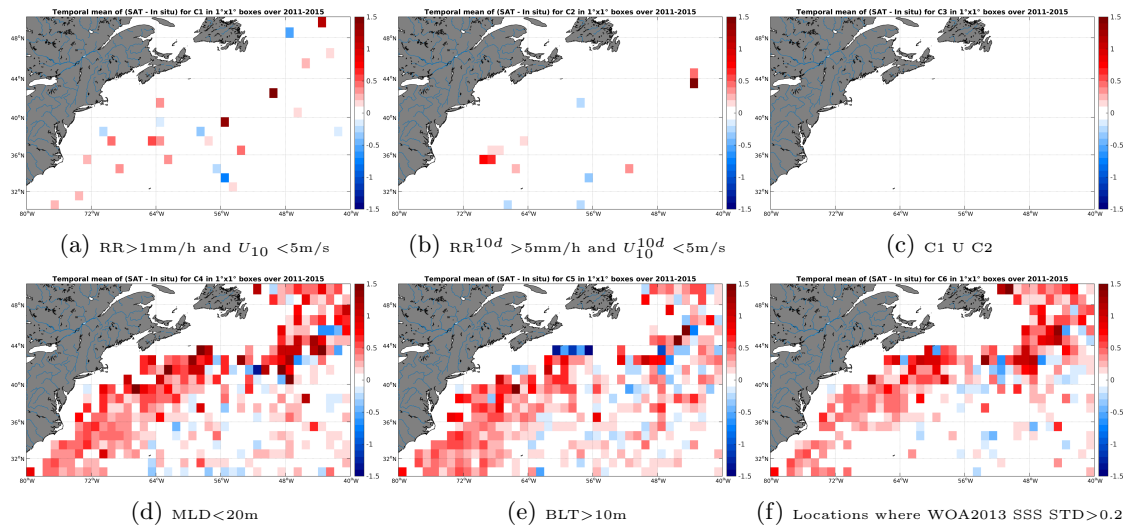
Figure 12: Temporal mean gridded over spatial boxes of size 1^\circ \times 1^\circ of \Delta SSS (Aquarius-L3-JPL-V4-7DAY-RUNNING - Argo) for 6 different subdatasets corresponding to: RR > 1\text{mm/h} and U_{10} < 5\text{m/s} (a), RR^{10d} > 5\text{mm/h} and U_{10}^{10d} < 5\text{m/s} (b), C1 U C2 (c), MLD < 20\text{m} (d), BLT > 10\text{m} (e), Locations where WOA2013 SSS STD > 0.2 (f).
