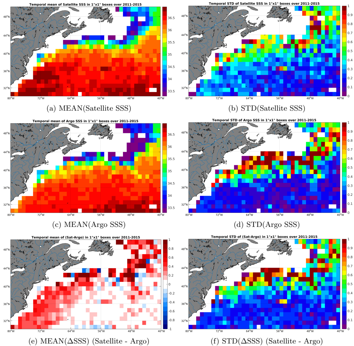
Figure 6: Temporal mean (left) and STD (right) of SSS from Aquarius-L3-JPL-V4-7DAY-RUNNING (top), Argo (middle), and of \Delta SSS (Satellite - Argo). Only match-up pairs are used to generate these maps.
