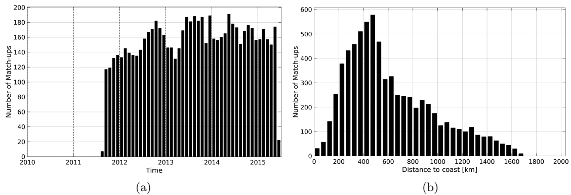
Figure 1: Number of match-ups between Argo and Aquarius-L3-JPL-V4-7DAY-RUNNING SSS as a function of time (a) and as function of the distance to coast (b) over the Gulf Stream Pi-MEP region and for the full satellite product period.
