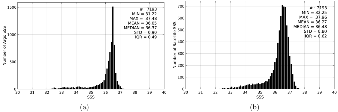
Figure 2: Histograms of SSS from Argo (a) and Aquarius-L3-JPL-V4-7DAY-RUNNING (b) considering all match-up pairs per bins of 0.1 over the Gulf Stream Pi-MEP region and for the full satellite product period.
