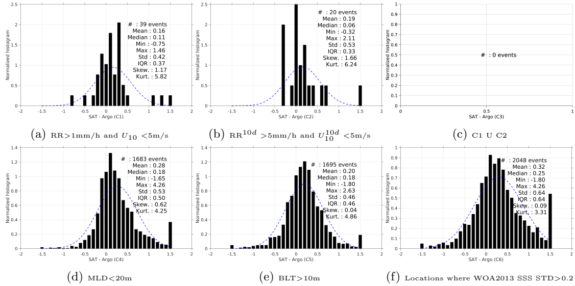
Figure 13: Normalized histogram of \Delta SSS (Aquarius-L3-JPL-V4-7DAY-RUNNING - Argo) for 6 different subdatasets corresponding to: RR>1mm/h and U_{10} < 5\text{m/s} (a), RR^{10d} > 5\text{mm/h} and U_{10}^{10d} < 5\text{m/s} (b), C1 U C2 (c),MLD<20m (d),BLT>10m (e),Locations where WOA2013 SSS STD>0.2 (f).
