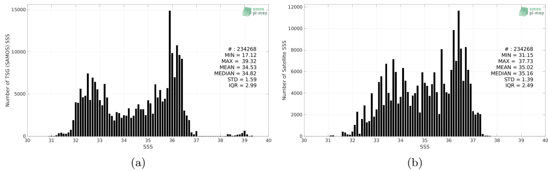
Figure 2: Histograms of SSS from TSG (SAMOS) (a) and Aquarius SSS L2 CAP v5 (JPL) (b) considering all match-up pairs per bins of 0.1 over the Gulf Stream Pi-MEP region and for the full satellite product period.
