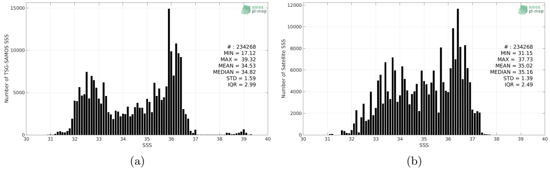
Figure 2: Histograms of SSS from TSG-SAMOS (a) and Aquarius-L2-JPL-V5 (b) considering all match-up pairs per bins of 0.1 over the Gulf Stream Pi-MEP region and for the full satellite product period.
