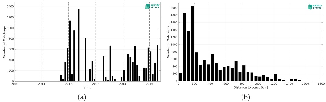
Figure 2: Number of match-ups between TSG (LEGOS-DM) and Aquarius SSS L2 CAP v5 (JPL) SSS as a function of time (a) and as function of the distance to coast (b) over the Gulf Stream Pi-MEP region and for the full satellite product period.
