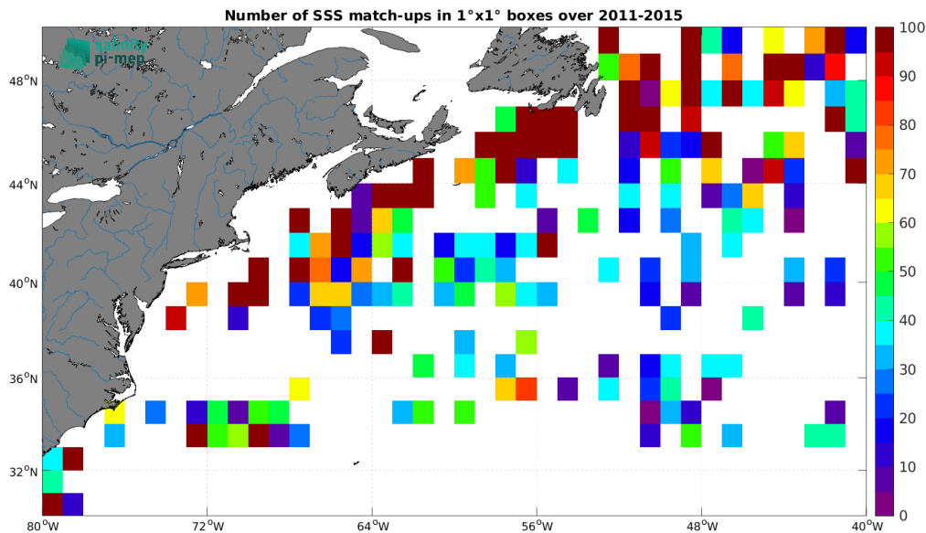
Figure 5: Number of SSS match-ups between TSG (LEGOS-DM) SSS and the Aquarius SSS L2 CAP v5 (JPL) SSS product for the Gulf Stream Pi-MEP region over 1^\circ \times 1^\circ boxes and for the full satellite product period.
