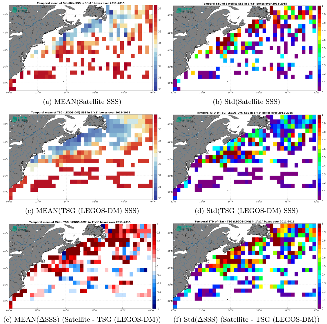
Figure 7: Temporal mean (left) and Std (right) of SSS from Aquarius SSS L2 CAP v5 (JPL) (top), TSG (LEGOS-DM) (middle), and of \Delta SSS (Satellite - TSG (LEGOS-DM)). Only match-up pairs are used to generate these maps.
