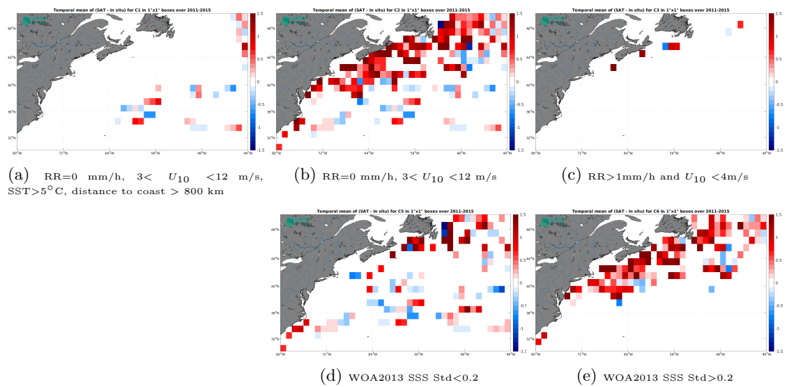
Figure 14: Temporal mean gridded over spatial boxes of size 1^\circ \times 1^\circ of \Delta SSS (Aquarius SSS L2 CAP v5 (JPL) - TSG (LEGOS-DM)) for 5 different subdatasets corresponding to: RR=0 mm/h, 3 < U_{10} < 12 m/s, SST > 5°C, distance to coast > 800 km (a), RR=0 mm/h, 3 < U_{10} < 12 m/s (b), RR > 1mm/h and U_{10} < 4 m/s (c), WOA2013 SSS Std < 0.2 (d), WOA2013 SSS Std > 0.2 (e).
