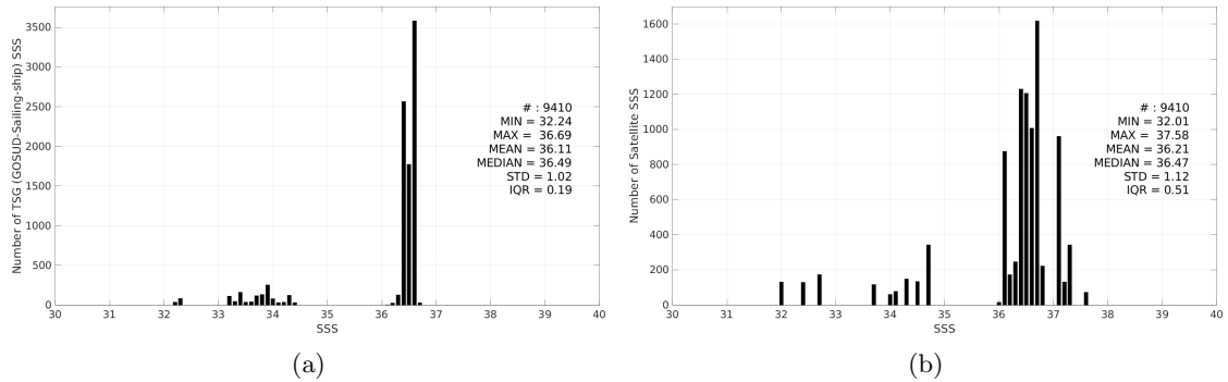
Figure 3: Histograms of SSS from TSG (GOSUD-Sailing-ship) (a) and Aquarius SSS L2 CAP v5 (JPL) (b) considering all match-up pairs per bins of 0.1 over the Gulf Stream Pi-MEP region and for the full satellite product period.
