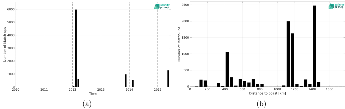
Figure 2: Number of match-ups between TSG (GOSUD-Sailing-ship) and Aquarius SSS L2 CAP v5 (JPL) SSS as a function of time (a) and as function of the distance to coast (b) over the Gulf Stream Pi-MEP region and for the full satellite product period.
