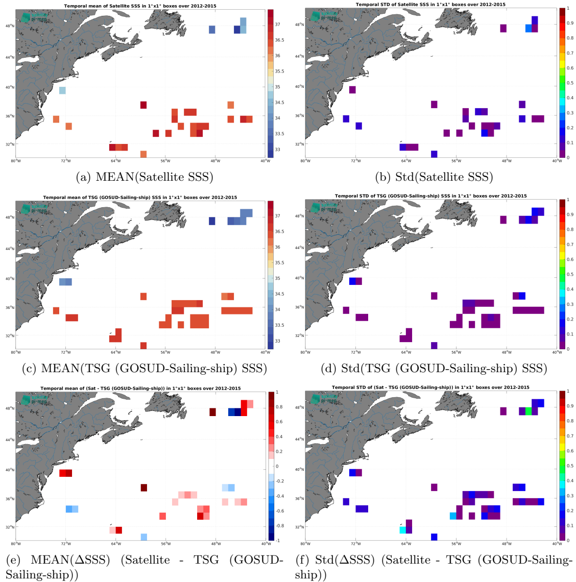
Figure 7: Temporal mean (left) and Std (right) of SSS from Aquarius SSS L2 CAP v5 (JPL) (top), TSG (GOSUD-Sailing-ship) (middle), and of \Delta SSS (Satellite - TSG (GOSUD-Sailing-ship)). Only match-up pairs are used to generate these maps.
