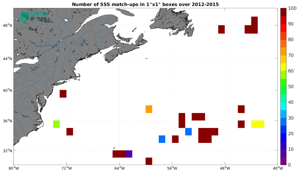
Figure 5: Number of SSS match-ups between TSG (GOSUD-Sailing-ship) SSS and the Aquarius SSS L2 CAP v5 (JPL) SSS product for the Gulf Stream Pi-MEP region over 1^\circ \times 1^\circ boxes and for the full satellite product period.
