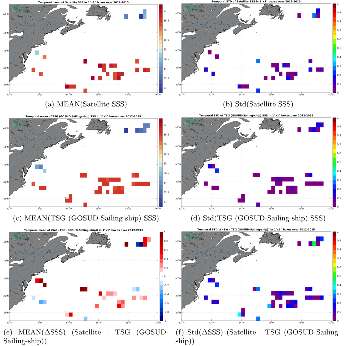
Figure 6: Temporal mean (left) and Std (right) of SSS from Aquarius SSS L2 CAP v5 (JPL) (top), TSG (GOSUD-Sailing-ship) (middle), and of \Delta SSS (Satellite - TSG (GOSUD-Sailing-ship)). Only match-up pairs are used to generate these maps.
