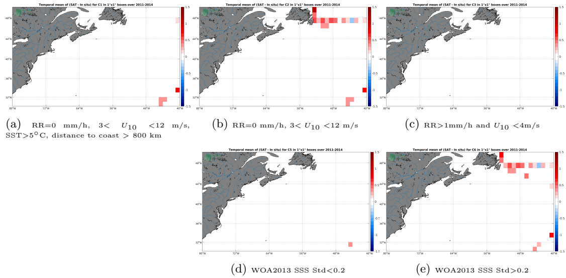
Figure 12: Temporal mean gridded over spatial boxes of size 1^\circ \times 1^\circ of \Delta\text{SSS} (Aquarius SSS L2 CAP v5 (JPL) - TSG (GOSUD-Research-vessel)) for 5 different subdatasets corresponding to:RR=0 mm/h, 3 < U_{10} < 12 m/s, SST>5°C, distance to coast > 800 km (a), RR=0 mm/h, 3 < U_{10} < 12 m/s (b), RR>1mm/h and U_{10} < 4 m/s (c), WOA2013 SSS Std<0.2 (d), WOA2013 SSS Std>0.2 (e).
