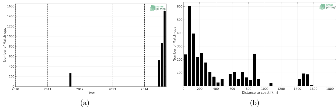
Figure 1: Number of match-ups between TSG (GOSUD-Research-vessel) and Aquarius SSS L2 CAP v5 (JPL) SSS as a function of time (a) and as function of the distance to coast (b) over the Gulf Stream Pi-MEP region and for the full satellite period.
