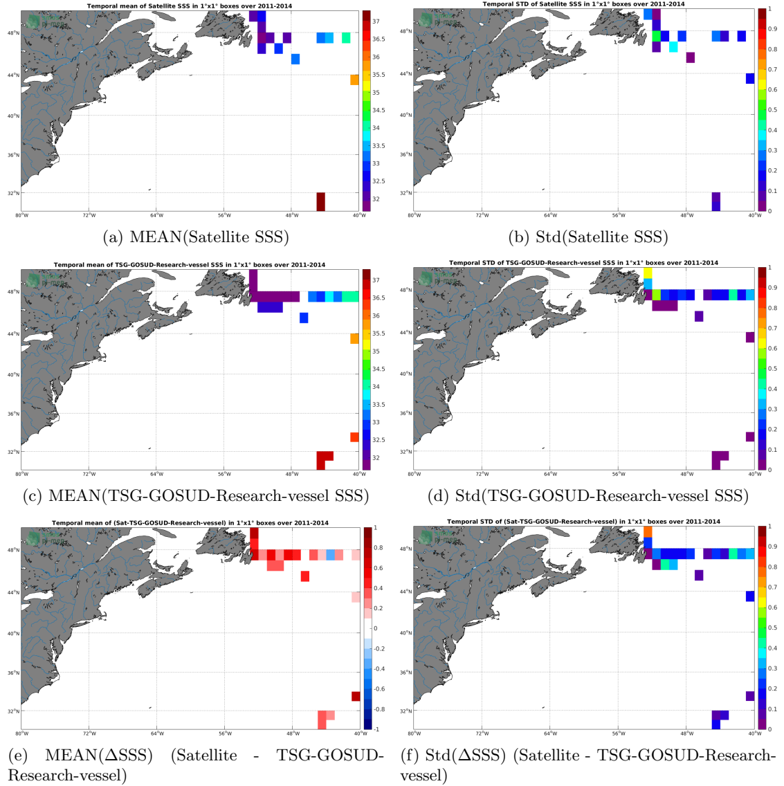
Figure 6: Temporal mean (left) and Std (right) of SSS from Aquarius-L2-JPL-V5 (top), TSG-GOSUD-Research-vessel (middle), and of \Delta\text{SSS} (Satellite - TSG-GOSUD-Research-vessel). Only match-up pairs are used to generate these maps.
