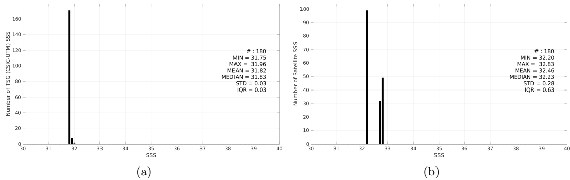
Figure 3: Histograms of SSS from TSG (CSIC-UTM) (a) and Aquarius SSS L2 CAP v5 (JPL) (b) considering all match-up pairs per bins of 0.1 over the Gulf Stream Pi-MEP region and for the full satellite product period.
