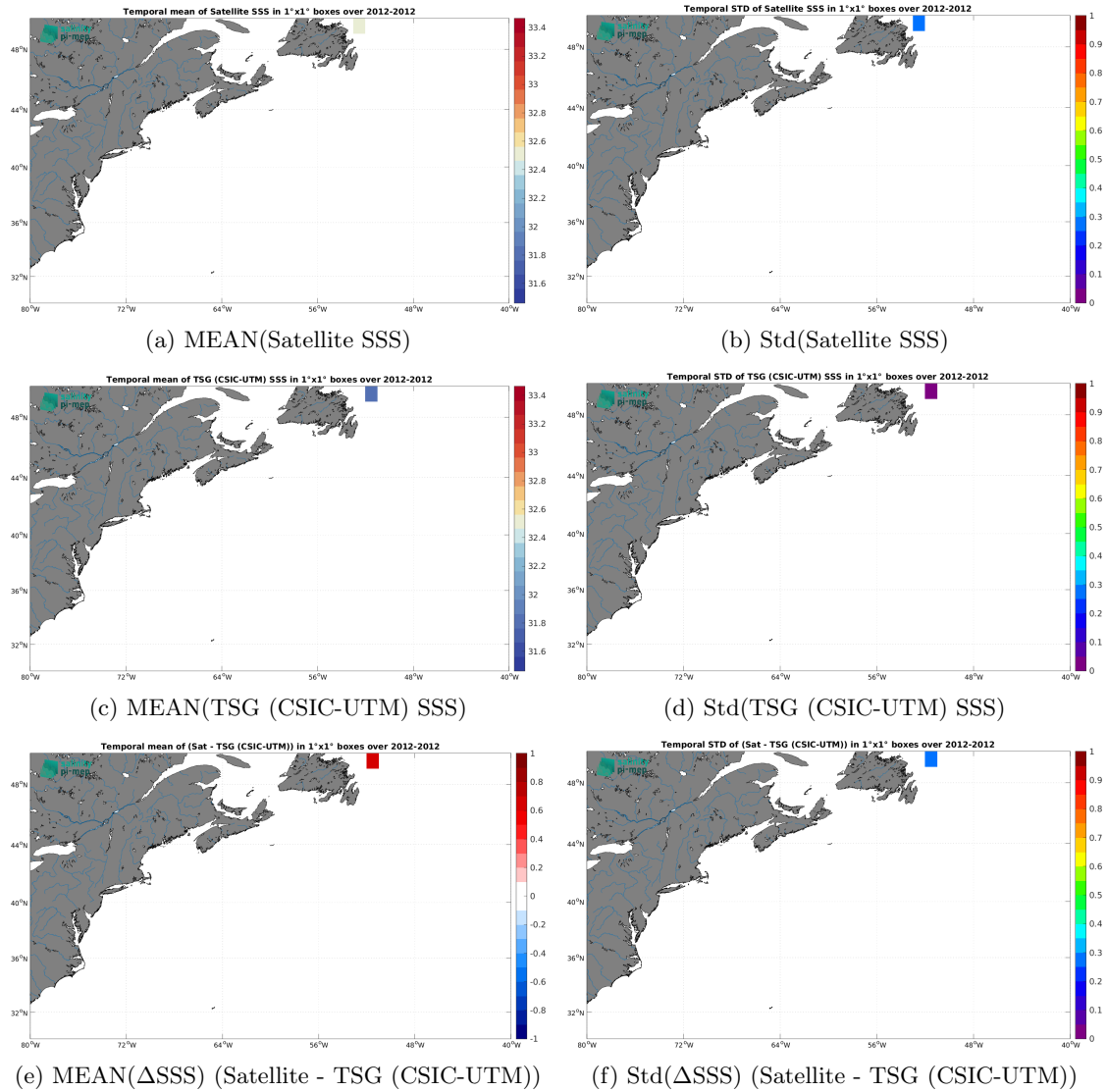
Figure 7: Temporal mean (left) and Std (right) of SSS from Aquarius SSS L2 CAP v5 (JPL) (top), TSG (CSIC-UTM) (middle), and of \Delta SSS (Satellite - TSG (CSIC-UTM)). Only match-up pairs are used to generate these maps.
