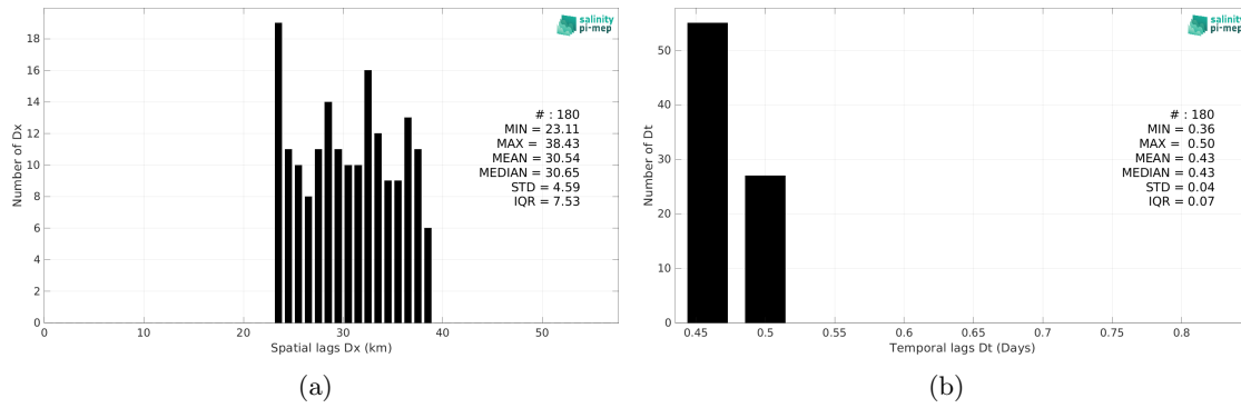
Figure 6: Histograms of the spatial (a) and temporal (b) lags between the location/time of the TSG (CSIC-UTM) measurement and the date of the corresponding Aquarius SSS L2 CAP v5 (JPL) SSS pixel.
