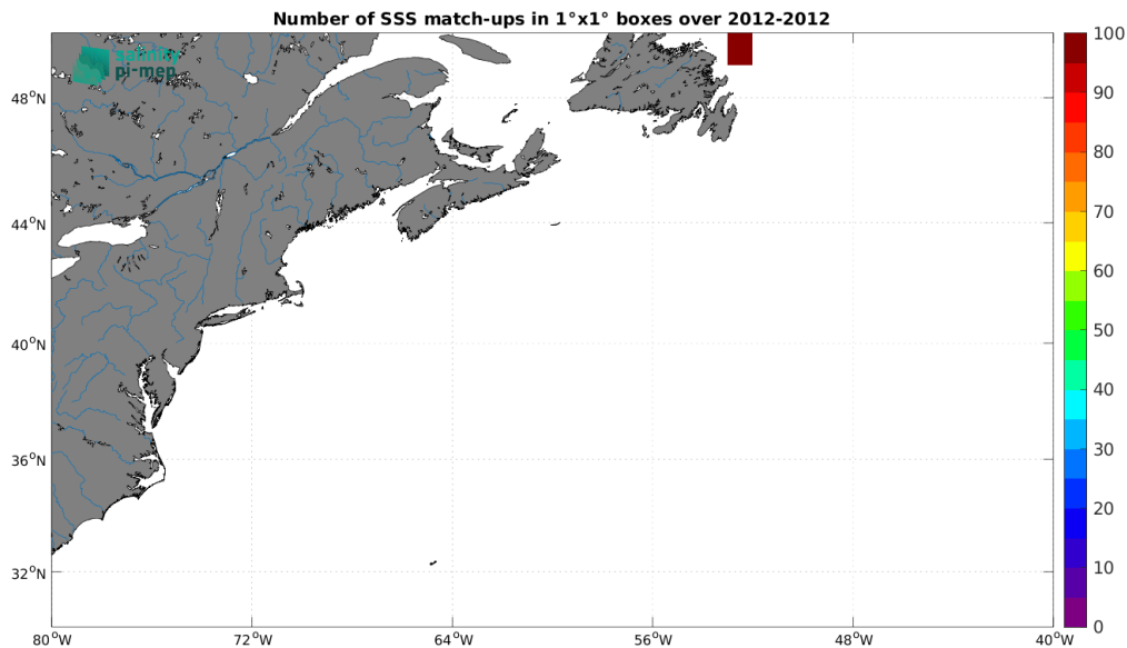
Figure 5: Number of SSS match-ups between TSG (CSIC-UTM) SSS and the Aquarius SSS L2 CAP v5 (JPL) SSS product for the Gulf Stream Pi-MEP region over 1^\circ \times 1^\circ boxes and for the full satellite product period.
