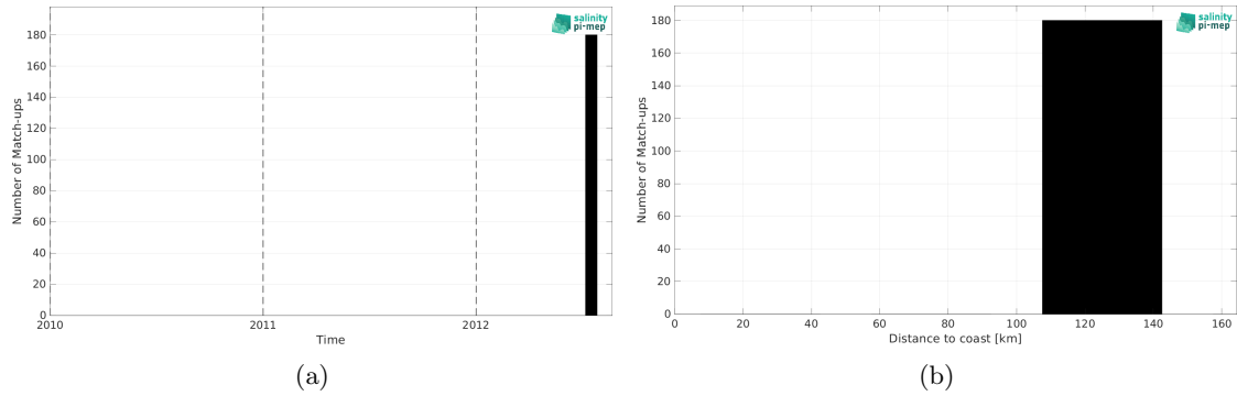
Figure 2: Number of match-ups between TSG (CSIC-UTM) and Aquarius SSS L2 CAP v5 (JPL) SSS as a function of time (a) and as function of the distance to coast (b) over the Gulf Stream Pi-MEP region and for the full satellite product period.
