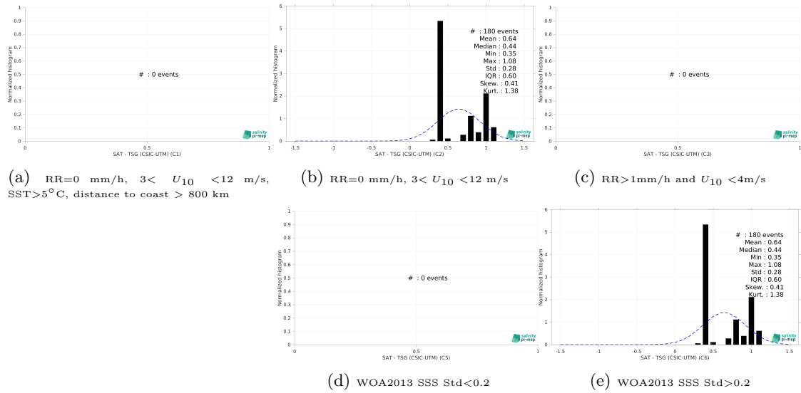
Figure 15: Normalized histogram of \Delta\text{SSS} (Aquarius SSS L2 CAP v5 (JPL) - TSG (CSIC-UTM)) for 5 different subdatasets corresponding to: RR=0 mm/h, 3 < U_{10} < 12 m/s, SST > 5^\circ\text{C} , distance to coast > 800 km (a), RR=0 mm/h, 3 < U_{10} < 12 m/s (b), RR > 1\text{mm/h} and U_{10} < 4\text{m/s} (c), WOA2013 SSS Std < 0.2 (d), WOA2013 SSS Std > 0.2 (e).
