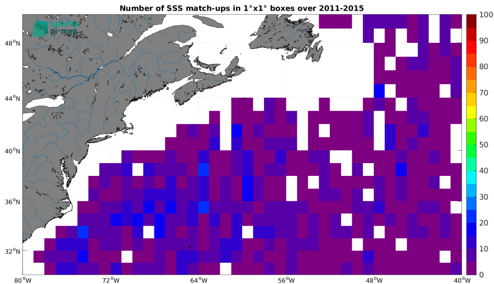
Figure 5: Number of SSS match-ups between Argo SSS and the Aquarius SSS L2 CAP v5 (JPL) SSS product for the Gulf Stream Pi-MEP region over 1^\circ \times 1^\circ boxes and for the full satellite product period.
