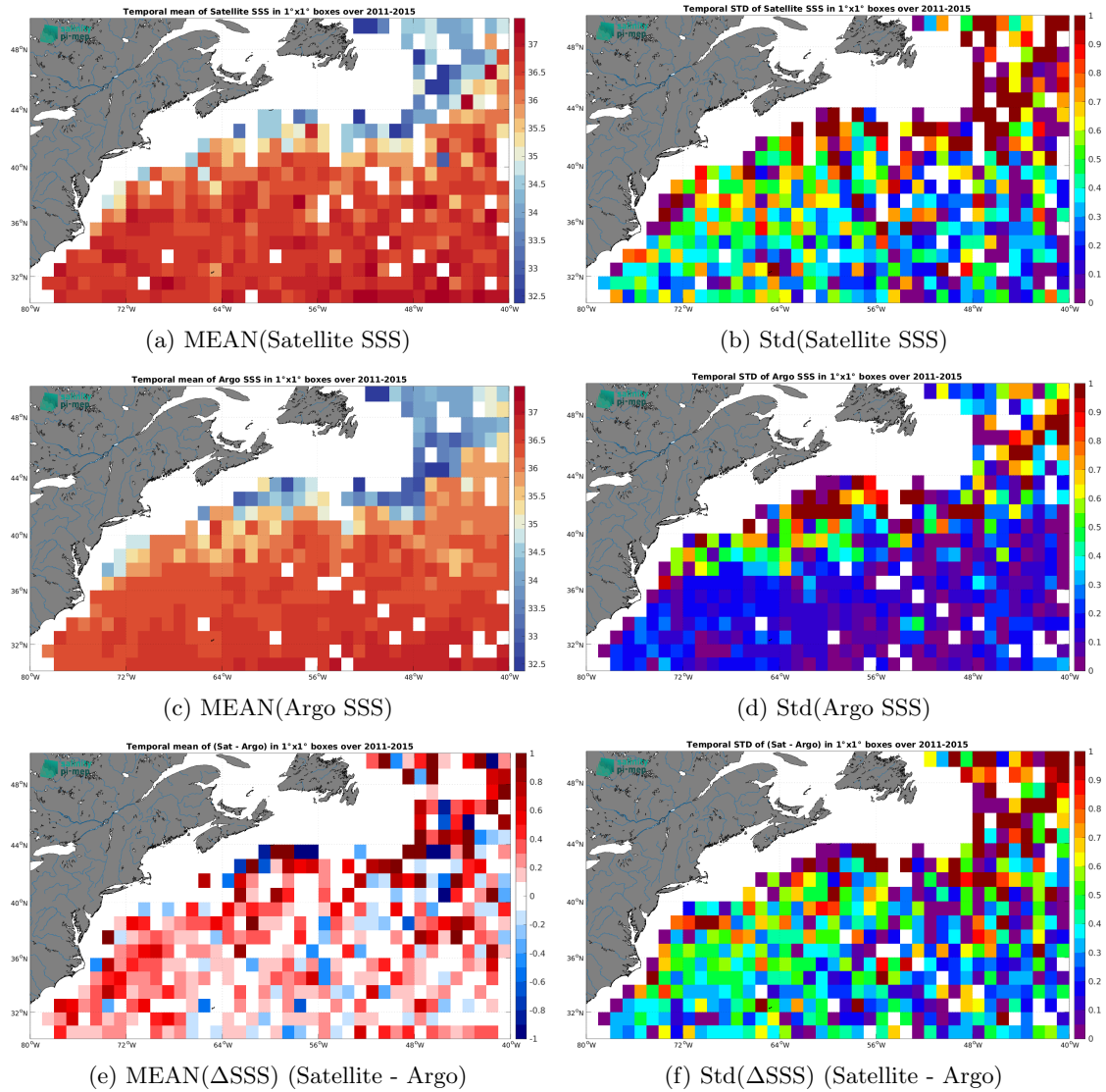
Figure 7: Temporal mean (left) and Std (right) of SSS from Aquarius SSS L2 CAP v5 (JPL) (top), Argo (middle), and of \Delta SSS (Satellite - Argo). Only match-up pairs are used to generate these maps.
