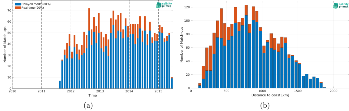
Figure 2: Number of match-ups between Argo and Aquarius SSS L2 CAP v5 (JPL) SSS as a function of time (a) and as function of the distance to coast (b) over the Gulf Stream Pi-MEP region and for the full satellite product period.
