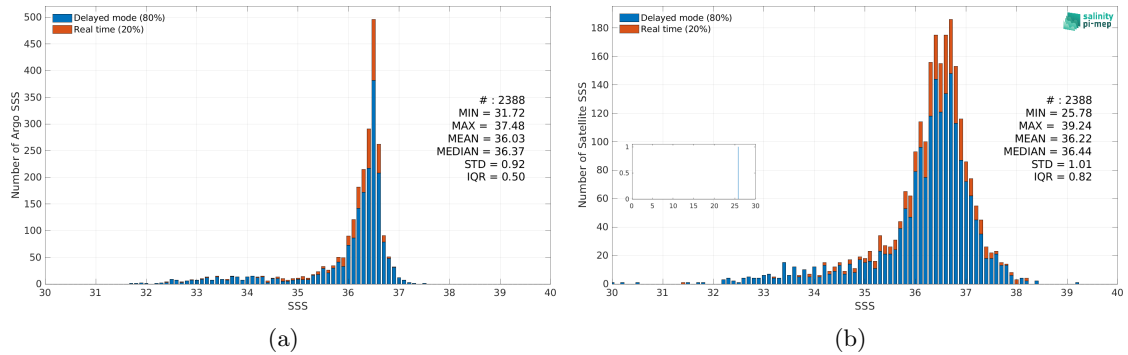
Figure 3: Histograms of SSS from Argo (a) and Aquarius SSS L2 CAP v5 (JPL) (b) considering all match-up pairs per bins of 0.1 over the Gulf Stream Pi-MEP region and for the full satellite product period.
