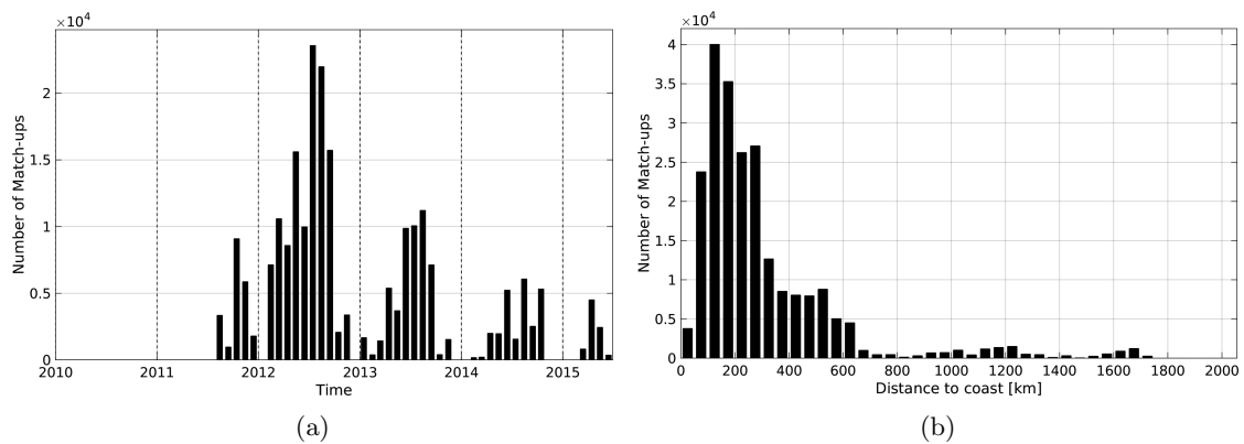
Figure 1: Number of match-ups between TSG-SAMOS and AQUARIUS-L2-JPL-V4 SSS as a function of time (a) and as function of the distance to coast (b) over the Gulf Stream Pi-MEP region and for the full satellite product period.
