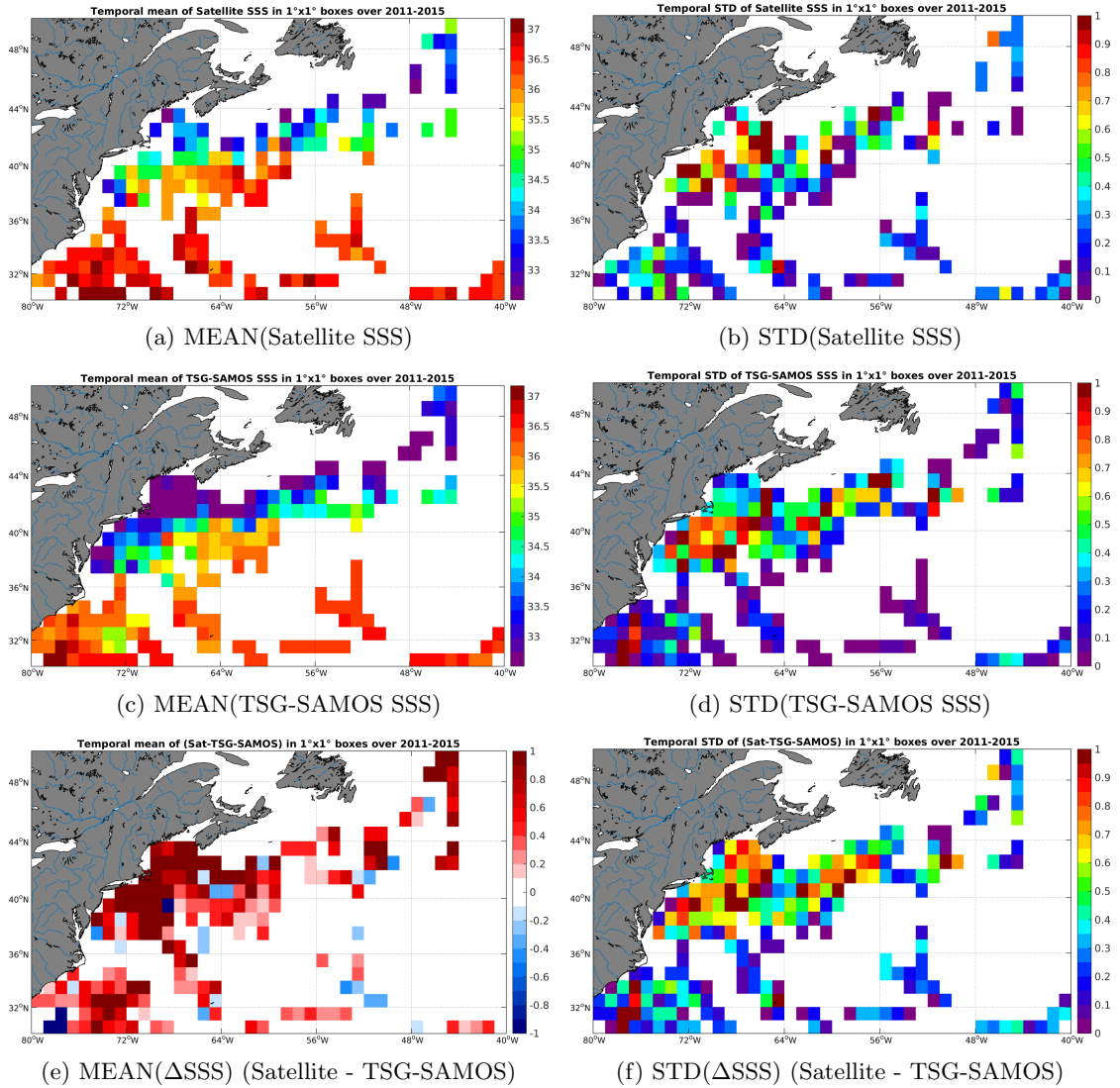
Figure 6: Temporal mean (left) and STD (right) of SSS from AQUARIUS-L2-JPL-V4 (top), TSG-SAMOS (middle), and of \Delta\text{SSS} (Satellite - TSG-SAMOS). Only match-up pairs are used to generate these maps.
