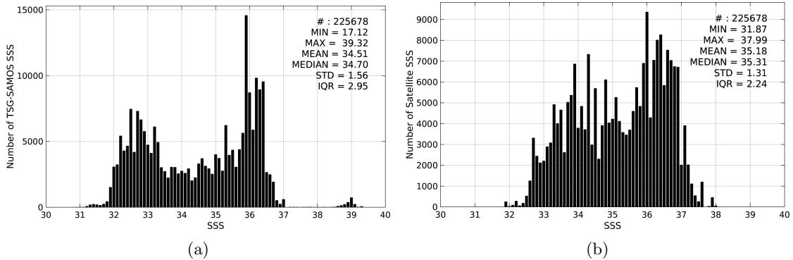
Figure 2: Histograms of SSS from TSG-SAMOS (a) and AQUARIUS-L2-JPL-V4 (b) considering all match-up pairs per bins of 0.1 over the Gulf Stream Pi-MEP region and for the full satellite product period.
