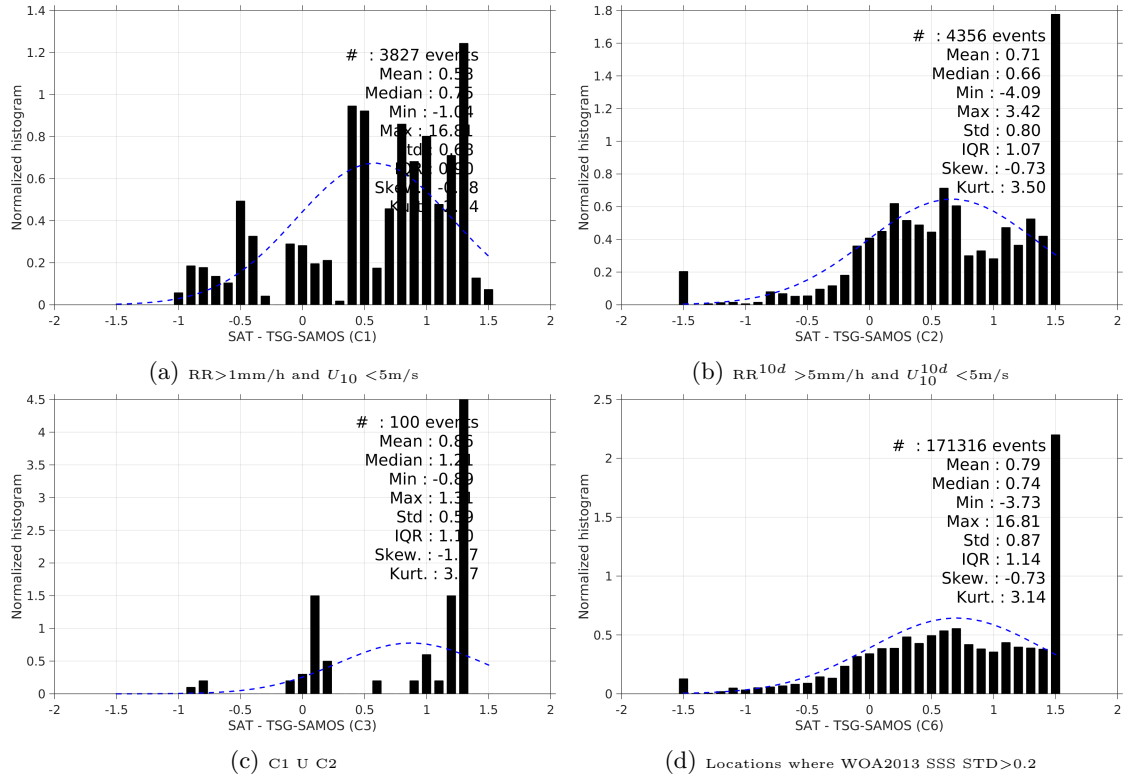
Figure 13: Normalized histogram of \Delta\text{SSS} (AQUARIUS-L2-JPL-V4 - TSG-SAMOS) for 6 different subdatasets corresponding to: RR>1mm/h and U_{10} < 5\text{m/s} (a), RR^{10d} > 5\text{mm/h} and U_{10}^{10d} < 5\text{m/s} (b), C1 U C2 (c), Locations where WOA2013 SSS STD>0.2 (d).
