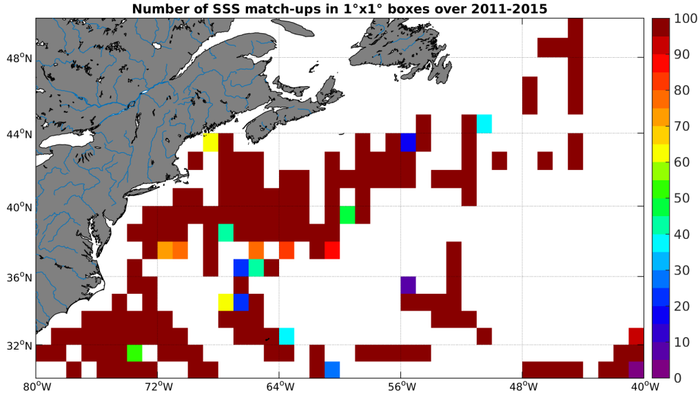
Figure 4: Number of SSS match-ups between TSG-SAMOS SSS and the AQUARIUS-L2-JPL-V4 SSS product for the Gulf Stream Pi-MEP region over 1^\circ \times 1^\circ boxes and for the full satellite product period.
