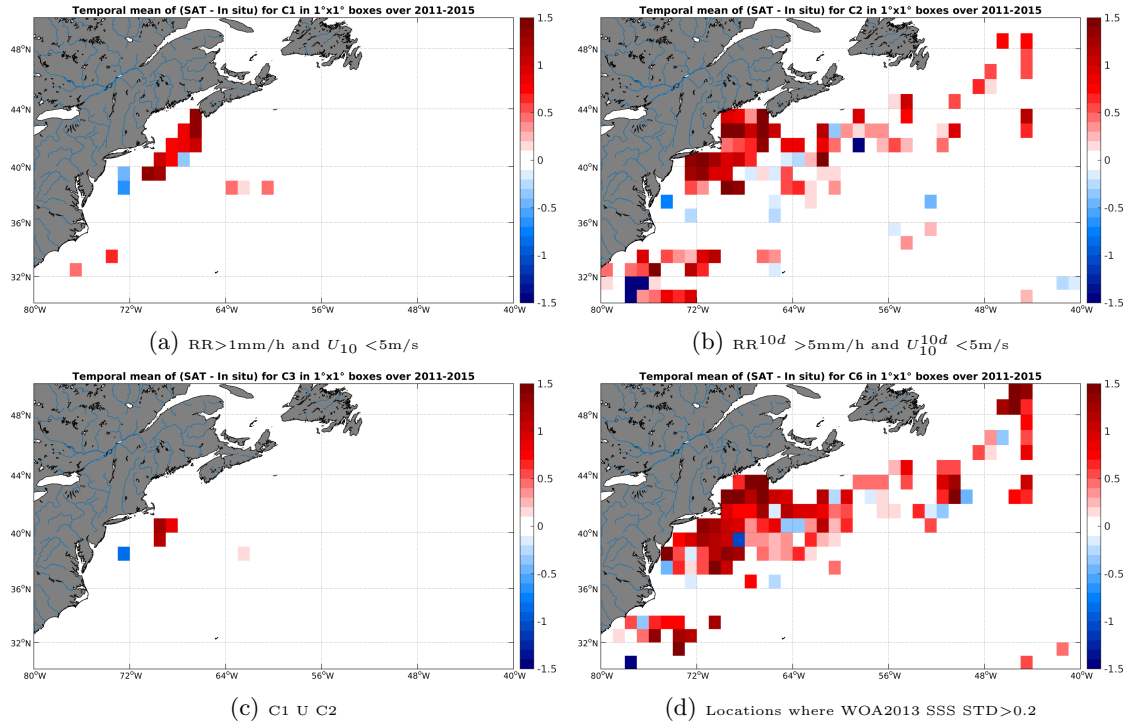
Figure 12: Temporal mean gridded over spatial boxes of size 1^\circ \times 1^\circ of \Delta SSS (AQUARIUS-L2-JPL-V4 - TSG-SAMOS) for 4 different subdatasets corresponding to:RR > 1 mm/h and U_{10} < 5 m/s (a), RR^{10d} > 5 mm/h and U_{10}^{10d} < 5 m/s (b), C1 U C2 (c),Locations where WOA2013 SSS STD > 0.2 (d).
