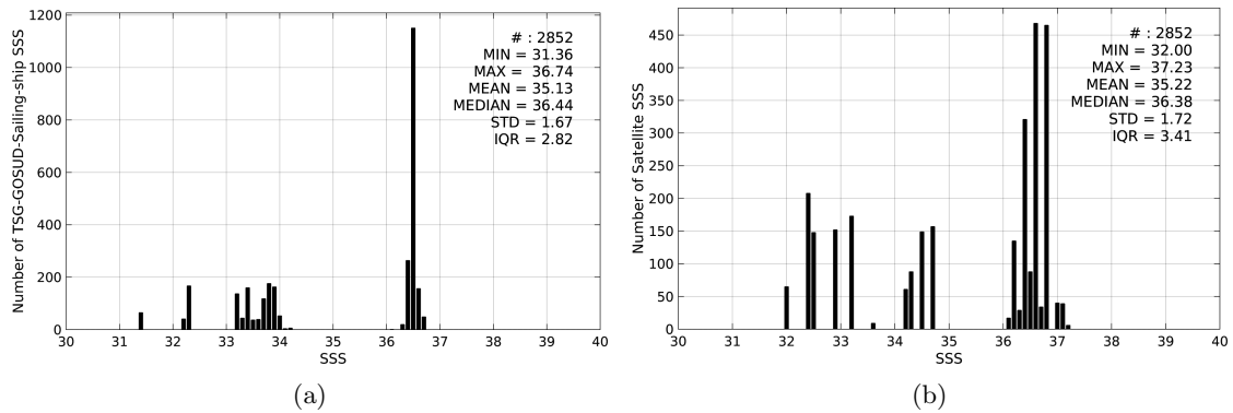
Figure 2: Histograms of SSS from TSG-GOSUD-Sailing-ship (a) and AQUARIUS-L2-JPL-V4 (b) considering all match-up pairs per bins of 0.1 over the Gulf Stream Pi-MEP region and for the full satellite product period.
