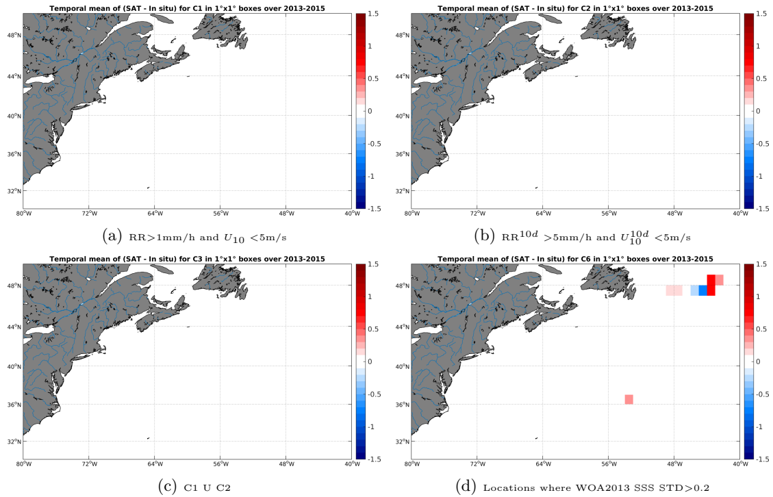
Figure 12: Temporal mean gridded over spatial boxes of size 1°x1° of \Delta SSS (AQUARIUS-L2-JPL-V4 - TSG-GOSUD-Sailing-ship) for 4 different subdatasets corresponding to:RR > 1mm/h and U_{10} < 5\text{m/s} (a), RR^{10d} > 5\text{mm/h} and U_{10}^{10d} < 5\text{m/s} (b), C1 U C2 (c),Locations where WOA2013 SSS STD > 0.2 (d).
