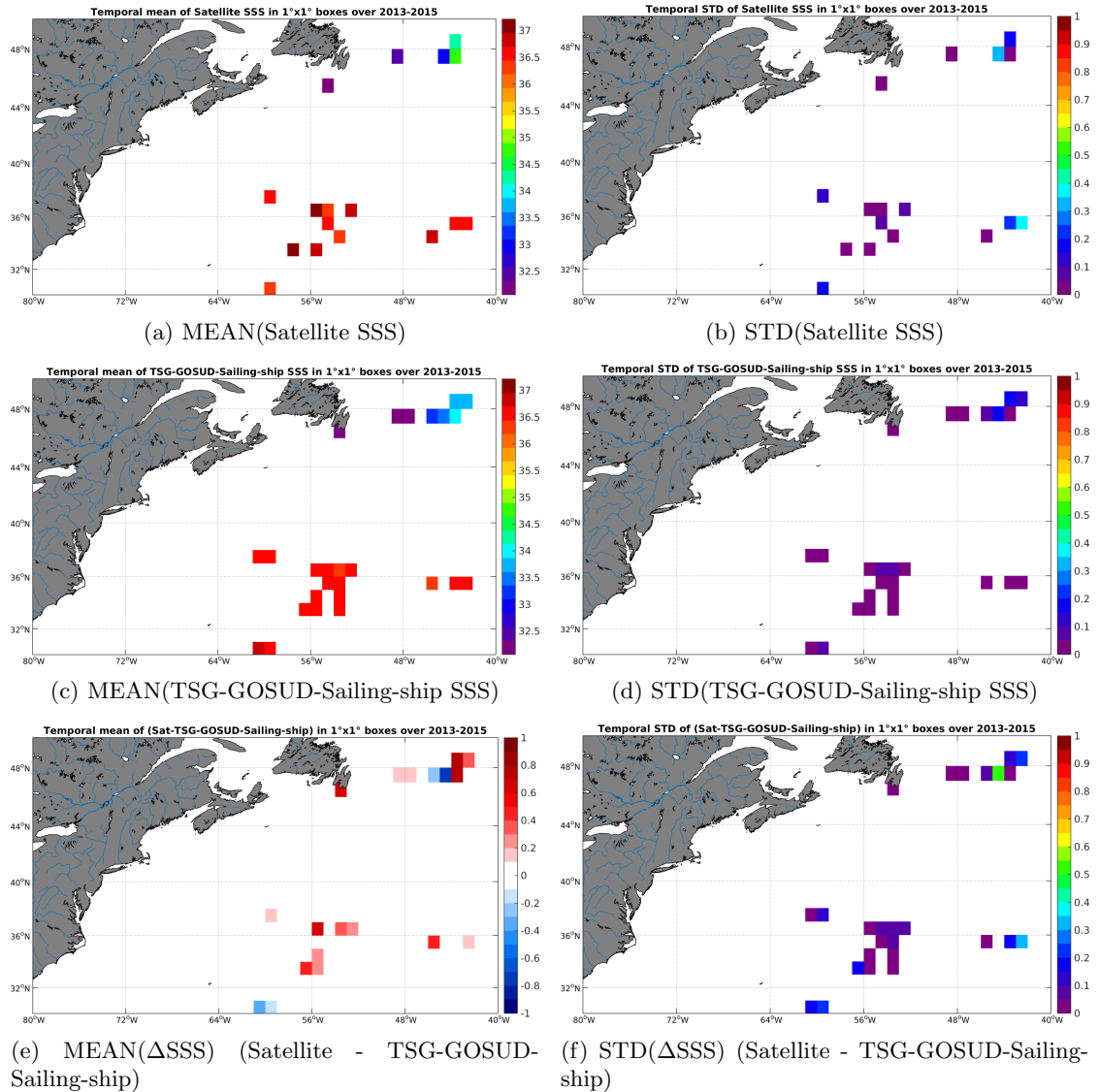
Figure 6: Temporal mean (left) and STD (right) of SSS from AQUARIUS-L2-JPL-V4 (top), TSG-GOSUD-Sailing-ship (middle), and of \Delta SSS (Satellite - TSG-GOSUD-Sailing-ship). Only match-up pairs are used to generate these maps.
