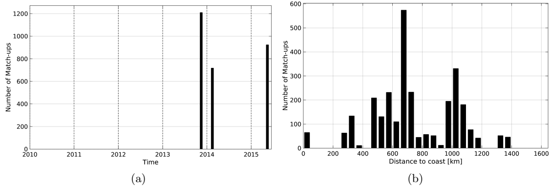
Figure 1: Number of match-ups between TSG-GOSUD-Sailing-ship and AQUARIUS-L2-JPL-V4 SSS as a function of time (a) and as function of the distance to coast (b) over the Gulf Stream Pi-MEP region and for the full satellite product period.
