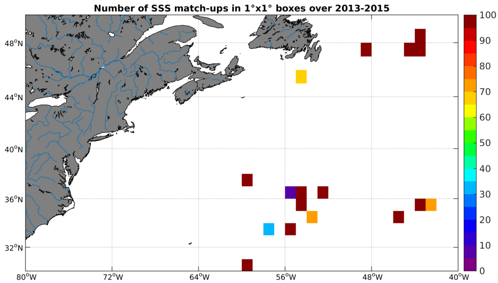
Figure 4: Number of SSS match-ups between TSG-GOSUD-Sailing-ship SSS and the AQUARIUS-L2-JPL-V4 SSS product for the Gulf Stream Pi-MEP region over 1^\circ \times 1^\circ boxes and for the full satellite product period.
