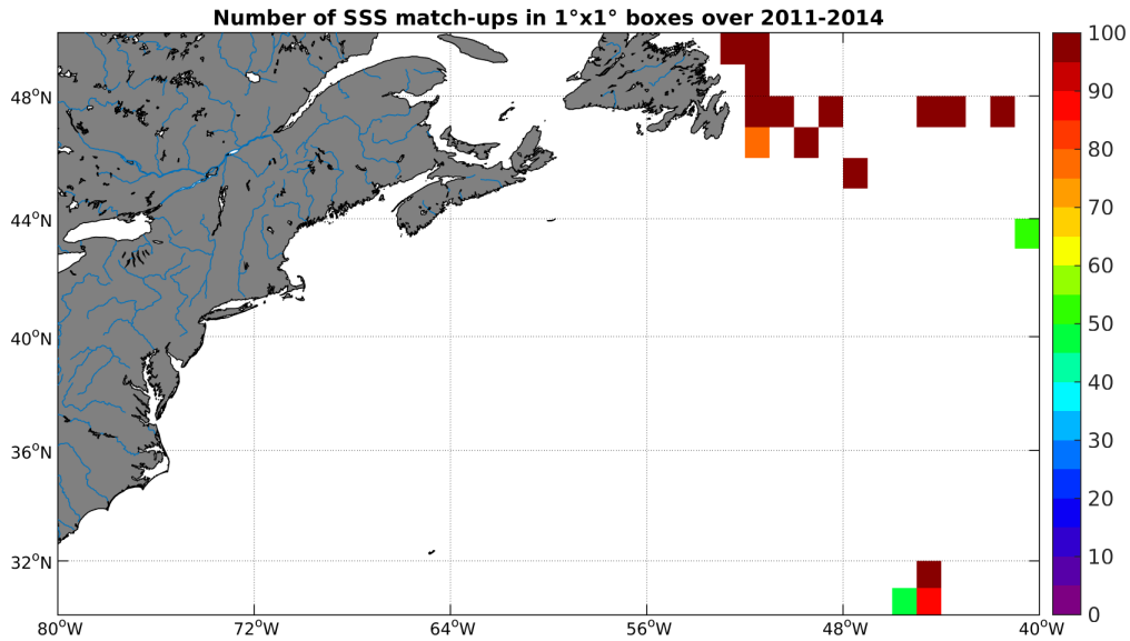
Figure 4: Number of SSS match-ups between TSG-GOSUD-Research-vessel SSS and the AQUARIUS-L2-JPL-V4 SSS product for the Gulf Stream Pi-MEP region over 1°x1° boxes and for the full satellite product period.
