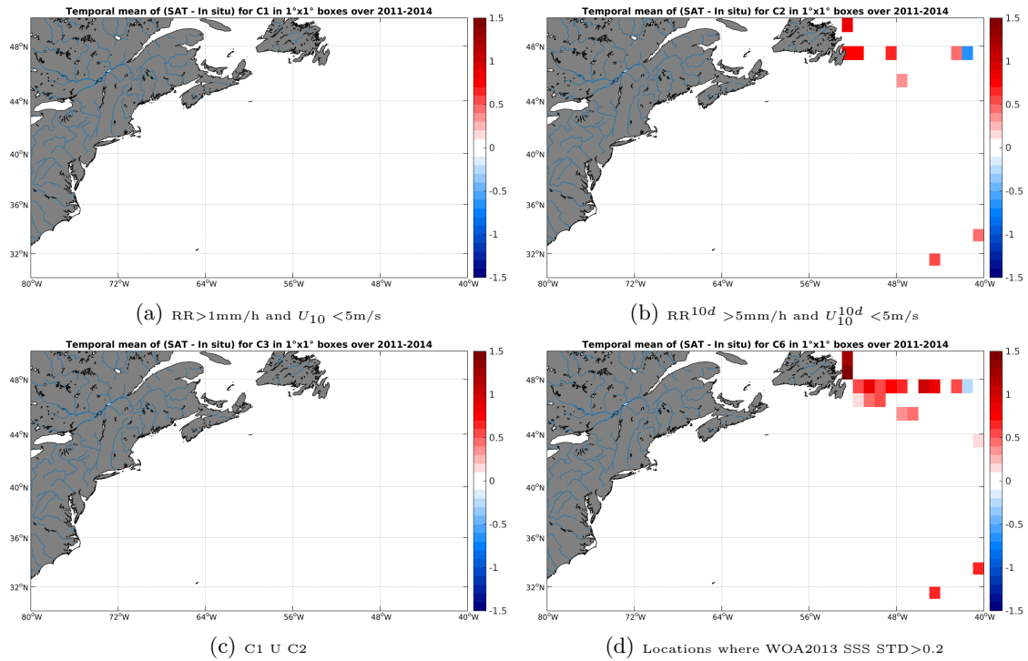
Figure 12: Temporal mean gridded over spatial boxes of size 1^\circ \times 1^\circ of \Delta SSS (AQUARIUS-L2-JPL-V4 - TSG-GOSUD-Research-vessel) for 4 different subdatasets corresponding to: RR > 1mm/h and U_{10} < 5\text{m/s} (a), RR^{10d} > 5\text{mm/h} and U_{10}^{10d} < 5\text{m/s} (b), C1 U C2 (c), Locations where WOA2013 SSS STD > 0.2 (d).
