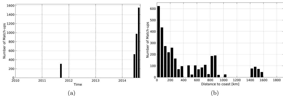
Figure 1: Number of match-ups between TSG-GOSUD-Research-vessel and AQUARIUS-L2-JPL-V4 SSS as a function of time (a) and as function of the distance to coast (b) over the Gulf Stream Pi-MEP region and for the full satellite product period.
