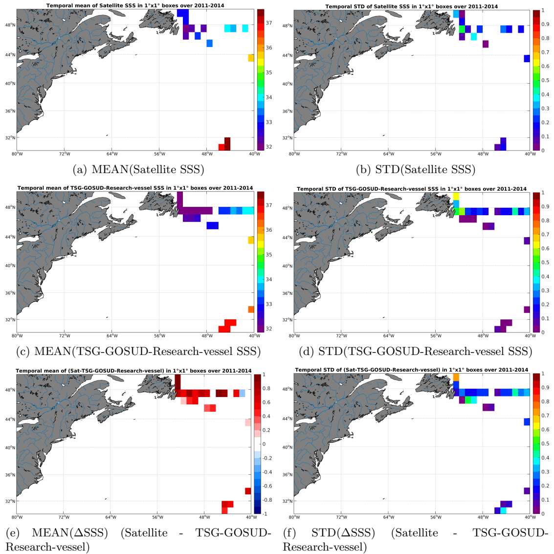
Figure 6: Temporal mean (left) and STD (right) of SSS from AQUARIUS-L2-JPL-V4 (top), TSG-GOSUD-Research-vessel (middle), and of \Delta SSS (Satellite - TSG-GOSUD-Research-vessel). Only match-up pairs are used to generate these maps.
