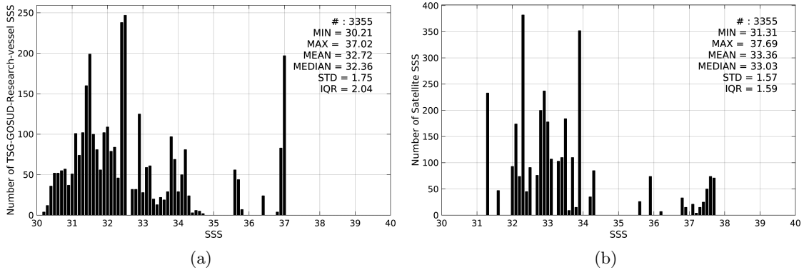
Figure 2: Histograms of SSS from TSG-GOSUD-Research-vessel (a) and AQUARIUS-L2-JPL-V4 (b) considering all match-up pairs per bins of 0.1 over the Gulf Stream Pi-MEP region and for the full satellite product period.
