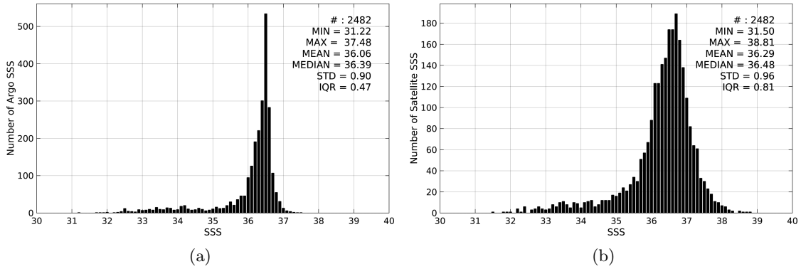
Figure 2: Histograms of SSS from Argo (a) and AQUARIUS-L2-JPL-V4 (b) considering all match-up pairs per bins of 0.1 over the Gulf Stream Pi-MEP region and for the full satellite product period.
