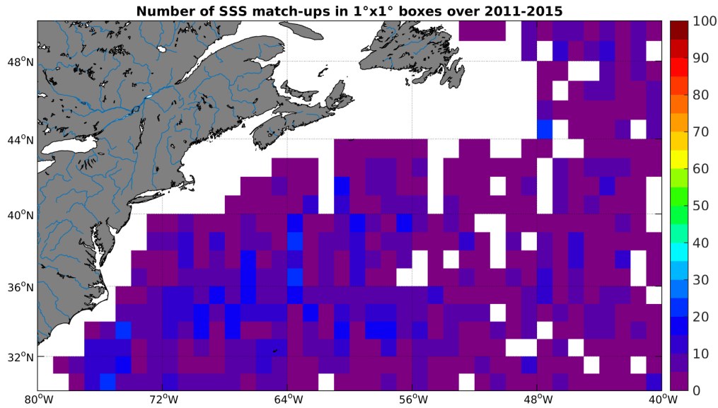
Figure 4: Number of SSS match-ups between Argo SSS and the AQUARIUS-L2-JPL-V4 SSS product for the Gulf Stream Pi-MEP region over 1^\circ \times 1^\circ boxes and for the full satellite product period.
