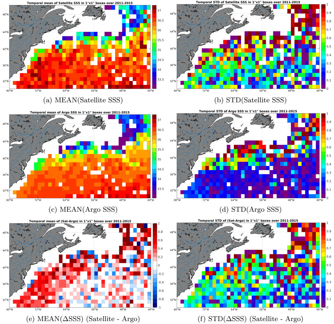
Figure 6: Temporal mean (left) and STD (right) of SSS from AQUARIUS-L2-JPL-V4 (top), Argo (middle), and of \Delta\text{SSS}(\text{Satellite} - \text{Argo}) . Only match-up pairs are used to generate these maps.
