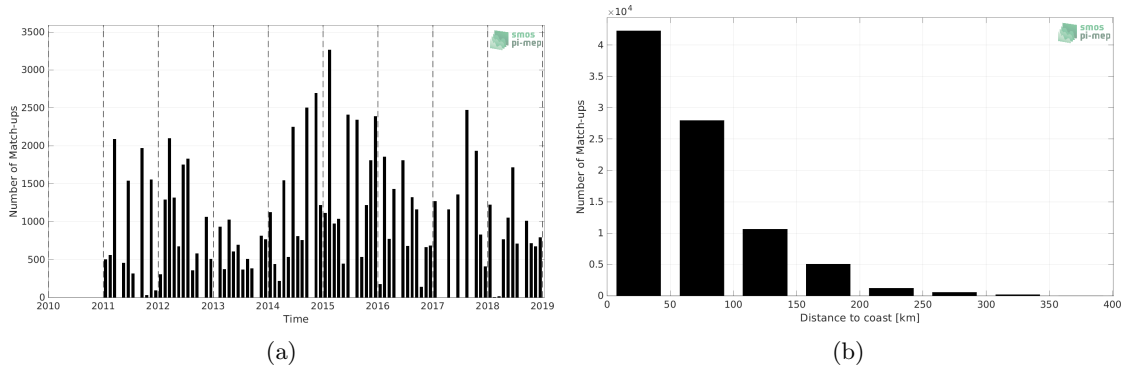
Figure 1: Number of match-ups between TSG (LEGOS-DM) and SMOS and SMAP SSS L4 OI v1 - 7 Days (LOPS) SSS as a function of time (a) and as function of the distance to coast (b) over the Mediterranean Sea Pi-MEP region and for the full satellite product period.
