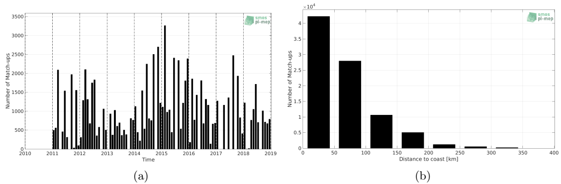
Figure 1: Number of match-ups between TSG (LEGOS-DM) and SMOS and SMAP SSS L4 OI v1 - 7 Days (LOPS) SSS as a function of time (a) and as function of the distance to coast (b) over the Mediterranean Sea Pi-MEP region and for the full satellite product period.
