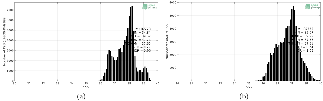
Figure 2: Histograms of SSS from TSG (LEGOS-DM) (a) and SMOS and SMAP SSS L4 OI v1 - 7 Days (LOPS) (b) considering all match-up pairs per bins of 0.1 over the Mediterranean Sea Pi-MEP region and for the full satellite product period.
