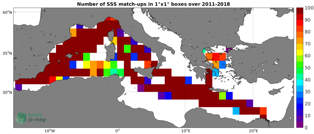
Figure 4: Number of SSS match-ups between TSG (LEGOS-DM) SSS and the SMOS and SMAP SSS L4 OI v1 - 7 Days (LOPS) SSS product for the Mediterranean Sea Pi-MEP region over 1^\circ \times 1^\circ boxes and for the full satellite product period.
