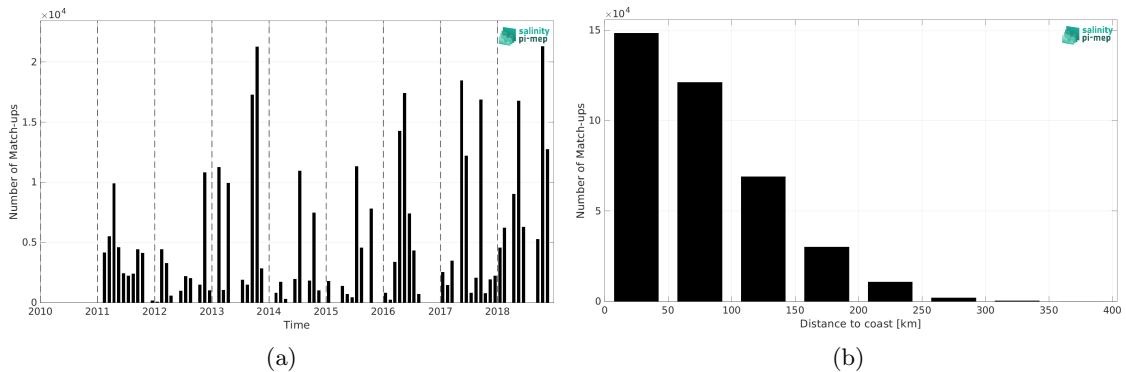
Figure 1: Number of match-ups between TSG (GOSUD-Research-vessel) and SMOS and SMAP SSS L4 OI v1 - 7 Days (LOPS) SSS as a function of time (a) and as function of the distance to coast (b) over the Mediterranean Sea Pi-MEP region and for the full satellite product period.
