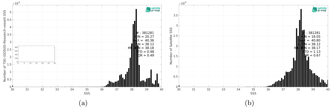
Figure 2: Histograms of SSS from TSG (GOSUD-Research-vessel) (a) and SMOS and SMAP SSS L4 OI v1 - 7 Days (LOPS) (b) considering all match-up pairs per bins of 0.1 over the Mediterranean Sea Pi-MEP region and for the full satellite product period.
