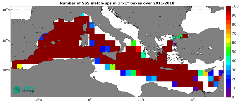
Figure 4: Number of SSS match-ups between TSG (GOSUD-Research-vessel) SSS and the SMOS and SMAP SSS L4 OI v1 - 7 Days (LOPS) SSS product for the Mediterranean Sea Pi-MEP region over 1^\circ \times 1^\circ boxes and for the full satellite product period.
