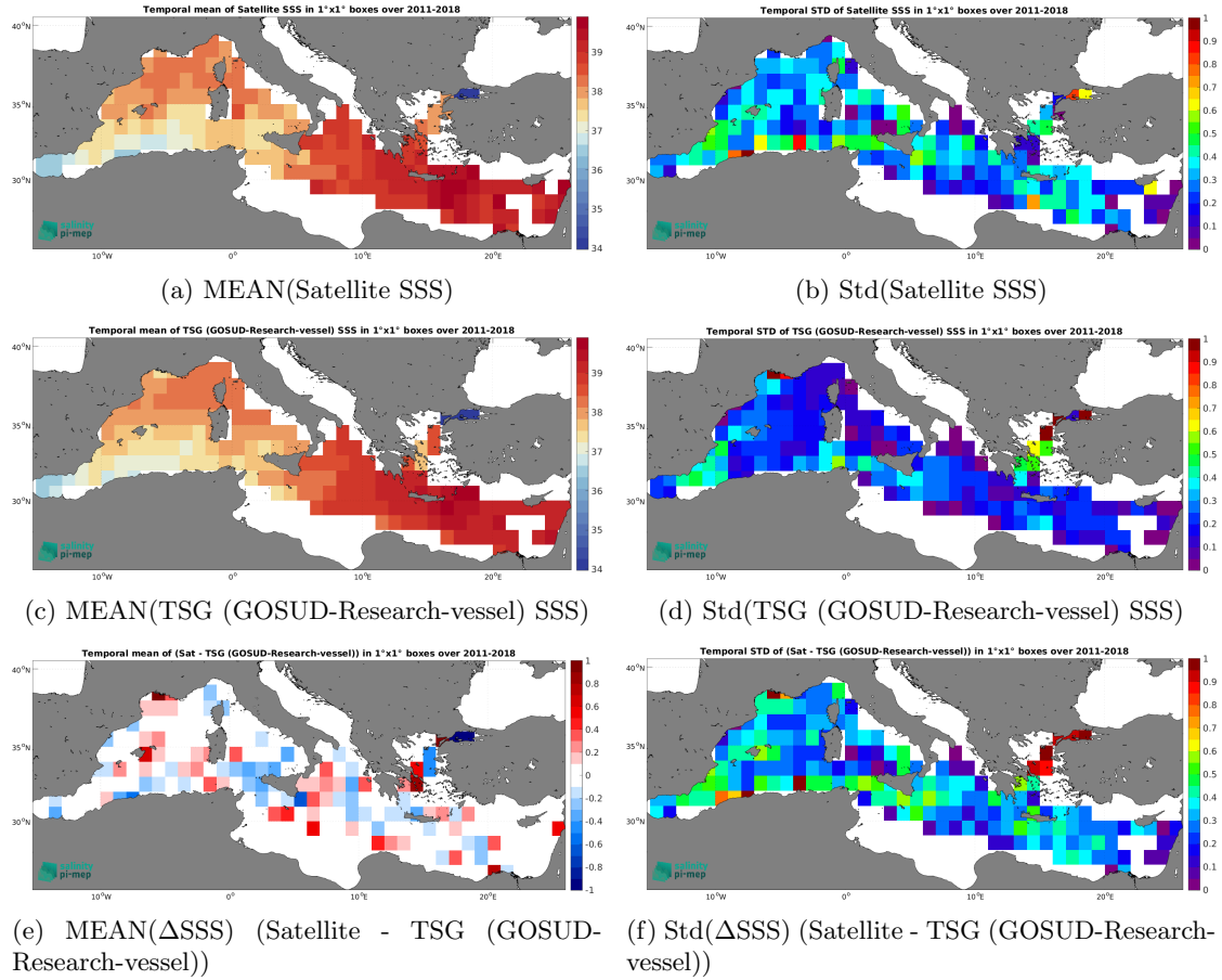
Figure 6: Temporal mean (left) and Std (right) of SSS from SMOS and SMAP SSS L4 OI v1 - 7 Days (LOPS) (top), TSG (GOSUD-Research-vessel) (middle), and of \Delta\text{SSS} (Satellite - TSG (GOSUD-Research-vessel)). Only match-up pairs are used to generate these maps.
