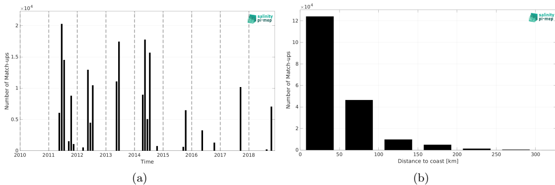
Figure 1: Number of match-ups between TSG (CSIC-UTM) and SMOS and SMAP SSS L4 OI v1 - 7 Days (LOPS) SSS as a function of time (a) and as function of the distance to coast (b) over the Mediterranean Sea Pi-MEP region and for the full satellite product period.
