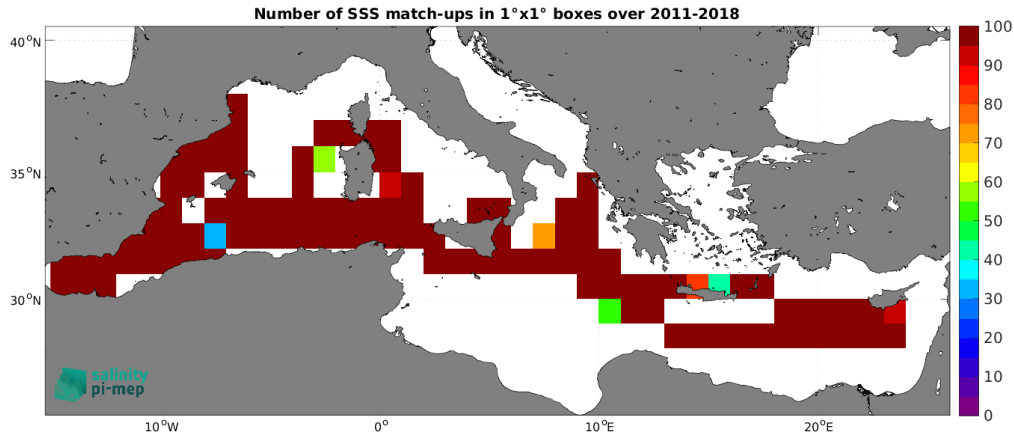
Figure 4: Number of SSS match-ups between TSG (CSIC-UTM) SSS and the SMOS and SMAP SSS L4 OI v1 - 7 Days (LOPS) SSS product for the Mediterranean Sea Pi-MEP region over 1^\circ \times 1^\circ boxes and for the full satellite product period.
