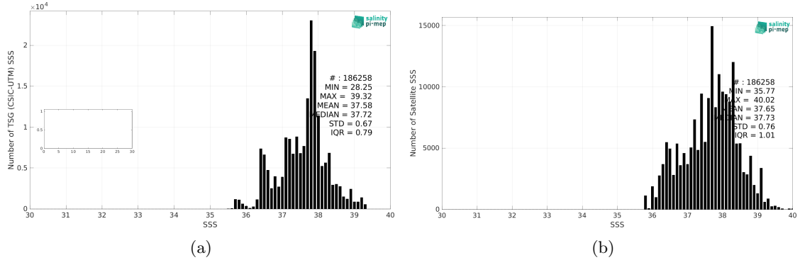
Figure 2: Histograms of SSS from TSG (CSIC-UTM) (a) and SMOS and SMAP SSS L4 OI v1 - 7 Days (LOPS) (b) considering all match-up pairs per bins of 0.1 over the Mediterranean Sea Pi-MEP region and for the full satellite product period.
