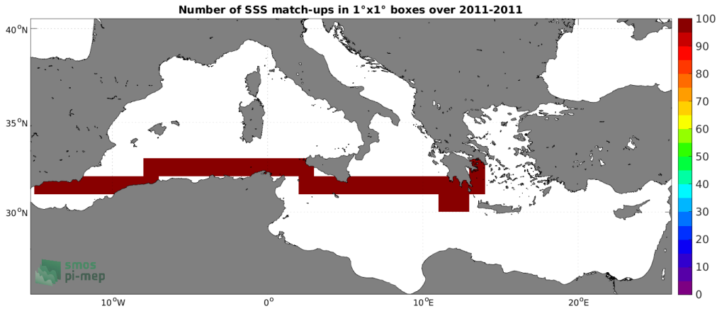
Figure 4: Number of SSS match-ups between TSG (SAMOS) SSS and the SMOS SSS L4 v1 - Weekly (CMEMS-CNR) SSS product for the Mediterranean Sea Pi-MEP region over 1^\circ \times 1^\circ boxes and for the full satellite product period.
