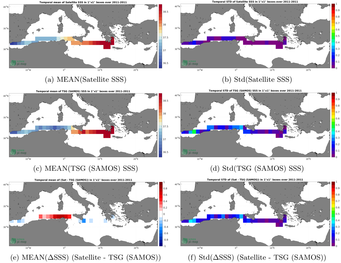
Figure 6: Temporal mean (left) and Std (right) of SSS from SMOS SSS L4 v1 - Weekly (CMEMS-CNR) (top), TSG (SAMOS) (middle), and of \Delta SSS (Satellite - TSG (SAMOS)). Only match-up pairs are used to generate these maps.
