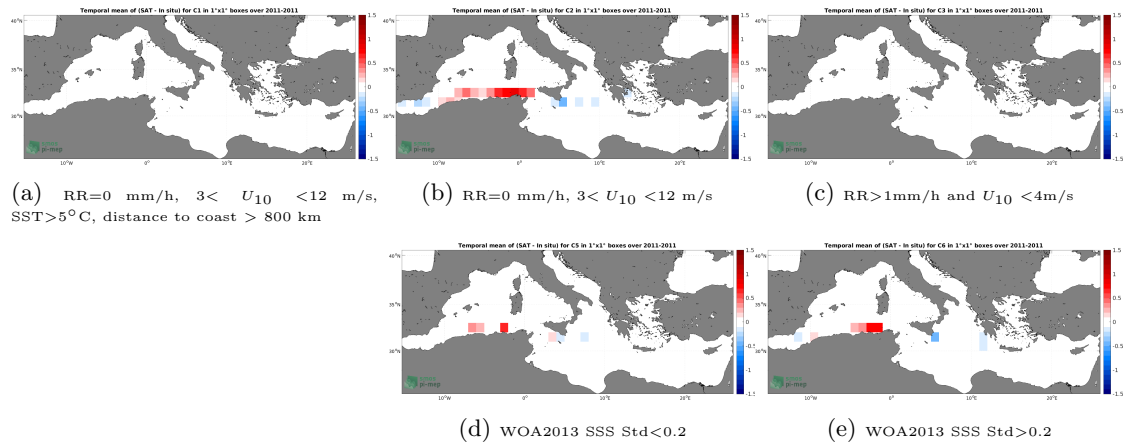
Figure 12: Temporal mean gridded over spatial boxes of size 1^{\circ}\times 1^{\circ} of \Delta\text{SSS} (SMOS SSS L4 v1 - Weekly (CMEMS-CNR) - TSG (SAMOS)) for 5 different subdatasets corresponding to:RR=0 mm/h, 3 < U_{10} < 12 m/s, SST >5^{\circ}\text{C} , distance to coast > 800 km (a), RR=0 mm/h, 3 < U_{10} < 12 m/s (b), RR >1 mm/h and U_{10} < 4 m/s (c), WOA2013 SSS Std <0.2 (d), WOA2013 SSS Std >0.2 (e).
