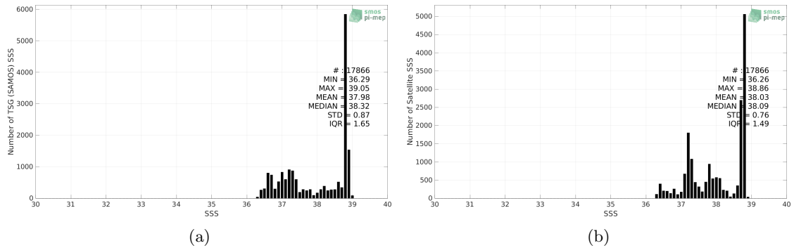
Figure 2: Histograms of SSS from TSG (SAMOS) (a) and SMOS SSS L4 v1 - Weekly (CMEMS-CNR) (b) considering all match-up pairs per bins of 0.1 over the Mediterranean Sea Pi-MEP region and for the full satellite product period.
