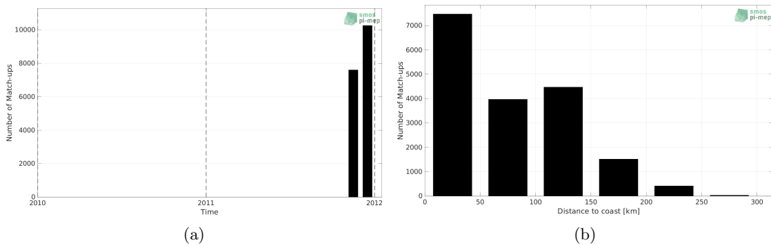
Figure 1: Number of match-ups between TSG (SAMOS) and SMOS SSS L4 v1 - Weekly (CMEMS-CNR) SSS as a function of time (a) and as function of the distance to coast (b) over the Mediterranean Sea Pi-MEP region and for the full satellite product period.
