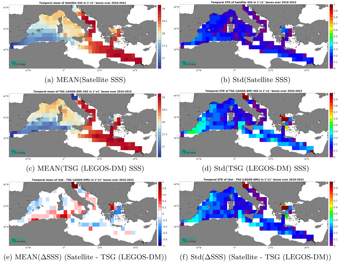
Figure 6: Temporal mean (left) and Std (right) of SSS from SMOS SSS L4 v1 - Weekly (CMEMS-CNR) (top), TSG (LEGOS-DM) (middle), and of \Delta\text{SSS} (Satellite - TSG (LEGOS-DM)). Only match-up pairs are used to generate these maps.
