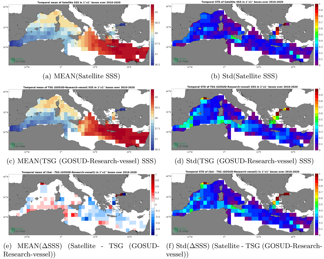
Figure 6: Temporal mean (left) and Std (right) of SSS from SMOS SSS L4 v1 - Weekly (CMEMS-CNR) (top), TSG (GOSUD-Research-vessel) (middle), and of \Delta SSS (Satellite - TSG (GOSUD-Research-vessel)). Only match-up pairs are used to generate these maps.
