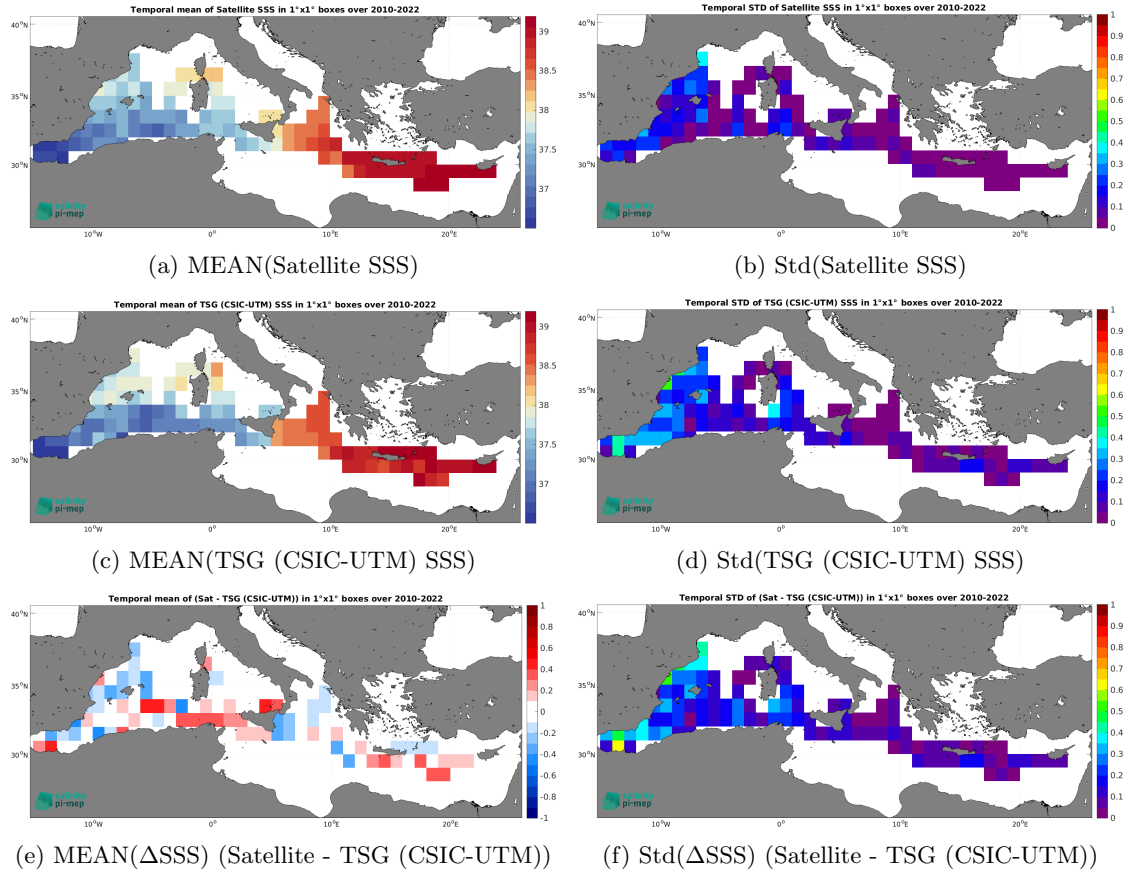
Figure 6: Temporal mean (left) and Std (right) of SSS from SMOS SSS L4 v1 - Weekly (CMEMS-CNR) (top), TSG (CSIC-UTM) (middle), and of \Delta\text{SSS} (Satellite - TSG (CSIC-UTM)). Only match-up pairs are used to generate these maps.
