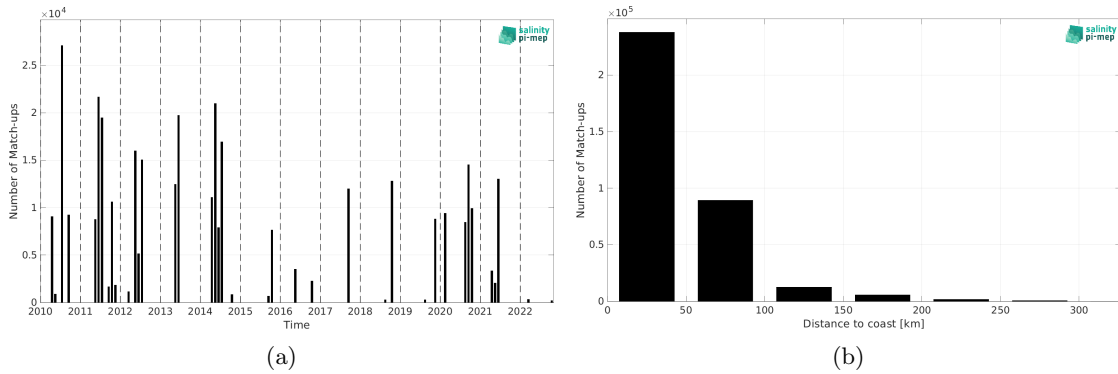
Figure 1: Number of match-ups between TSG (CSIC-UTM) and SMOS SSS L4 v1 - Weekly (CMEMS-CNR) SSS as a function of time (a) and as function of the distance to coast (b) over the Mediterranean Sea Pi-MEP region and for the full satellite product period.
