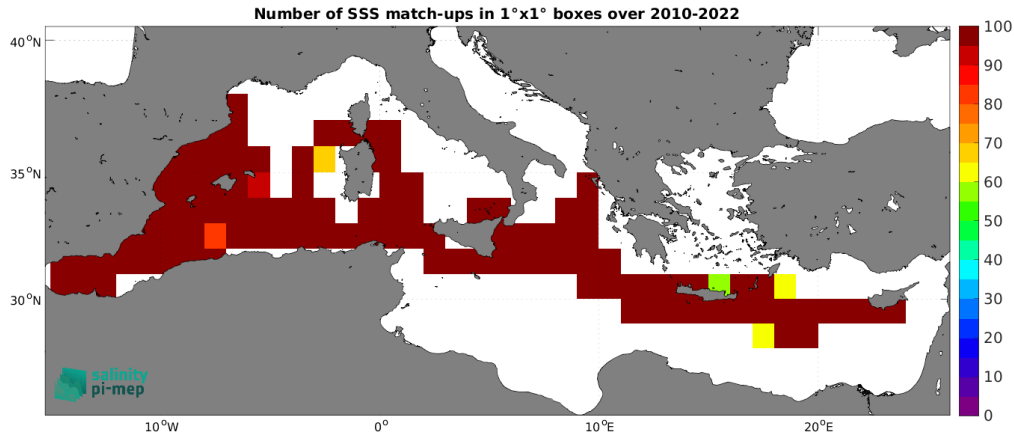
Figure 4: Number of SSS match-ups between TSG (CSIC-UTM) SSS and the SMOS SSS L4 v1 - Weekly (CMEMS-CNR) SSS product for the Mediterranean Sea Pi-MEP region over 1^\circ \times 1^\circ boxes and for the full satellite product period.
