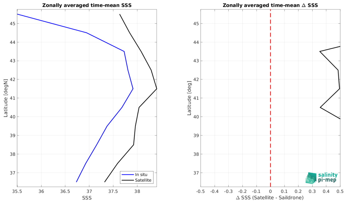
Figure 8: Left panel: Zonal mean SSS from SMOS SSS L4 v1 - Weekly (CMEMS-CNR) satellite product (black) and from Sairdron (blue). Right panel: Zonal mean of \Delta SSS (Satellite - Sairdron) for all the collected Pi-MEP match-up pairs estimated over the full satellite product period.
