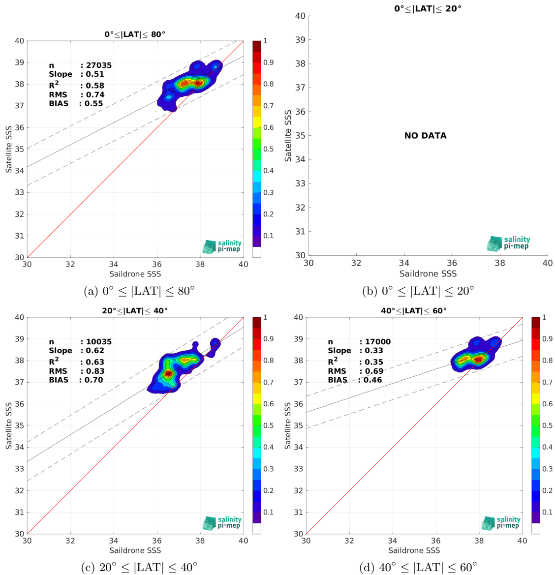
Figure 9: Contour maps of the concentration of SMOS SSS L4 v1 - Weekly (CMEMS-CNR) SSS (y-axis) versus Saildrone SSS (x-axis) at match-up pairs for different latitude bands. For each plot, the red line shows x=y . The black thin and dashed lines indicate a linear fit through the data cloud and the \pm 95\% confidence levels, respectively. The number match-up pairs n , the slope and R^2 coefficient of the linear fit, the root mean square (RMS) and the mean bias between satellite and in situ data are indicated for each latitude band in each plots.
