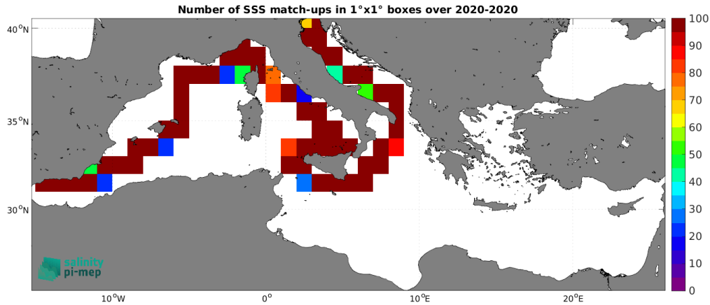
Figure 4: Number of SSS match-ups between Saildrone SSS and the SMOS SSS L4 v1 - Weekly (CMEMS-CNR) SSS product for the Mediterranean Sea Pi-MEP region over 1^\circ \times 1^\circ boxes and for the full satellite product period.
