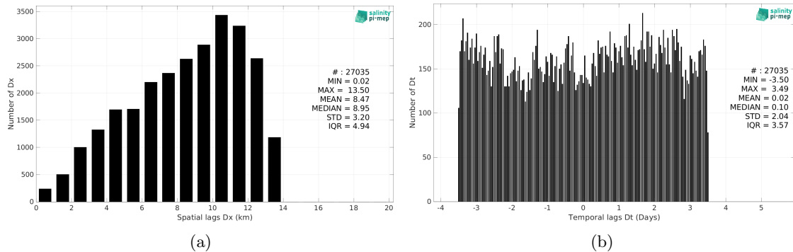
Figure 5: Histograms of the spatial (a) and temporal (b) lags between the location/time of the Saildrone measurement and the date of the corresponding SMOS SSS L4 v1 - Weekly (CMEMS-CNR) SSS pixel.
