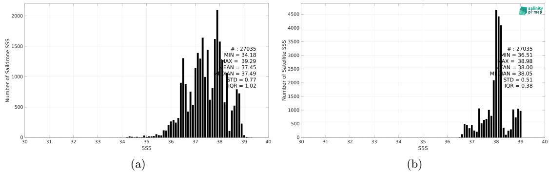
Figure 2: Histograms of SSS from Saildrone (a) and SMOS SSS L4 v1 - Weekly (CMEMS-CNR) (b) considering all match-up pairs per bins of 0.1 over the Mediterranean Sea Pi-MEP region and for the full satellite product period.
