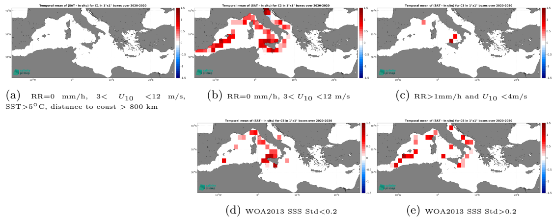
Figure 12: Temporal mean gridded over spatial boxes of size 1^\circ \times 1^\circ of \Delta SSS (SMOS SSS L4 v1 - Weekly (CMEMS-CNR) - Saildrone) for 5 different subdatasets corresponding to:RR=0 mm/h, 3 < U_{10} < 12 m/s, SST >5^\circ\text{C} , distance to coast > 800 km (a), RR=0 mm/h, 3 < U_{10} < 12 m/s (b), RR >1 mm/h and U_{10} < 4 m/s (c), WOA2013 SSS Std <0.2 (d), WOA2013 SSS Std >0.2 (e).
