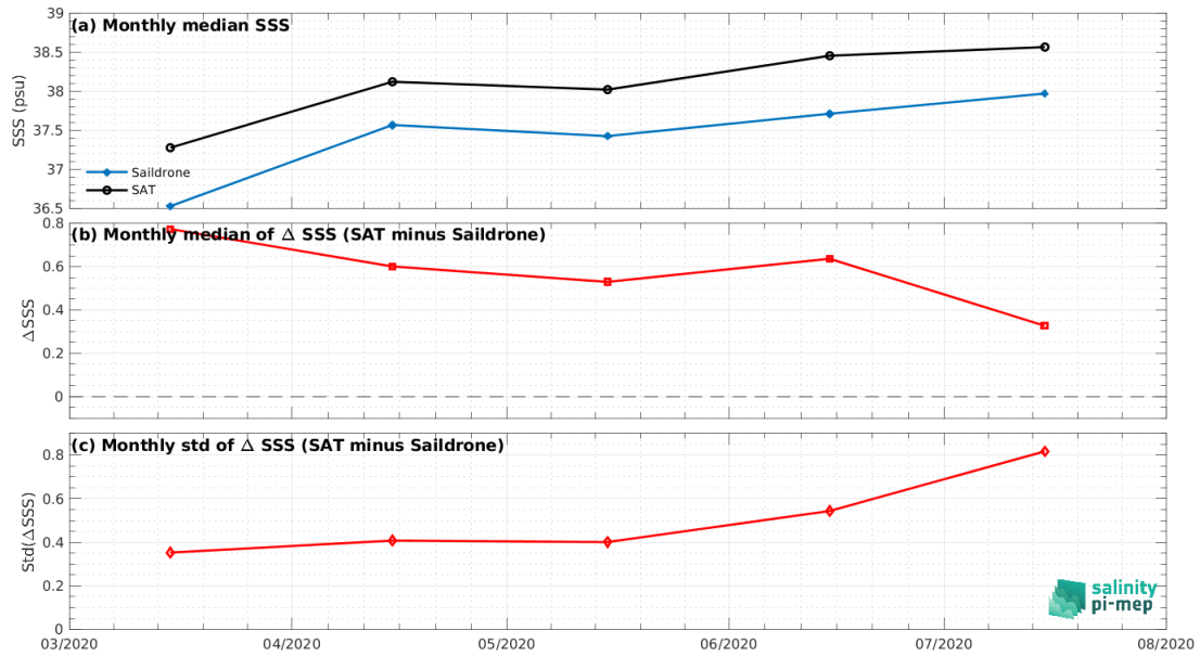
Figure 7: Time series of the monthly median SSS (top), median of \Delta SSS (Satellite - Saildrone) and Std of \Delta SSS (Satellite - Saildrone) over the Mediterranean Sea Pi-MEP region considering all match-ups collected by the Pi-MEP.
