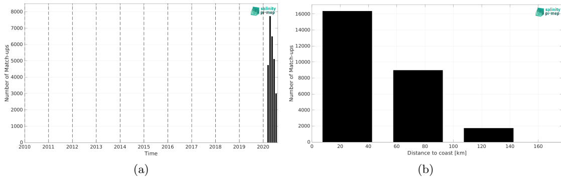
Figure 1: Number of match-ups between Saildrone and SMOS SSS L4 v1 - Weekly (CMEMS-CNR) SSS as a function of time (a) and as function of the distance to coast (b) over the Mediterranean Sea Pi-MEP region and for the full satellite product period.
