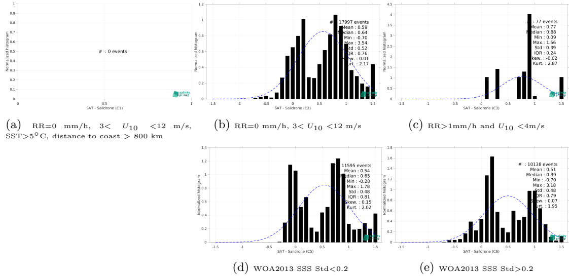
Figure 13: Normalized histogram of \Delta SSS (SMOS SSS L4 v1 - Weekly (CMEMS-CNR) - Saildrone) for 5 different subdatasets corresponding to: RR=0 mm/h, 3 < U_{10} < 12 m/s, SST>5°C, distance to coast > 800 km (a), RR=0 mm/h, 3 < U_{10} < 12 m/s (b), RR>1mm/h and U_{10} < 4 m/s (c), WOA2013 SSS Std<0.2 (d), WOA2013 SSS Std>0.2 (e).
