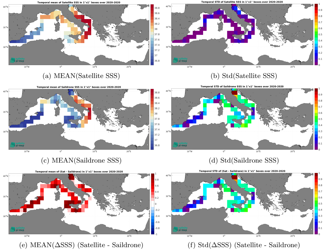
Figure 6: Temporal mean (left) and Std (right) of SSS from SMOS SSS L4 v1 - Weekly (CMEMS-CNR) (top), Saildrone (middle), and of \Delta SSS (Satellite - Saildrone). Only match-up pairs are used to generate these maps.
